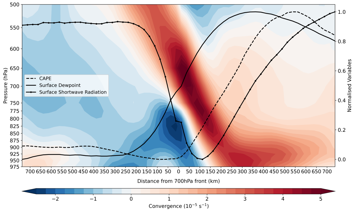
Figure 3. Climatological convergence at pressure levels (shaded), CAPE (dashed line), surface dewpoints (straight line), surface shortwave radiation (straight dotted line) in ERA5 depending on the distance from the 700 hPa front. Excluding convergence, the climatological means are normalised between 0 and 1. The CAPE in ERA5 is calculated based on the most unstable parcel below 350 hPa.
