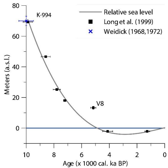
Figure 6: Recalibrated relative sea level curve from Vaskebugt, Arveprinsen Ejland (Long et al., 1999). Sample V8 was excluded from the polynomial fit.
