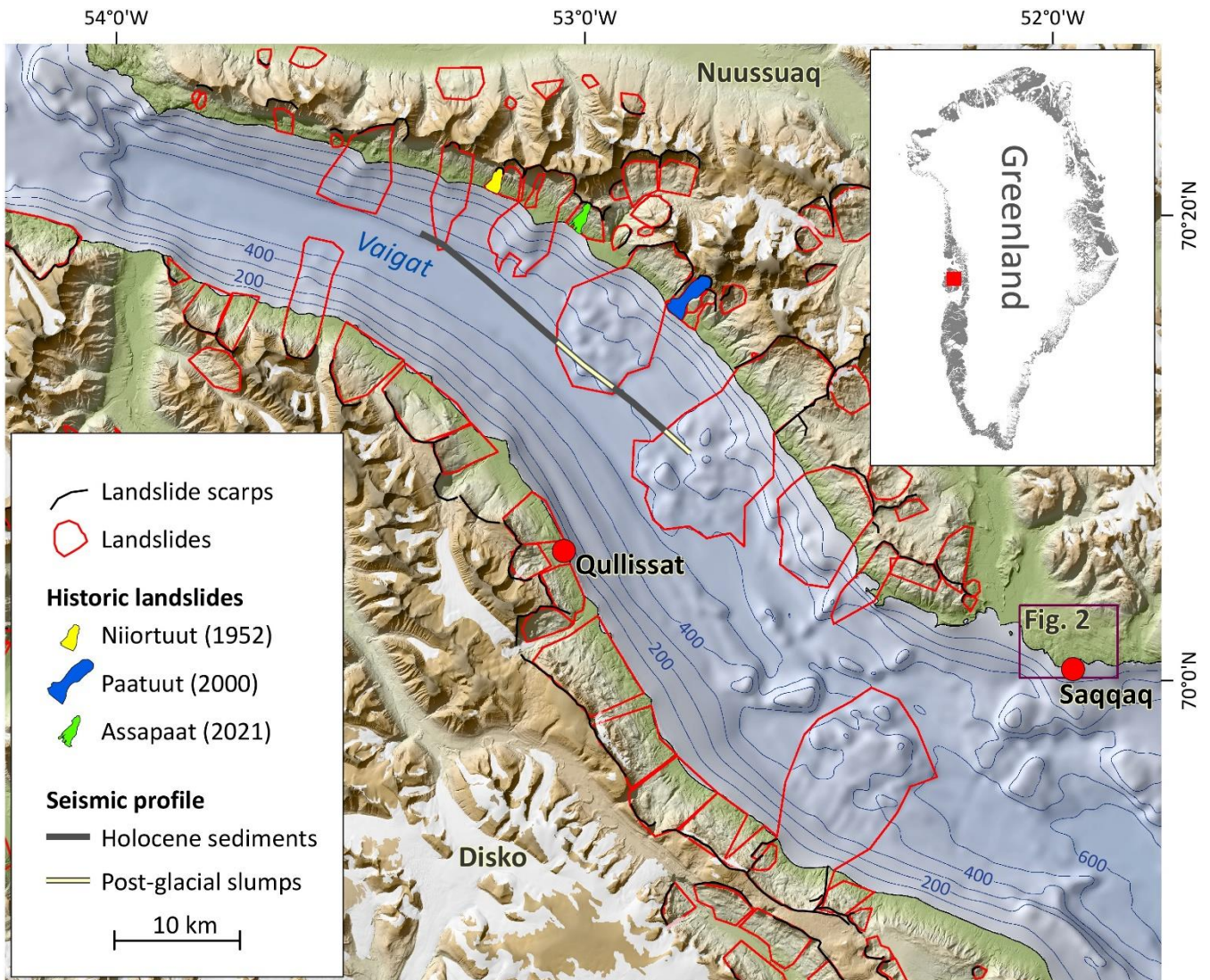
690 Figure 1: Landslide mapping by Svennevig (2019) and Svennevig et al (2023b). Bathymetry from Bedmachine Greenland v4 (Morlighem et al., 2021), other map data from SDFI (2018) and ArcticDEM (Porter et al., 2018). A seismic profile line from Vaigat available from Marcussen et al. (2001) is shown, where the sediments along the profile were interpreted as either post-glacial slumps or glacial moraines, surrounded by horizontal Holocene sediments.
