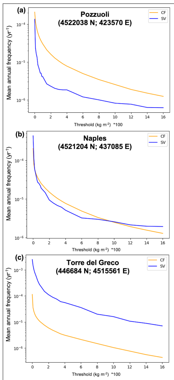
Figure 10. Hazard curves showing the mean annual frequency of exceeding a set of intensity thresholds (tephra load, in \text{kg m}^{-2} ) at three target sites: a) Pozzuoli, b) Municipality of Naples and c) Torre del Greco, due to the impact of Somma-Vesuvius (blue curve) and Campi Flegrei (orange curve), in 50 years.
