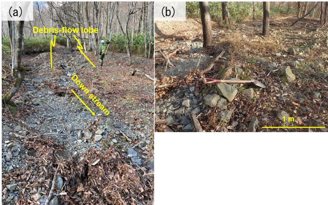
Figure 6: Recent debris flow deposits on a debris flow fan of the Paleogene accretionary complex site: (a) debris-flow lobe, (b) boulders entrained by debris flows.
