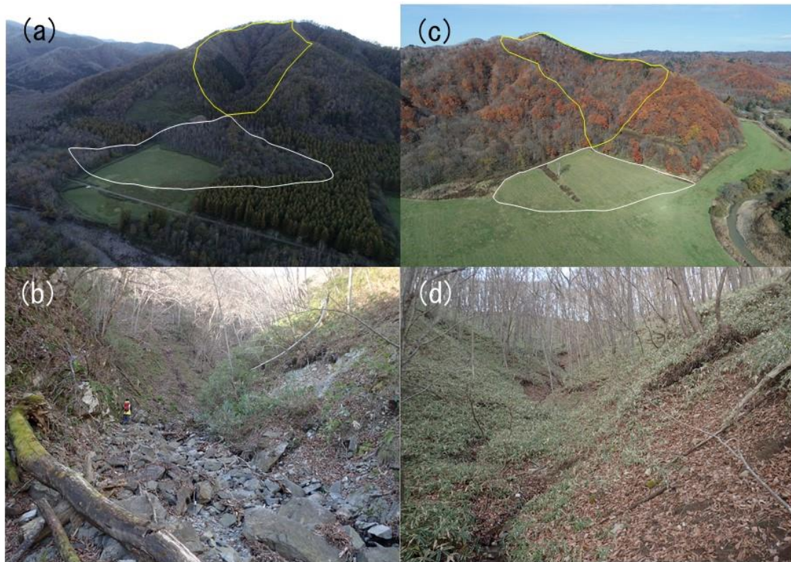
290 Figure 5: Debris flow fans and the channel of the drainage basins in both sites. (a) A debris flow fan in the Paleogene accretionary complex site. White and yellow solid lines are the debris flow fan and drainage basin boundaries, respectively. (b) Channel condition of the drainage basins in the Paleogene accretionary complex site. (c) A debris flow fan in the Neogene sedimentary rock site. White and yellow solid lines are the debris flow fan and drainage basin boundaries, respectively. (d) Channel condition of the drainage basins in the Neogene sedimentary rock site.
