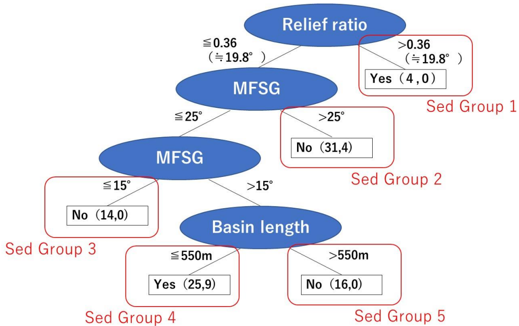
Figure 8: Decision tree for the Neogene sedimentary rock site.
