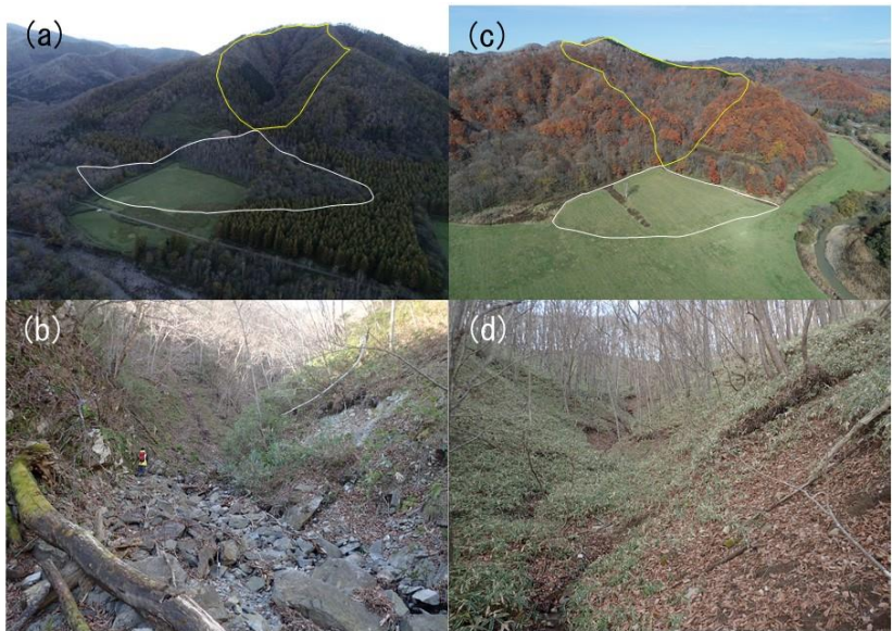
Figure 5: Debris flow fans and the channel of the drainage basins in both sites. (a) A debris flow fan in the Paleogene accretionary complex site. White and yellow solid lines are the debris flow fan and drainage basin boundaries, respectively. (b) Channel condition of the drainage basins in the Paleogene accretionary complex site. (c) A debris flow fan in the Neogene sedimentary rock site. White and yellow solid lines are the debris flow fan and drainage basin boundaries, respectively. (d) Channel condition of the drainage basins in the Neogene sedimentary rock site.
