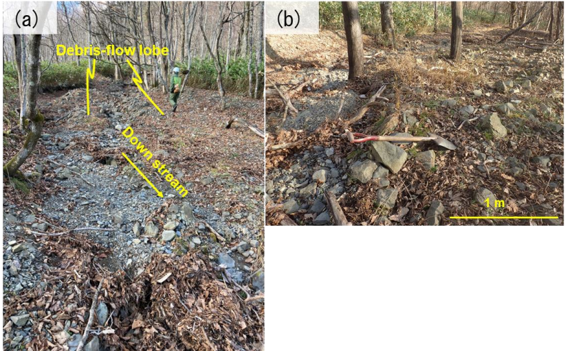
475 | Figure 6: Recent debris flow deposits on a debris flow fan, of the Paleogene accretionary complex site: (a) debris-flow lobe, (b) 480 boulders entrained by debris flows.
