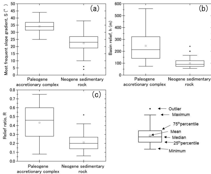
Figure 2: Topographic properties of each drainage basin in the Paleogene accretionary complex site and the Neogene sedimentary rock site: (a) most frequent slope gradient, (b) basin relief, (c) relief ratio.
