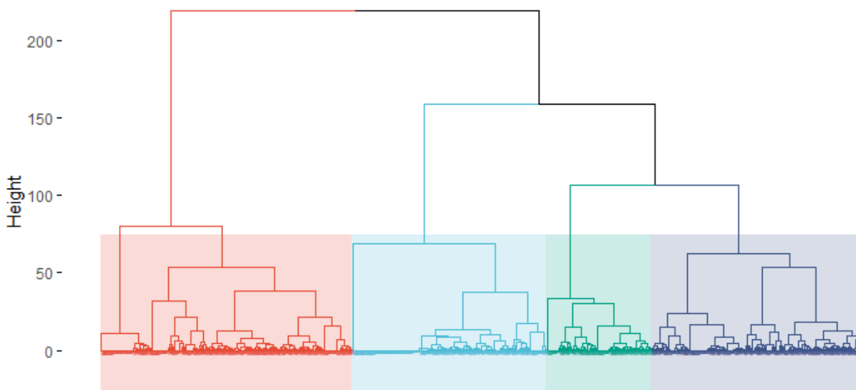
Figure A.5: Dendrogram of hierarchical clustering of DIS with the 4 clusters colored.
