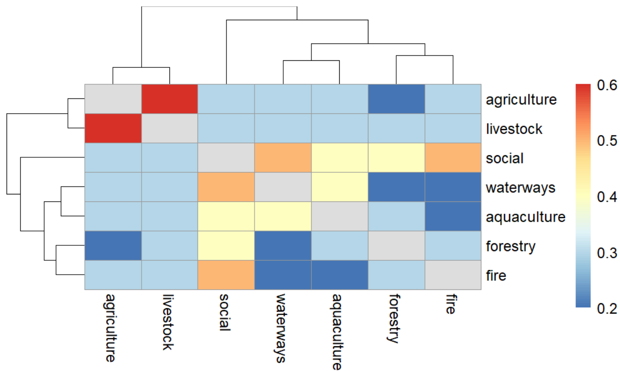
Figure A.4: Correlations between the occurrences of different impact types. Correlation analysis was performed on the obtained drought impact dataset with annual aggregation before transformation for hierarchical clustering. Correlations are calculated using Spearman's Rho.
