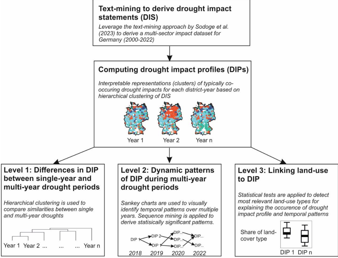
Figure 1: Overview of the methods used to compute drought impact profiles and analyze their patterns.
