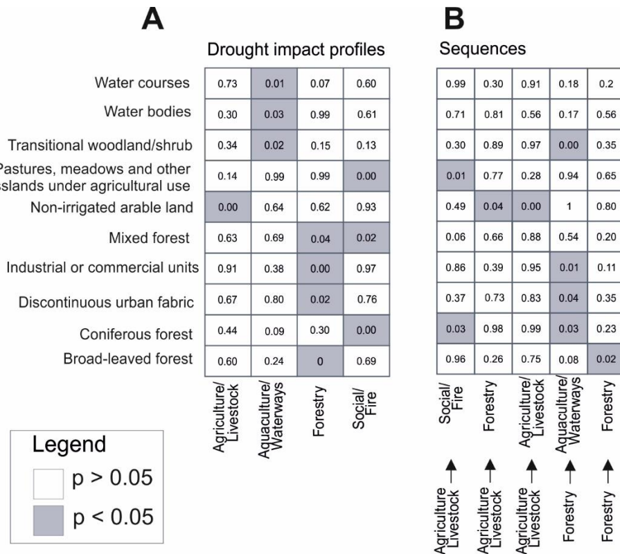
335 Figure 8: Testing associations between land-cover types and (A) DIP occurrences and (B) DIP sequences according to the one-sided Mann-Whitney U test. A significant p-value indicates that districts where a particular DIP (sequence) indicates have a higher share of respective land-cover types.
