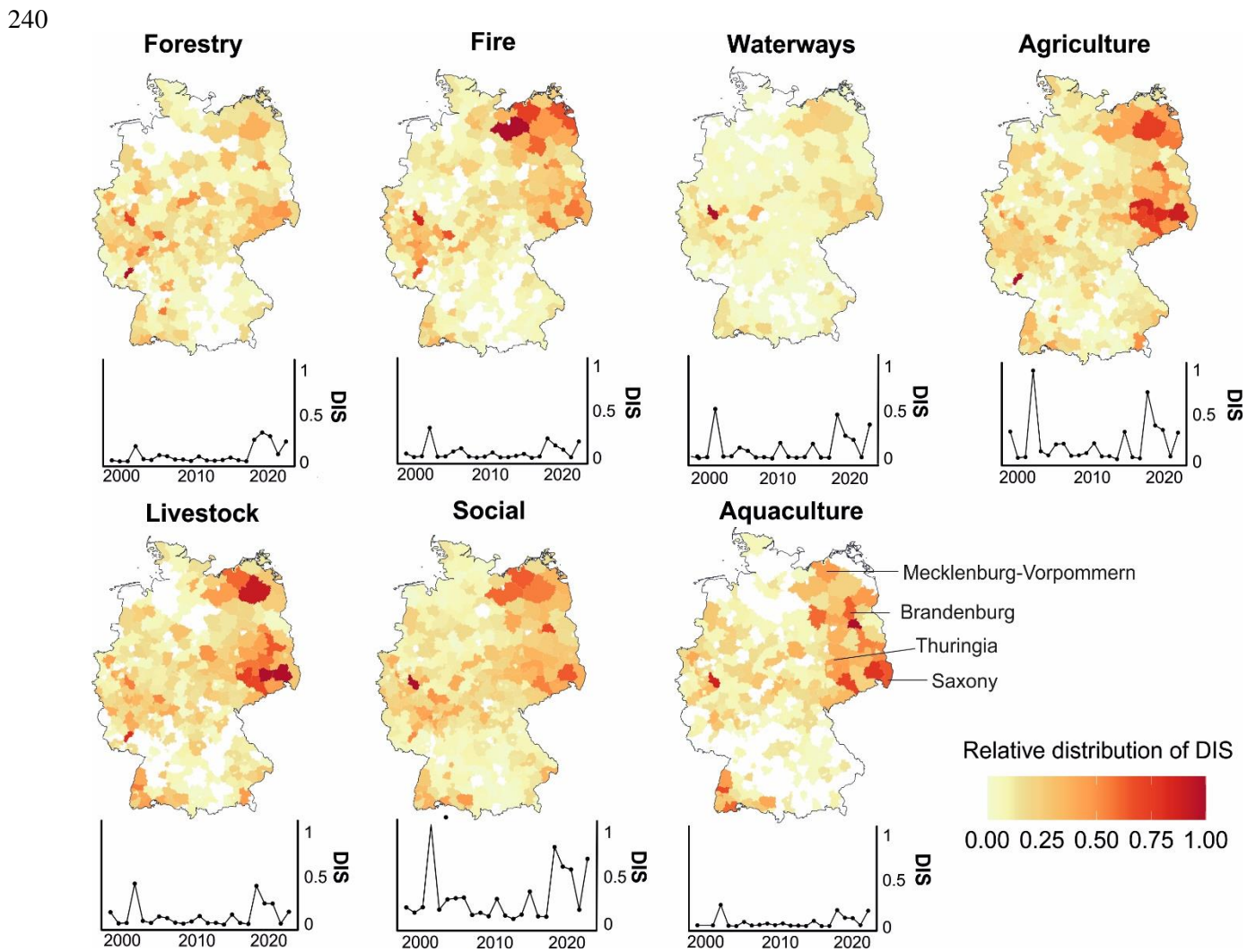
Figure 3: Spatial and temporal distribution of drought impact statements (DIS) between 2000-2022. Each map displays the relative distribution for a particular impact type, where 1 corresponds to the DIS type’s national maximum and 0 to the minimum. Each time series displays the magnitude of DIS, where 1 corresponds to the maximum DIS among all impact types, and 0 is the minimum.
