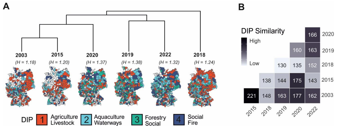
Figure 5: Comparison of annual events based on DIPs within each district. A dendrogram of hierarchical clustering where a structure of similar years emerges. The height dimension within the dendrogram refers to the dissimilarity between the years. H indicates the calculated diversity index. B similarity matrix with the number of identical DIPs between individual years and is used to perform the hierarchical clustering in panel A.
