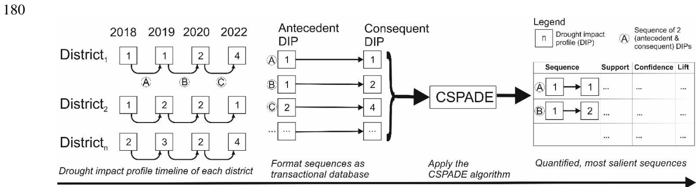
185 Figure 2: Process of extracting DIP sequences with CSPADE algorithm. For each district, a timeline was created representing the DIP observed during the multi-year drought period. These were split into a transactional database representing the transitions between the DIPs of two consecutive years. By using the CSPADE algorithm, we extracted the most frequent sequences and quantified them based on lift, support, and confidence metrics.
