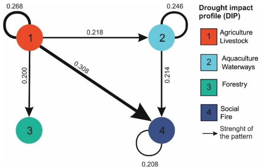
305 Figure 7: Sequences of DIPs during multi-year drought period discovered with CSPADE sequence mining algorithm. All sequences with a minimum support measure of 0.2 are displayed and labeled accordingly. Full evaluation metrics are provided in Table A.3.
