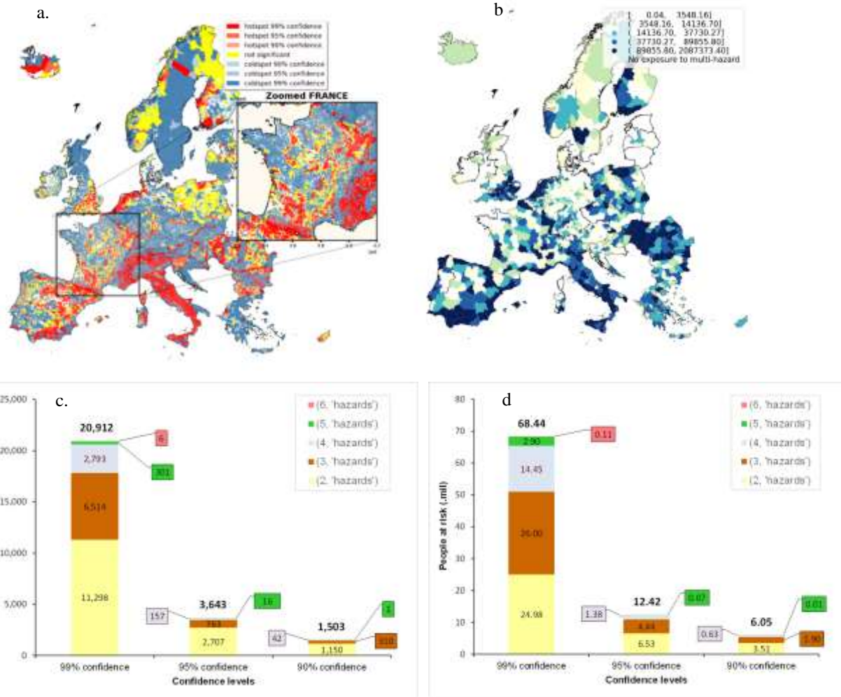
Figure 5. Regions (LAUs) with population at risk exposed to multi-hazards by significance level (a.); Sum of population at risk exposed to multi-hazards assessed at NUTS3 (only hotspots regions with > 90 % confidence interval) (b.); Number of administrative areas at risk exposed to multi-hazards by confidence interval and number of hazards (c.); Population at risk exposed to multi-hazards by confidence interval and number of hazards (d.).
