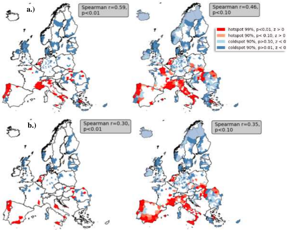
450 Figure 11. Regions (NUTS ) at risk exposed to multi-hazards identified with high significance, p < 0.01 (left), and p < 0.10 (right) as 455 hotspots/cold-spots and their correlation coefficient (Spearman r ) with independent variables: a.) empirical data – fatalities, b.) empirical data – count of events .
