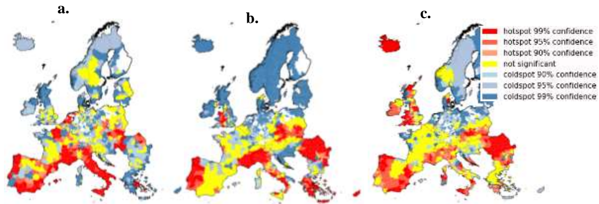
Figure 9. Identified hot /cold -spots regions (NUTS3) with a.) population at riskexposed to multi hazard; b.) fatalities from multi-hazard, c.) number of events with fatalities; -used in Spearman correlation analysis for the validation purpose
