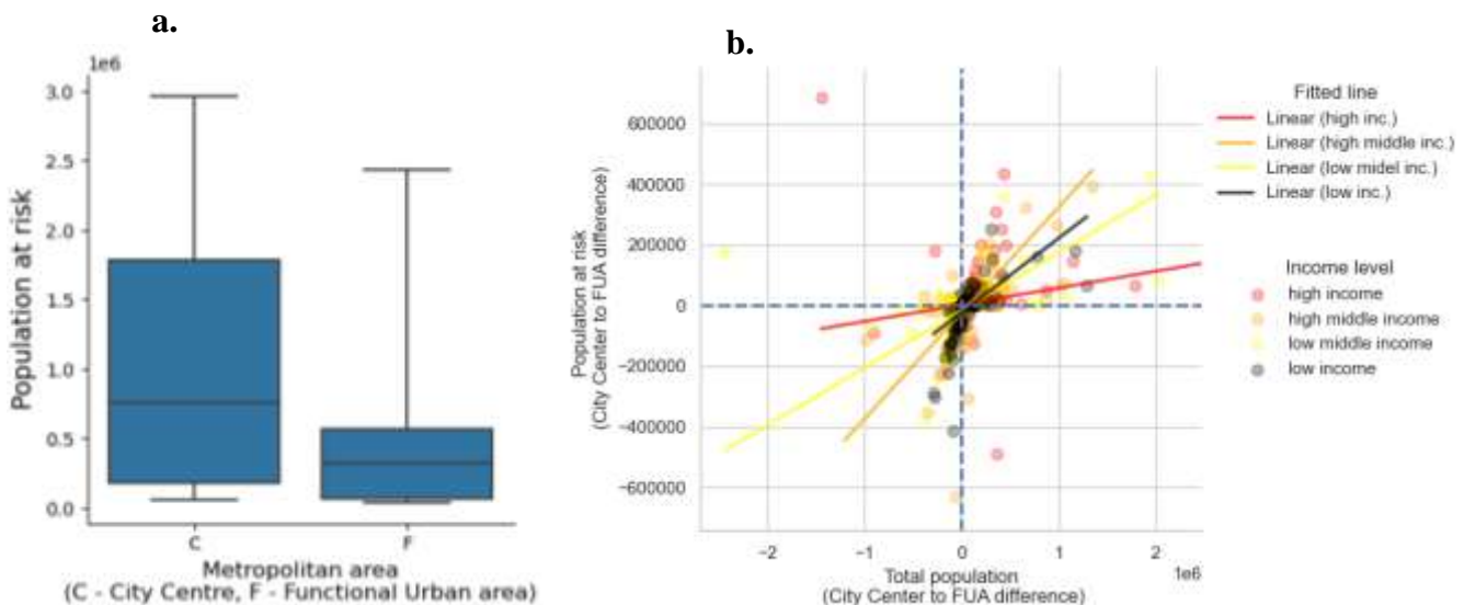
Figure 8. Population at riskexposed to multi-hazards at the level of Metropolitan area; a). European countries' population at riskexposed within Metropolitan categories: City Centres (C) and Functional urban area (F). The lower and upper whiskers represent, respectively, the lowest 5% and the highest 95% of the calculated population at riskexposed to multi-hazards for each metropolitan category; b). Linear relation between population at riskexposed and total population assessed as difference from FUA of the City Centres. A flatter fitted line indicates a weaker or less pronounced relationship between the population at
