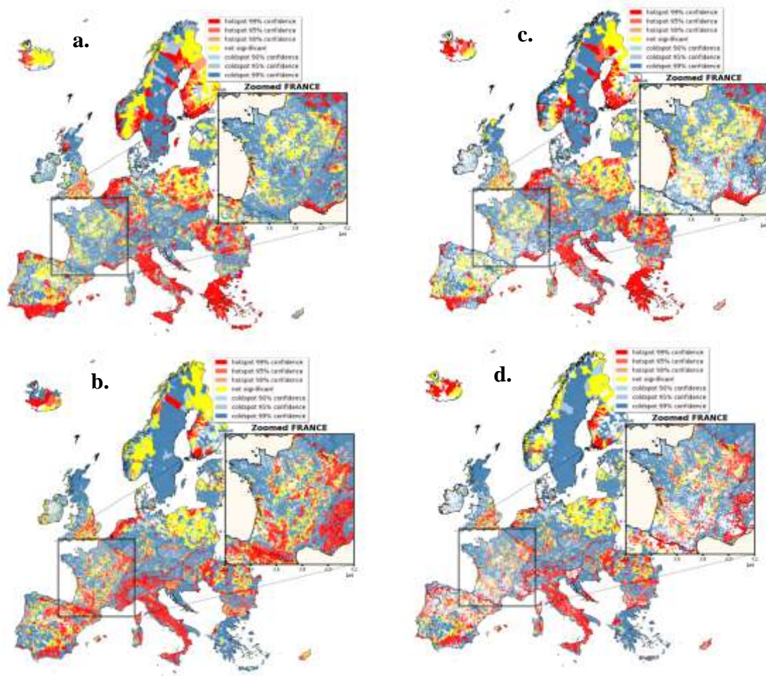
260 Figure 3. Regions (LAUs) at-risk exposed to multi-hazards identified by the meta-data analysis performed on a.) absolute population exposure , b.) relative (%) population exposure, c.) absolute residential built-up exposure and d.) relative (%) residential built-up exposure
