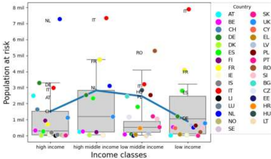
Figure 7. Population at risk/exposed per income level. The markers represent countries' population at risk/exposed of multi-hazard split by income level. The blue line links the 75th quantile of the income classes
