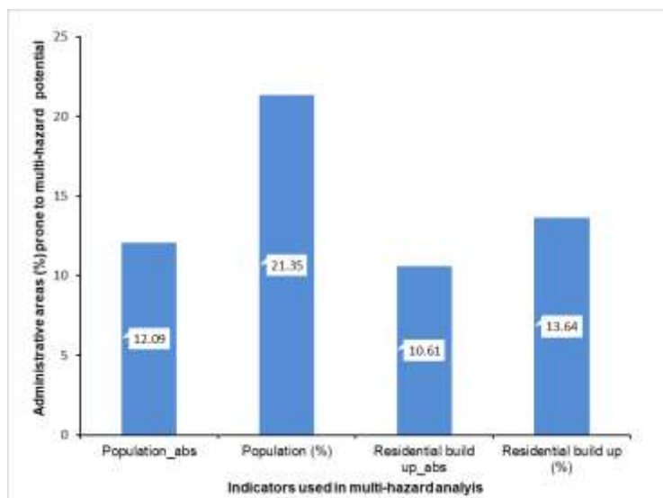
Figure 4. Local administrative units (as % from the total in Europe) identified as being prone to multi-hazards risk -based on different indicators -(population and residential built-up) and aggregation types (relative and absolute)
