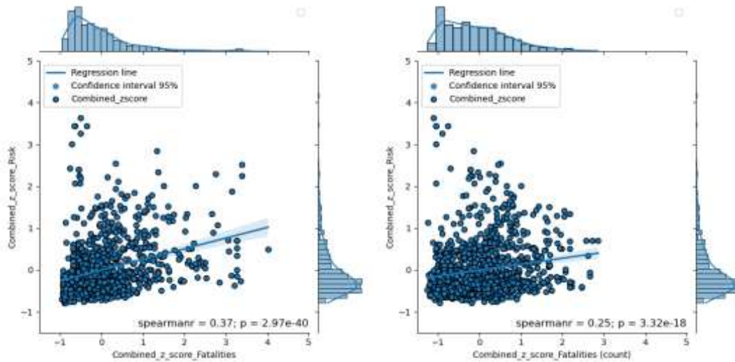
Figure 10 Spearman correlation between the multi-hazard clusters' size (Z-scores) of population at risk exposed with the empirical fatalities from past events (lefts) and events count (right )
