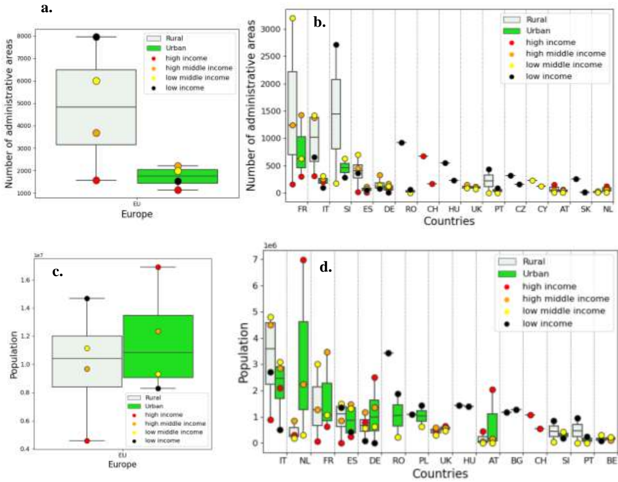
Figure 6. Number of administrative areas (LAUs) with population at risk/exposed to multi-hazards by income level and urbanization level (a. – Europe wide, b. - the 15 highest ranked countries) (upper part); Population at risk/exposed to multi-hazards by income level and urbanization level (c. – Europe wide, d. - the 15 highest ranked countries) (lower part)
