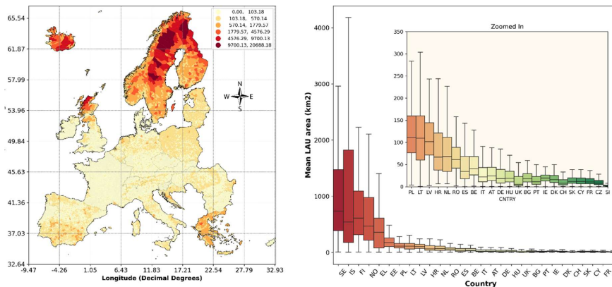
135 Figure 2: Local Administrative Units area (km2), spatial distribution (left) and mean LAUs area per country (right)
