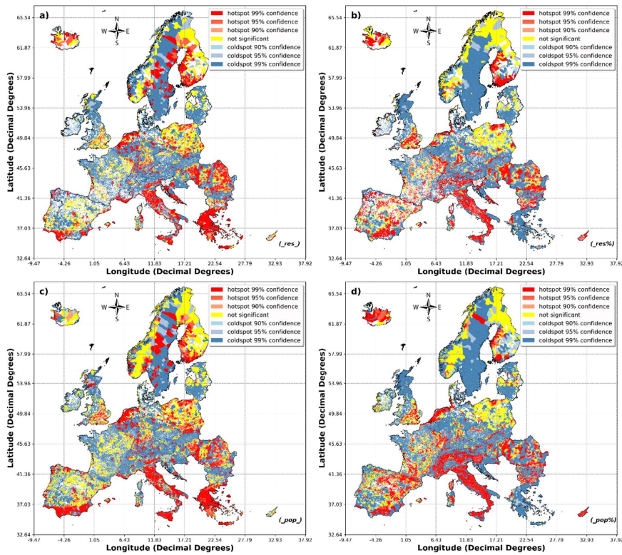
260 Figure 3: Regions (LAUs) exposed to multi-hazards identified by the meta-data analysis performed on a.) absolute residential built-up exposure and b.) relative (%) residential built-up exposure c.) absolute population exposure , d.) relative (%) population exposure.
