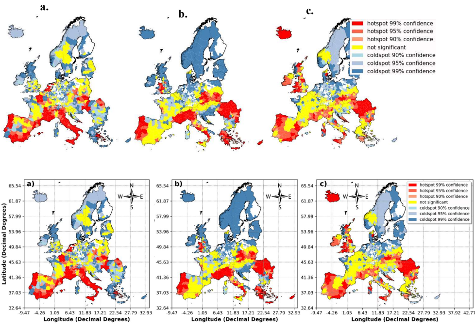
410 Figure 9: Identified hot /cold -spots regions (NUTS3) with a.) population exposed to multi-hazard; b.) fatalities from multi-hazard, c.) number of events with fatalities; used in Spearman correlation analysis for the validation purpose
