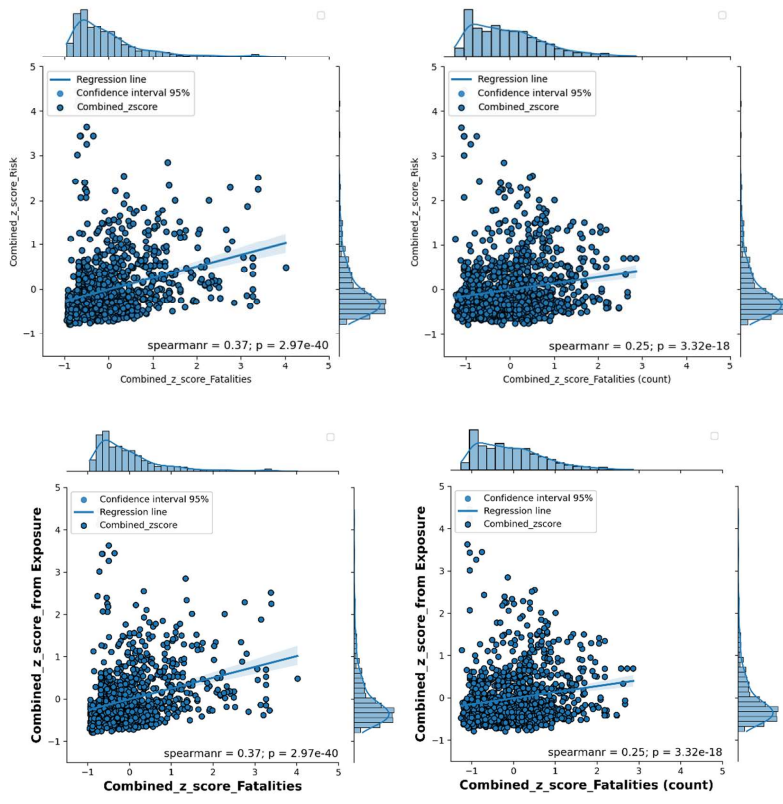
Figure 10: Spearman correlation between the multi-hazard clusters' size (Z-scores) of population exposed with the empirical fatalities from past events (lefts) and events count (right)
