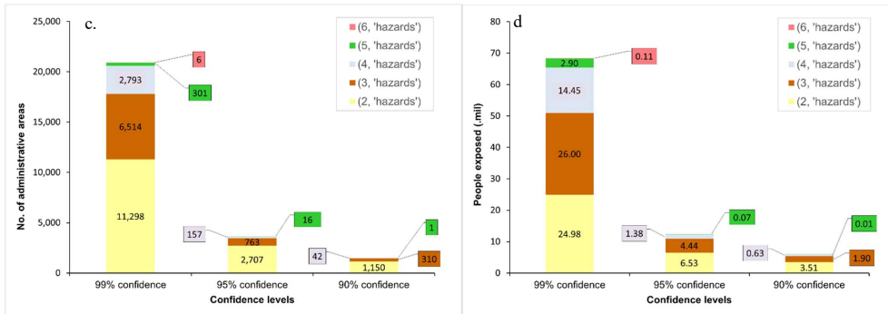
300 Figure 5: Regions (LAUs) with population exposed to multi-hazards by significance level (a.); Sum of population exposed to multi-hazards assessed at NUTS3 (only hotspots regions with > 90 % confidence interval) (b.); Number of administrative areas exposed to multi-hazards by confidence interval and number of hazards (c.); Population exposed to multi-hazards by confidence interval and number of hazards (d).
