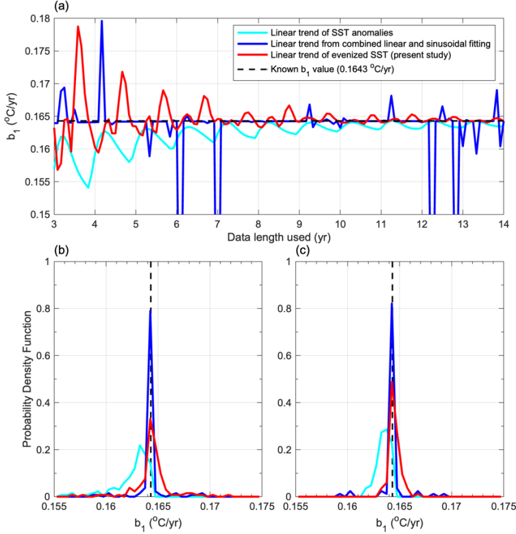
355 Figure 8: (a) \widehat{b}_1 as function of data length using the simulated SST data and probability density function of \widehat{b}_1 using data length of (b) 3-14 years and (c) 7-14 years by applying the methods of SST anomalies (cyan lines), combined linear and sinusoidal fitting (blue lines), and evenized SST (red lines). The black dashed lines denote the known b_1 value.
