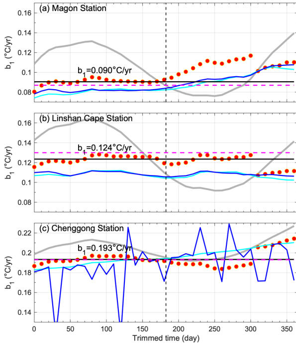
Figure 7: \bar{b}_1 as function of trimmed time using the SST data collected in (a) Magon, (b) Linshan Cape, and (c) Chenggong stations. The OSLR1 method and our proposed method (steps 1-7) are represented respectively by the grey curves and red dots. The black lines depict the averaged \bar{b}_1 values based on corrected data within a trimmed time shorter than T_{tr}/2 , indicated by the vertical dashed line. The cyan and blue curves are the slope estimated using SST anomalies and combined linear and sinusoidal fitting methods, respectively. The magenta dashed lines are the slope derived from linear fitting to the STL nonlinear curve.
