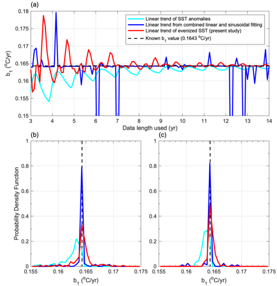
Figure 8: (a) b_1 as function of data length using the simulated SST data and probability density function of b_1 using data length of (b) 3-14 years and (c) 7-14 years by applying the methods of SST anomalies (cyan lines), combined linear and sinusoidal fitting (blue lines), and evenized SST (red lines). The black dashed lines denote the known b_1 value.
