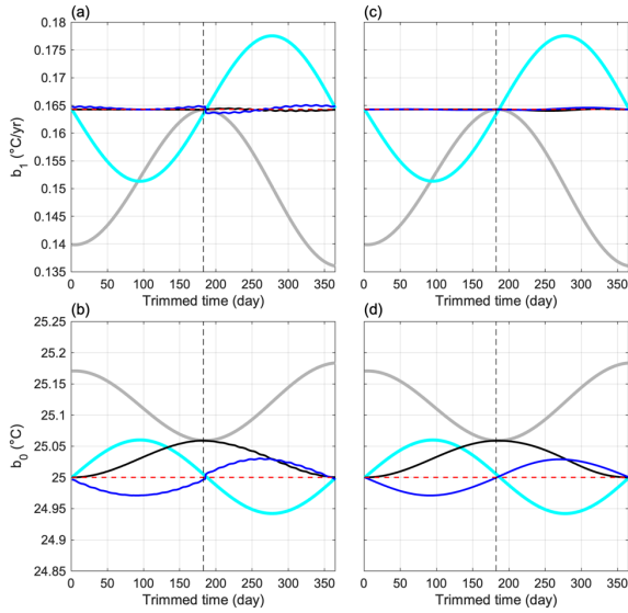
230 Figure 6: Relationship (a) between the trimming time and \hat{b}_1 and (b) between the trimming time and \hat{b}_0 for simulated SST (1) with ST_{SV} represented as a sine function (3) (grey curve) and a cosine (4) (cyan curve). (c) and (d) are the same as (a) and (b), respectively, but removing the tidal signals ST_R . The black and blue curves depict the outcomes after correcting the seasonal bias through steps 1-7.
