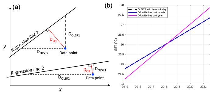
Figure 4: (a) Schematic diagram showing the distances between the data point and the regression line used for OLSR1, OLSR2, and OR. Regression lines 1 and 2 represent steep and gentle slopes, respectively. (b) Regression lines derived from OLSR1 and OR with month and year time units using SST data collected at Chenggong station.
