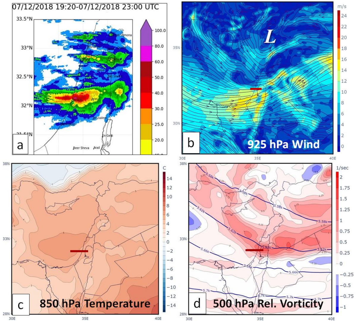
145 Figure 2. Synoptic conditions on 7 December 2018 of (a) Integrated rainfall during 1920-2300 UTC. Atmospheric fields are from 21:00 UTC: (b) Wind field (streamlines and speed, in \text{ms}^{-1} units) at 925 hPa, (c) Temperature ( ^{\circ}\text{C} ) at 850 hPa and (d) Geopotential height (GPH, m) and relative vorticity ( 10^{-5} \text{ s}^{-1} ) at 500 hPa. The maps are derived from ECMWF Integrated Forecast System (IFS) of 0.1^{\circ} resolution. The train is denoted by a red thick line
