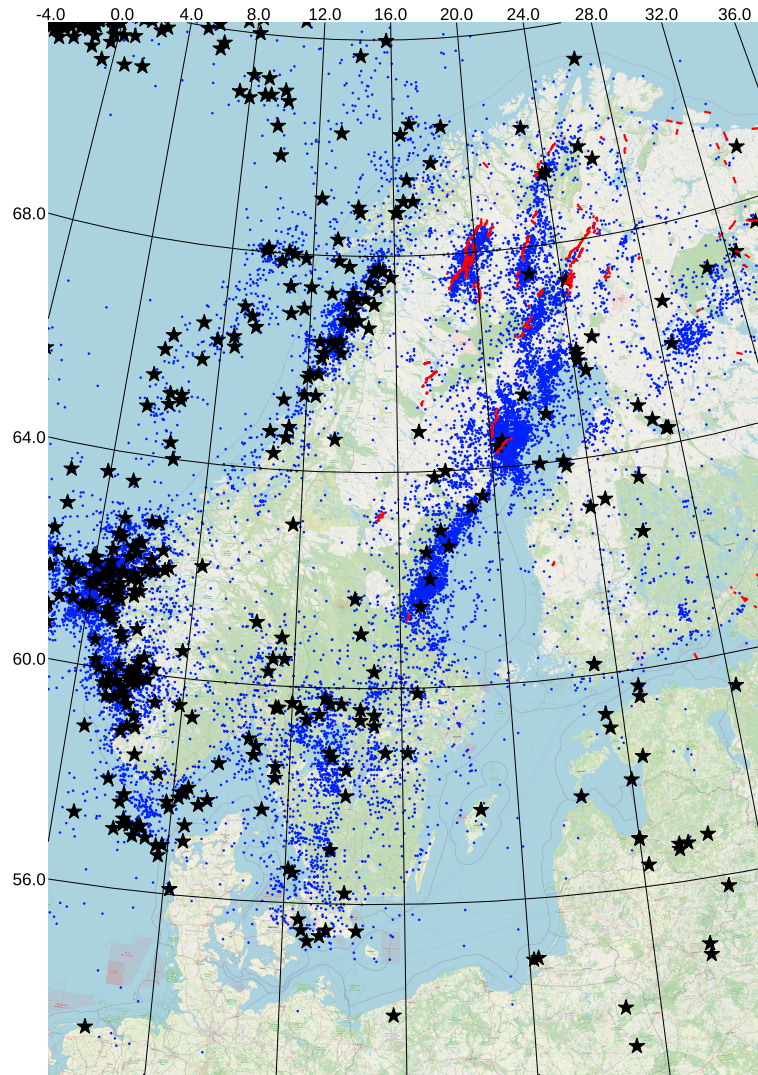
Figure 2. Tectonic source zonation scheme Earthquakes in the Fennoscandian region from our catalogue between 1875 and 2022 (A blue dots) and the area source zonation scheme ESHM20 catalogue 1497 - 2014 where M_w \geq 3.5 (B black stars) used in this study. The red line indicates a zone encompassing Sweden that is 300 km. Red lines: post-glacial faults from the Swedish border or economic zone boundaries Munier et al. (2020). Numbers detail the zone numbers.
