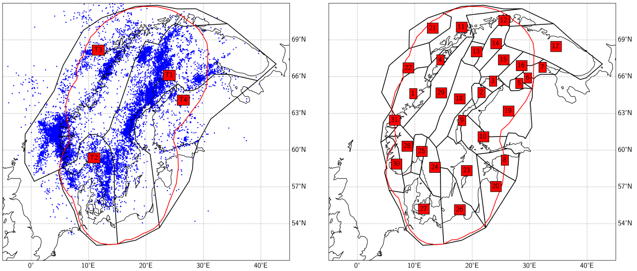
Figure 4. Earthquakes in the ESHM20 catalogue (black stars) and our Tectonic source zonation scheme with the fully declustered earthquake catalogue used in this study (blue dots), north of 63 degrees latitude and between 17 and 32.5 degrees east longitude. Red lines: post-glacial faults (B) Area source zonation scheme. The red line indicates a zone encompassing Sweden that is 300 km from the Swedish border or economic zone boundaries. Numbers detail the zone numbers.
