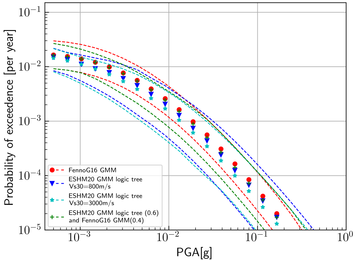
Figure 7. Mean hazard curves for Uppsala, Sweden, for different GMM implementations, see Section 4.6 for details. Yearly probability of exceedance versus PGA in g. Solid lines-symbols show the mean, while the upper and lower dashed lines show the 84% and 16% fractiles.
