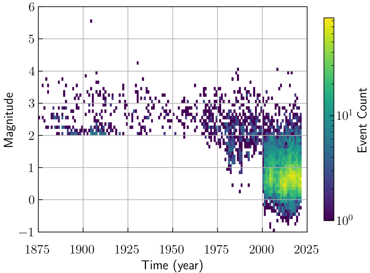
Figure 3. Magnitude-time density plot of the earthquakes since 1875 in the zone encompassing Sweden that is 300 km from the Swedish border or economic zone boundaries (blue dots within the red zone in Figure 4A) from the declustered and magnitude homogenized catalogue.
