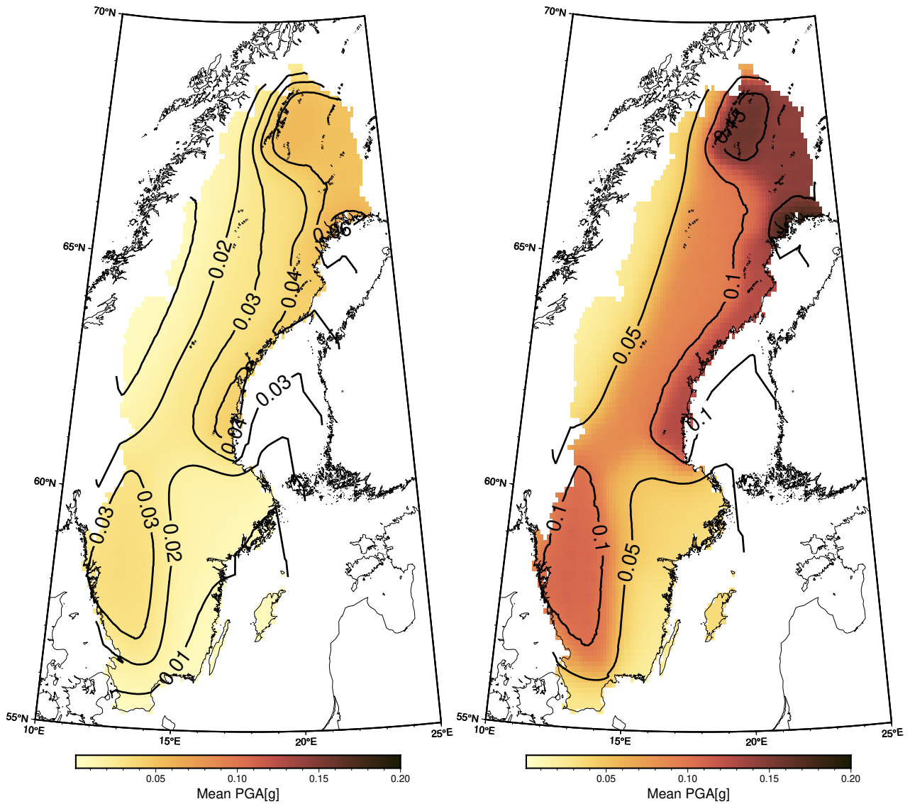
Figure 8. Seismic hazard maps for return periods of 475 years (left) and 2500 years (right). Contour lines represent 0.01g for the 475 year map and 0.025, 0.05g for the 2500 year map. Post-glacial faults indicated by black lines.
