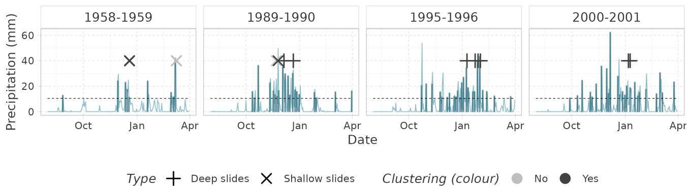
Figure 8. Precipitation time-series (light-blue line) and exceedances (blue bars) above the 80th quantile of wet days (dotted line) for North of Lisbon region, in some selected periods. Points corresponding with the occurrence of landslides are reported with crosses. The colour of the crosses indicates the presence of precipitation clustering prior to the landslide.
