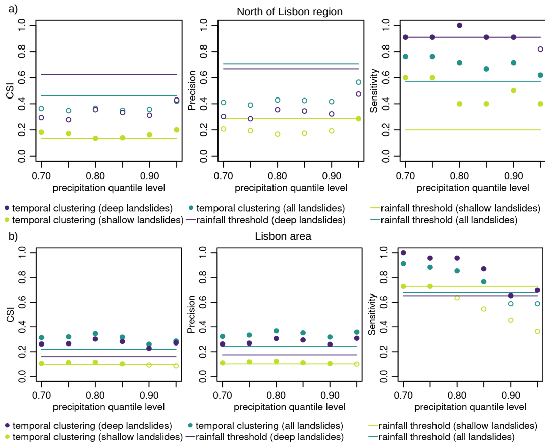
Figure 10. Cluster occurrence approach (dots) compared to the use of solely rainfall thresholds (lines) for a) North of Lisbon region and b) Lisbon area. The considered metrics for performance are: Critical Success Index (CSI); Precision (SR); Sensitivity (POD). Points are filled when the cluster-based approach outperforms the approach based solely on rainfall thresholds. Colors represent the subset of landslides used (see legend).
