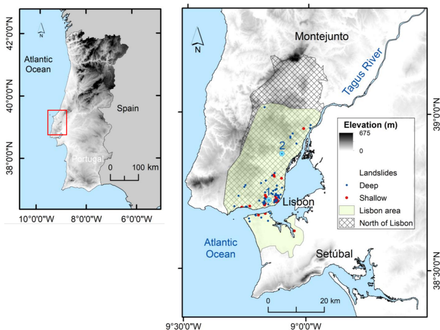
Figure 1. North of Lisbon and Lisbon study areas. Dots represent the landslide cases associated to the different landslide events described in the Disaster Database available at Zêzere et al. (2022). Red dots represent shallow landslide events and blue dots the deep landslide events. Rainfall gauges (blue circles): 1) Lisboa Geofísico; 2) São Julião do Tojal. The landslides associated to the north of Lisbon dataset were not included to improve readability.
