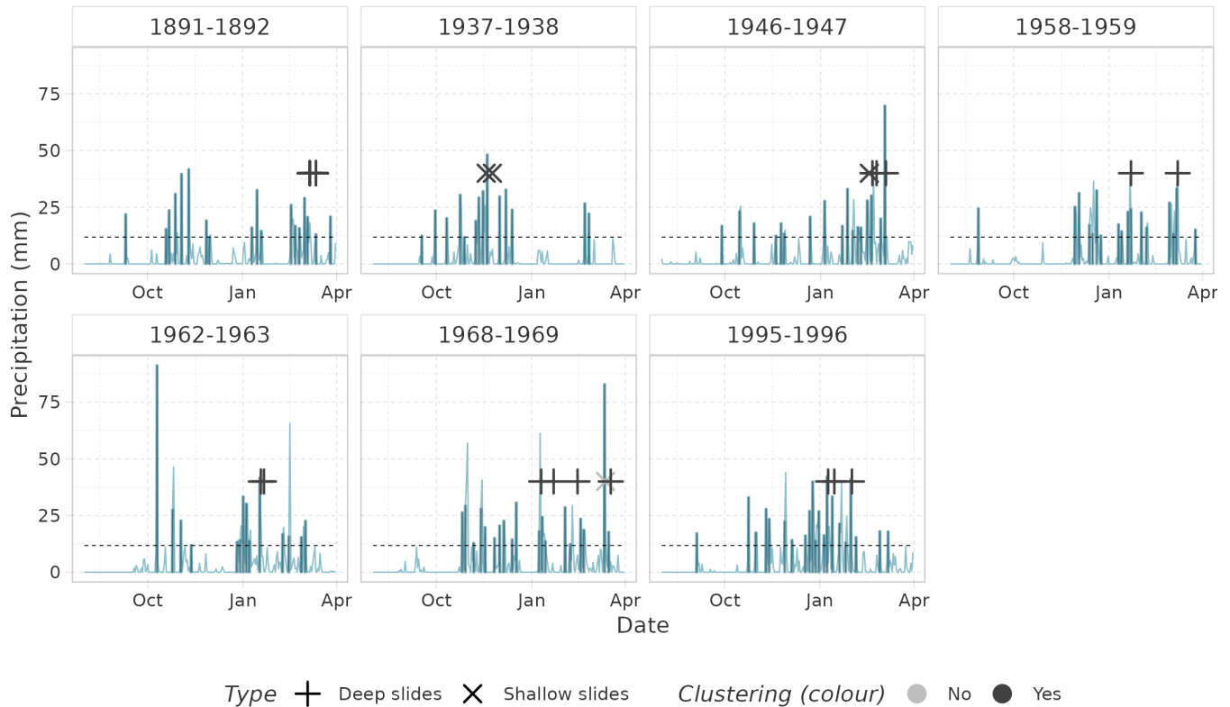
Figure 9. Same as Fig. 8 but for the Lisbon area.
