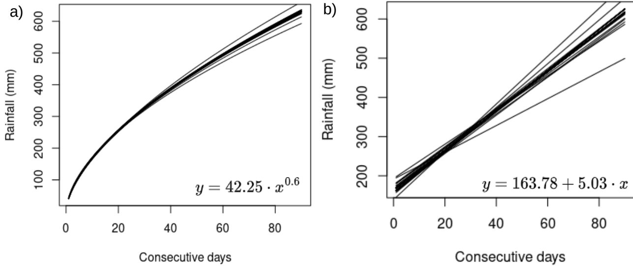
Figure 5. Empirical thresholds obtained from the calibration procedure. Panel a) Lisbon area, Panel b) North of Lisbon region. In the bottom right is reported the equation of the regression curve with the average parameters.
