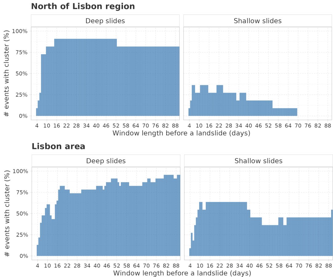
Figure 6. Percentage of windows with temporal clustering of rainfall preceding landslide events, for the two data sets, separated between shallow and deep landslides. Results are reported for u equal to the 80th quantile of daily positive precipitation.
