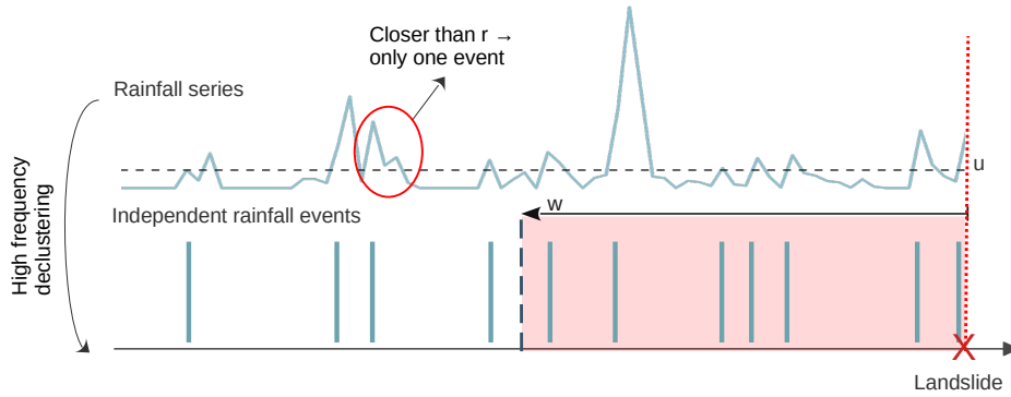
Figure 3. Illustration of the detection method adopted for temporal clustering identification Bevacqua et al. (2021); Banfi and De Michele (2022). The top curve represent the rainfall time series, the peaks on the second line represent the selected heavy rainfall events, after high-frequency declustering. r is the minimum number of days between two peaks. u is the threshold for heavy rainfall. w represents the time window (in days, red shading) before the occurrence of a landslide (red cross). We count n the number of events in the window w
