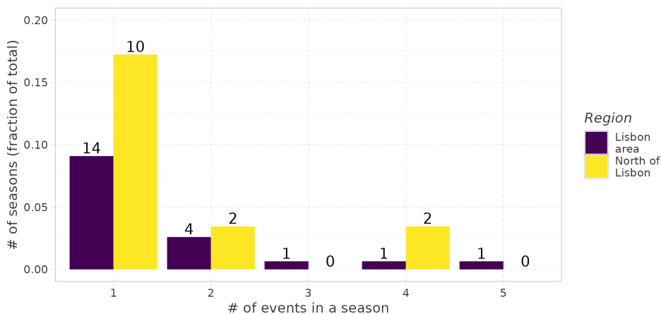
Figure 7. Fraction of season with 1, 2, 3, 4 or 5 landslides (y-axis) and absolute number (label above bars).
