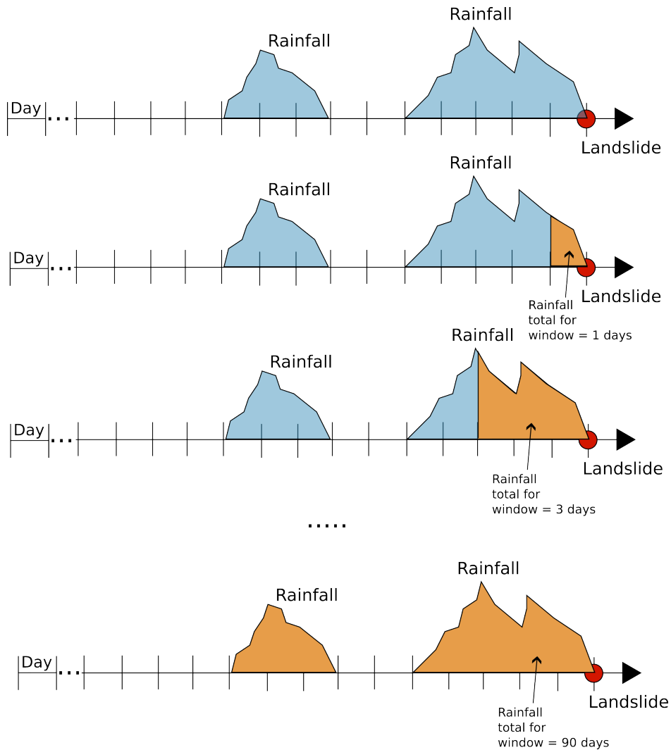
Figure 2. Illustration of step iv (presented in section 2.2) for the computation of rainfall thresholds. The first row represents the time series of precipitation prior to the occurrence of the landslide (shown as a red dot). The following rows show the accumulated precipitation (in orange) over time windows of different lengths prior to the landslide. By expanding the time window, more precipitation before the landslide is considered.
