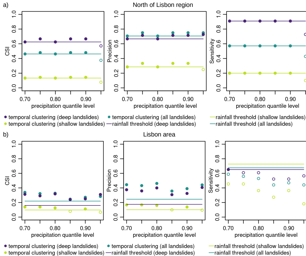
Figure 11. Performance metrics of the methods based on temporal clustering joined with rainfall thresholds and compared to the use of solely rainfall thresholds (lines) for a) North of Lisbon region and b) Lisbon area. The considered metrics for performance are: Critical Success Index (CSI); Precision (SR); Sensitivity (POD). Points are filled when the first method cluster-based approach outperforms the second one approach based solely on rainfall thresholds. Colors represent the subset of landslides used (see legend).
