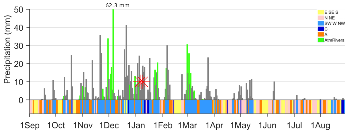
Figure 12. Daily rainfall (light vertical grey bars) along with the correspondent circulation weather type (in colours) for the first months of the 2000/2001 hydrological year. In addition, if the occurrence of the ARs takes place during this hydrological year is highlighted in green in the daily rainfall bars. The red stars indicate the landslides occurrence.
