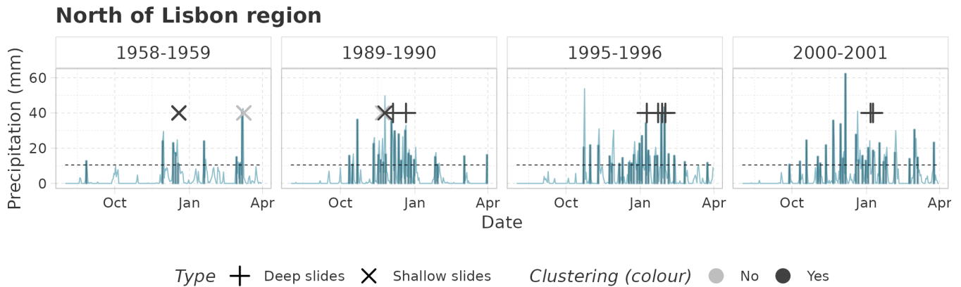
Figure 8. Precipitation time-series (light-blue line) and exceedances (blue bars) above the 80th quantile of wet days (dotted line) for North of Lisbon region, in some selected periods. Points corresponding with the occurrence of landslides are reported with crosses. The colour of the crosses indicates the presence of precipitation clustering prior to the landslide.
