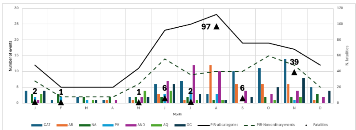
Figure 12: Monthly distribution of the total number of flood cases for the different regions. The solid line shows the entire Pyrenees-POCTEFA region, and the dashed line shows the number of significant events (period 1981-2015). The triangles indicate the total number of casualties in the entire study area, the value is included next to the symbol.
