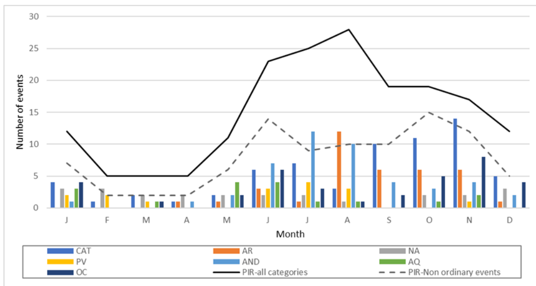
Figure 7: Monthly distribution of the total number of flood cases for the different regions. The solid line shows the entire Pyrenees-POCTEFA region, and the dashed line shows the number of notable events (period 1981-2015).
