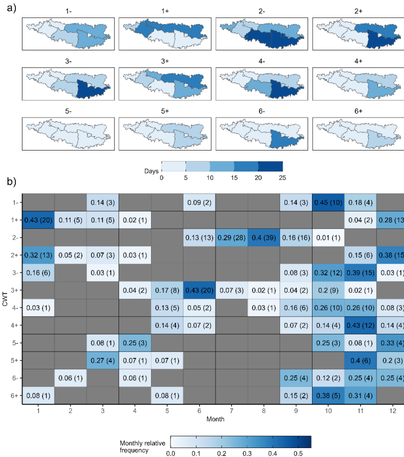
Figure 17. a) Number of flood days by weather type (WT) and Pyrenean region. b) Monthly relative frequencies of flood days by weather type and month. Between parenthesis absolute values are shown in flood days per month.
