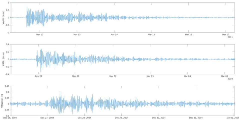
800 Figure 7. Records on Port Vila coastal gauge of 3 transoceanic tsunamis during 6 days after each related earthquake: (bottom) the 26 December 2004 tsunami triggered by the Mw 9.1 Sumatra earthquake in Indonesia; (middle) the 27 February 2010 tsunami triggered by the Mw 8.8 Maule earthquake in Chile; (top) the 11 March 2011 tsunami triggered by the Mw 9.1 Tōhoku earthquake in Japan; the vertical red line symbolizes the earthquake time. The data was detided using a bandpass filter. (Top and middle: 1 min sampling rate data; bottom: 6 min sampling rate data).
