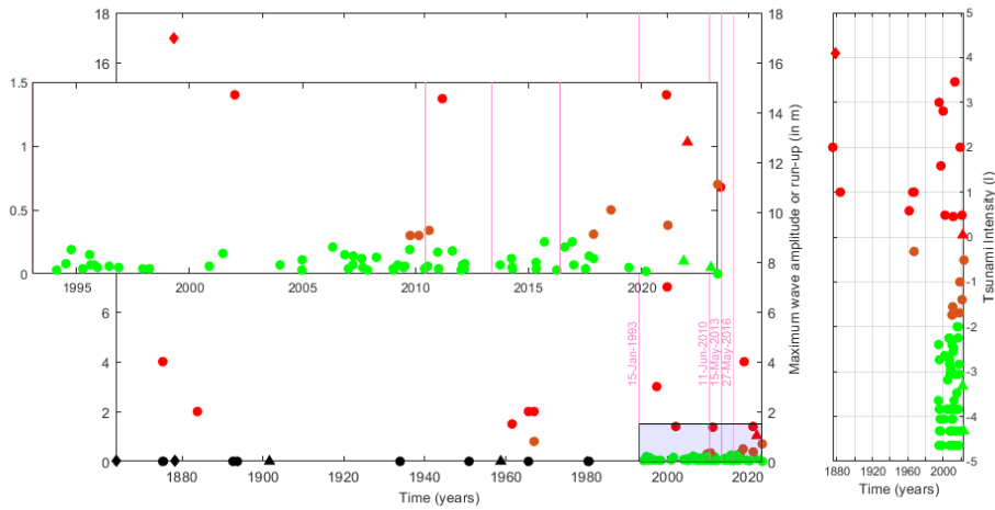
Figure 2. Tsunami maximum recorded amplitude or maximum elevation run-up for each event reported in Vanuatu Arc and listed in Table S1 (left plot). Circles represent tsunamis triggered by earthquakes, triangles represent those triggered by volcanic eruptions, and diamonds represent tsunamis which could have either an earthquake or volcanic origin. The threat level code is provided with green (0-0.3 m), orange (0.3-1 m) and red (1 m and above) colours. The black colour represents the tsunamis reported in Vanuatu Arc without any amplitude or run-up values provided. The vertical pink lines symbolize the beginning of the period of data availability for the five tide gauges located in the Vanuatu Arc. The light blue rectangle (bottom right of the figure) symbolizes the part of the plot zoomed in. The right plot presents the tsunami intensity based on Iida (1963) scale.
