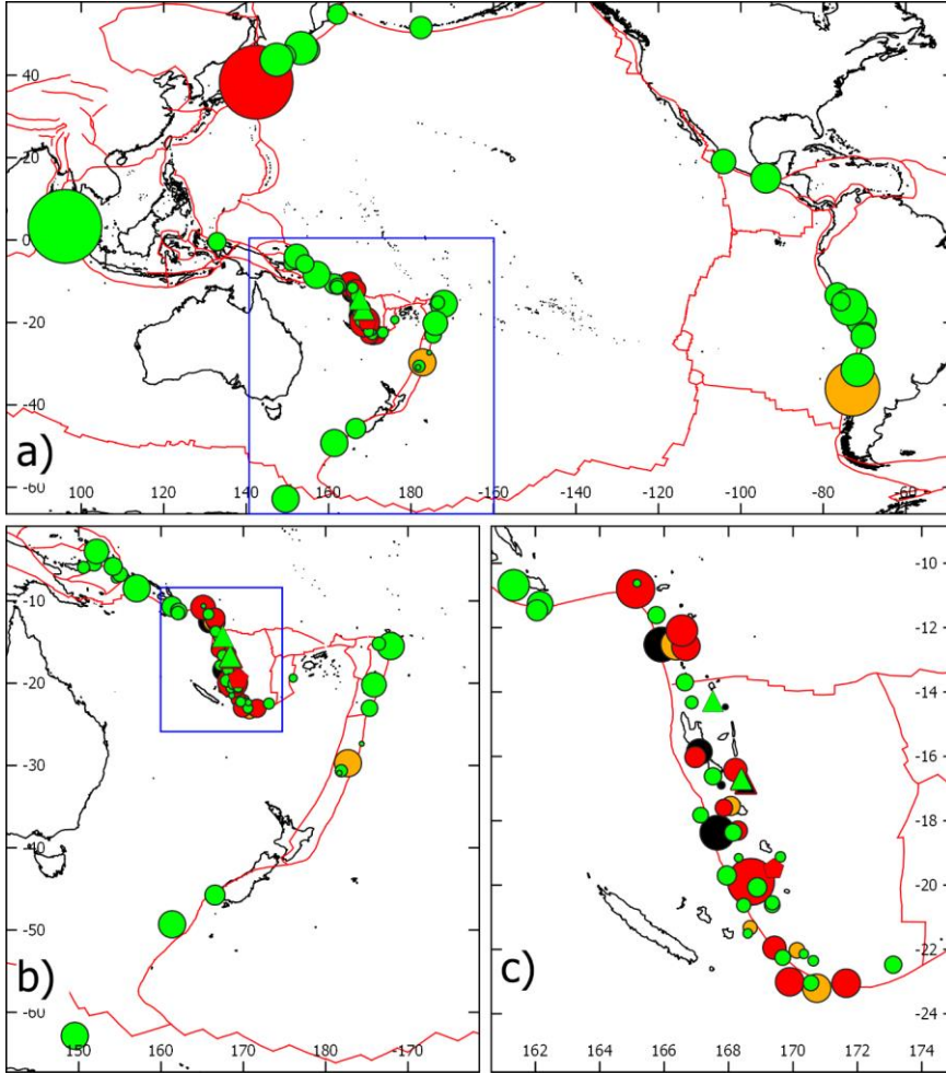
780 | Figure 4 Location of the sources of tsunami reported/recorded in Vanuatu Arc. (a) Oceanic scale ; (b) Southwest Pacific Ocean scale ; (c) Vanuatu Arc scale. The red lines symbolize the plate boundaries; the blue rectangle in (a) represents the extent of (b) and in (b) the extent of (c); earthquake sources are represented with circles (size is function of the magnitude), volcanic eruptions with triangles and both earthquake and volcanic source by a pentagon; Maximum wave amplitude or vertical run-up refers to the threat level ranges: 0-0.3 m: green symbols ; 0.3-1.0 m : orange symbols ; above 1.0 m : red symbols ; no amplitude or run-up information : black symbols. 785
