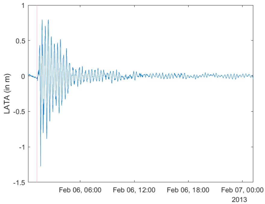
795 | Figure 6 Records on Lata Wharf coastal gauge of the 6 February 2013 tsunami triggered by a Mw 8.0 earthquake west of Ndende Island in the Santa Cruz Islands group (1 min sampling rate data). The vertical red line symbolizes the earthquake time.
