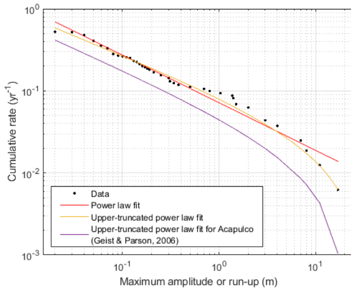
815 Figure 9. Tsunami exceedance frequency curve showing the cumulative rate of tsunamis (yr -1 ) exceeding the maximum amplitude or run-up value given by the abscissa for the present tsunami catalogue of the Vanuatu Arc over the period 1863-2023. The black dots represents the data; the red line represents the trend with a power law fit ( a=0.0716 ; b=-0.581 ); the yellow line represents the trend using an upper-truncated power law fit based on the work from Burroughs and Tebbens (2001) with C=0.0993 and D=-0.4626 ; the purple line is an example of the trend using an upper-truncated power law fit for tsunami exceedance frequency for Acapulco (Geist and Parsons, 2006).
