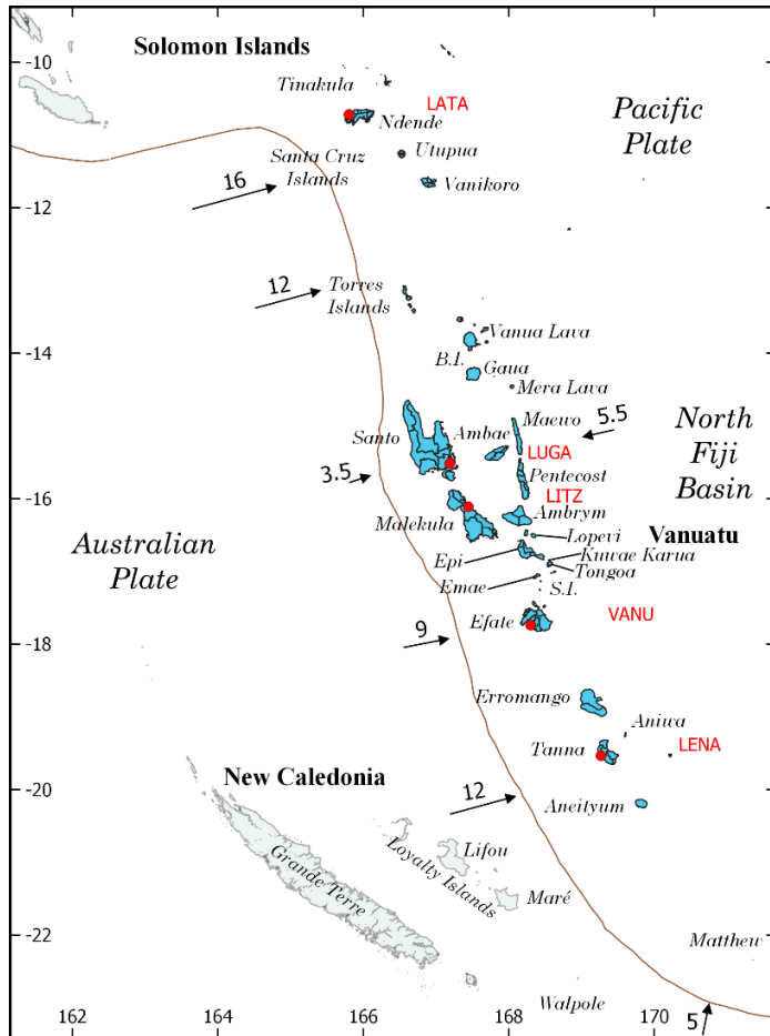
Figure 1 The Vanuatu Arc at the boundary between the Australian and the Pacific tectonic plates. The convergence rates are symbolized with the black arrows (values from Calmant et al., 2003, are indicated in cm/year). The five coastal tide gauges are symbolized with red circles.
