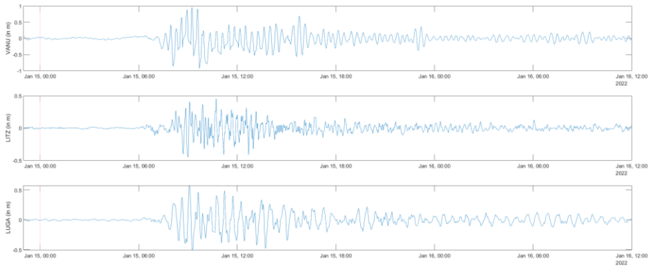
805 Figure 8. Records of the HTHH tsunami on three of the five coastal gauges of the Vanuatu Arc. From South (top) to North (bottom): VANU, LITZ & LUGA. The red vertical line indicates the time of the main volcanic eruption.
