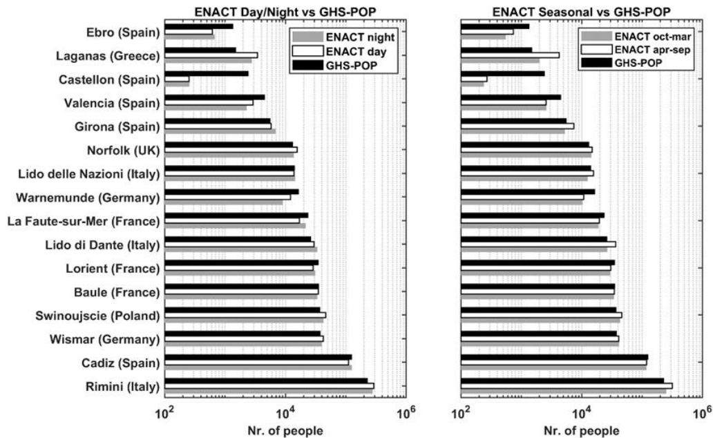
510 Figure 10: Overview of the population on the AoIs of the sites' test cases: the GHS-POP estimate is compared with the ENACT estimate for the day-time and night-time (left box) and with the ENACT estimate for summer (April-September) and winter (October-March) seasons (right box). The number of people is represented using a logarithmic scale.
