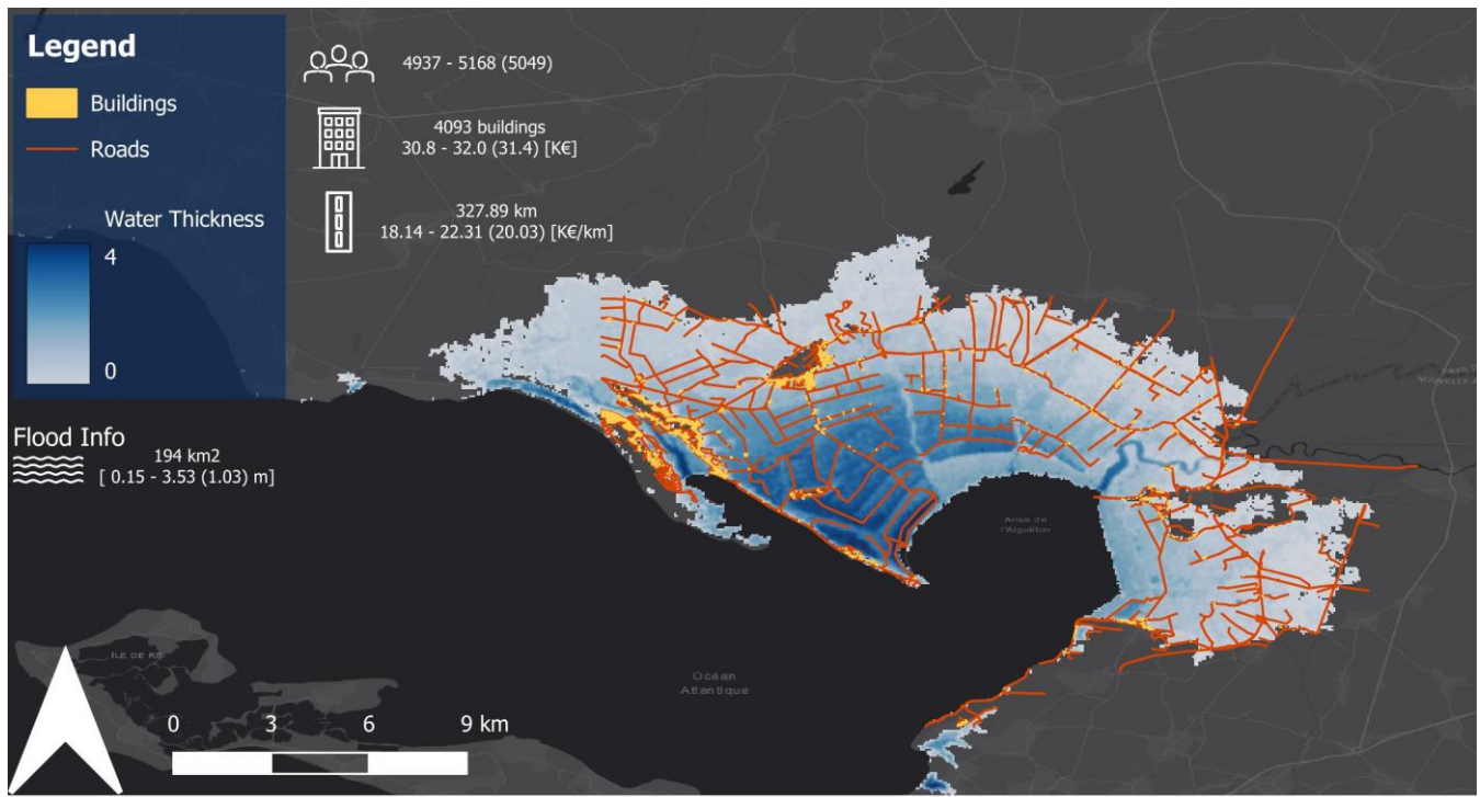
Figure E. 1. Modelled impact map for Xynthia (La Faute-sur-Mer, France) – 2010. The map contains information on the modelled flood extent, the estimation of affected people, the damage assessment for buildings (number of flooded buildings and mean damage) and the damage assessment for roads (affected road length and mean damage).
