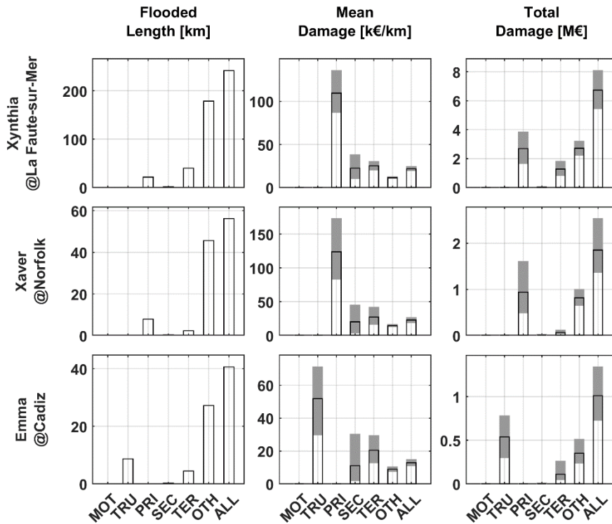
350 Figure 7: Overview of impacts to roads for Xynthia at La Faute-sur-Mer (France, 2010; first row), Xaver at Norfolk (UK, 2013; second row) and, Emma storm at Cadiz (Spain, 2018; third row): length of flooded roads in km (deterministic estimate; first column), mean damage per km in thousands of € (probabilistic estimate; second column) and, total damage (in the AoI) in millions of € (probabilistic estimate; third column). The results are shown for motorways (MOT), trunks (TRU), primary (PRI), secondary (SEC), tertiary (TER), others (OTH) and all (ALL) roads. Damages are based on average 2020 price levels for EU-28, European Union with 28 Member States (Eurostat, 2019).
