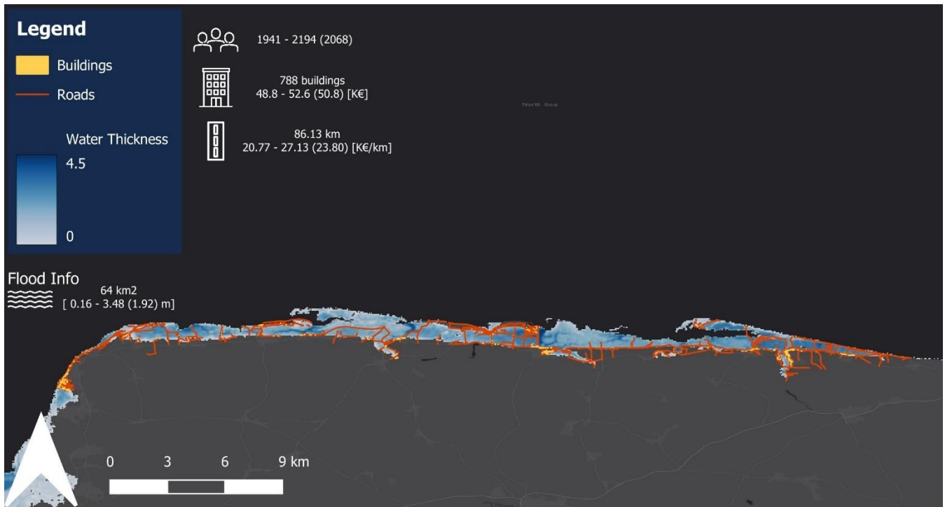
Figure E. 2. Modelled impact map for Xaver (Norfolk, UK) – 2013. The map contains information on the modelled flood extent, the estimation of affected people, the damage assessment for buildings (number of flooded buildings and mean damage) and the damage assessment for roads (affected road length and mean damage).
