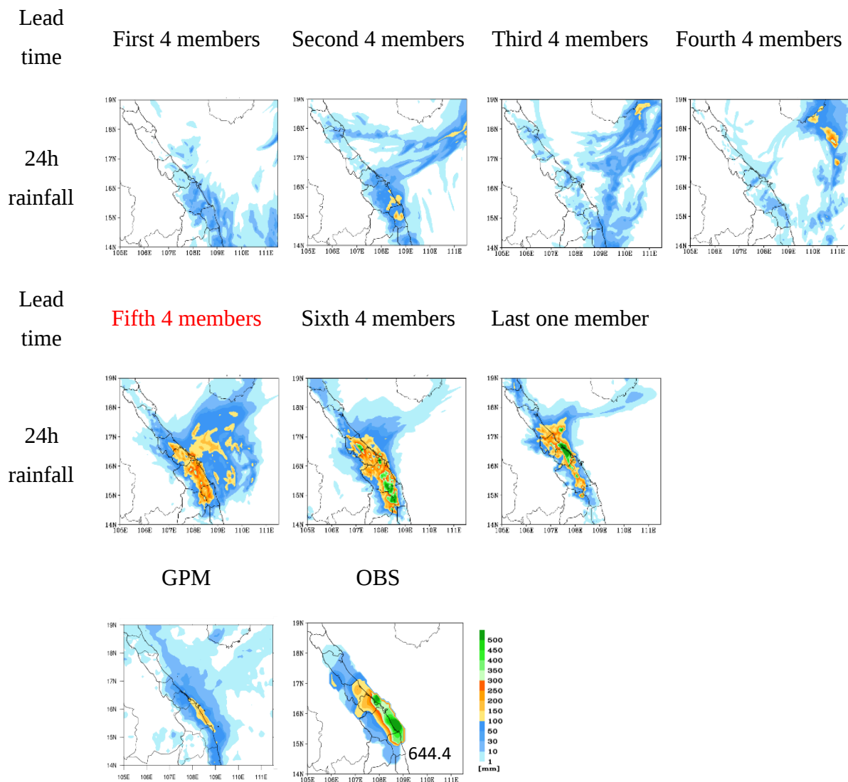
392 Figure 4. The predicted 24h rainfall by subgroup members, 24h accumulated rainfall by 393 the Global Precipitation Measurement (GPM) estimate (IMERG Final Run product), 24h 394 observed rainfall (mm, peak amount labeled at the lower-right corner) for the period of 395 12:00 UTC 9 December – 12:00 UTC 10 December 2018 as labelled. The same color bar 396 (lower right) is used for all panels.
