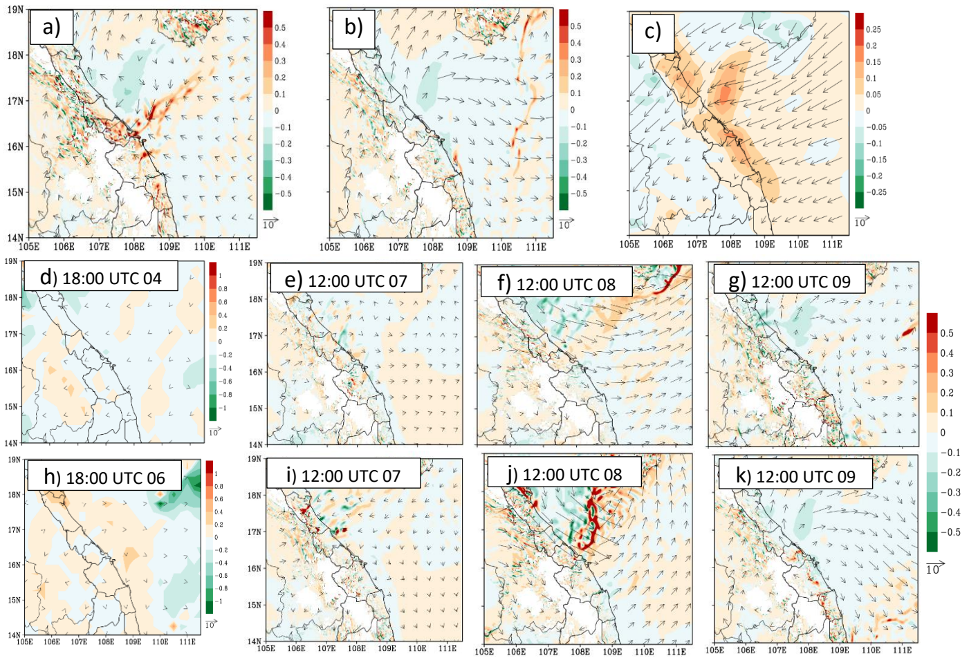
524 Figure 10. The difference in the horizontal wind ( \text{ms}^{-1} , vector, reference length at the low- 525 right corner of the panel), and vertical velocity ( \text{ms}^{-1} , shaded, the reference color scale is 526 on the right of panel) between (a) averaged 5 good members and (b) averaged 5 bad 527 members and the NCEP FNL analysis data at 925 hPa and at 12 UTC 09. (c) The NCEP 528 FNL analysis horizontal wind ( \text{ms}^{-1} , vector, reference length at the low-right corner of the 529 panel) and vertical velocity ( \text{ms}^{-1} , shaded) at 925 mb and at 12 UTC 09. (d) The difference 530 in the horizontal wind ( \text{ms}^{-1} , vector, reference length at the low-right corner of the panel), 531 and relative humidity (% , shaded, the reference color scale is on the right of panel) between 532 the initial data of a good member at a longer lead time (at 1800 UTC 4 Dec) and the NCEP 533 FNL analysis data at 925 hPa. (e), (f), and (g) present the difference in the evolution of 534 weather features with time by this good member. (h) as in (d) but for a bad member 535 (member ran at 1800 UTC 6 Dec). (i), (j) and (k) as in (e), (f), and (g), respectively, but for
