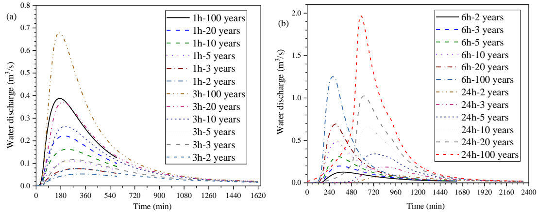
Fig. 13 Predicted hydrographs for different design rainfall events: (a) 1h and 3h events; (b) 6h and 24h events. In the legends, for example, “1h-100 years” means the rainfall event of 100 years return period and 1h duration.
