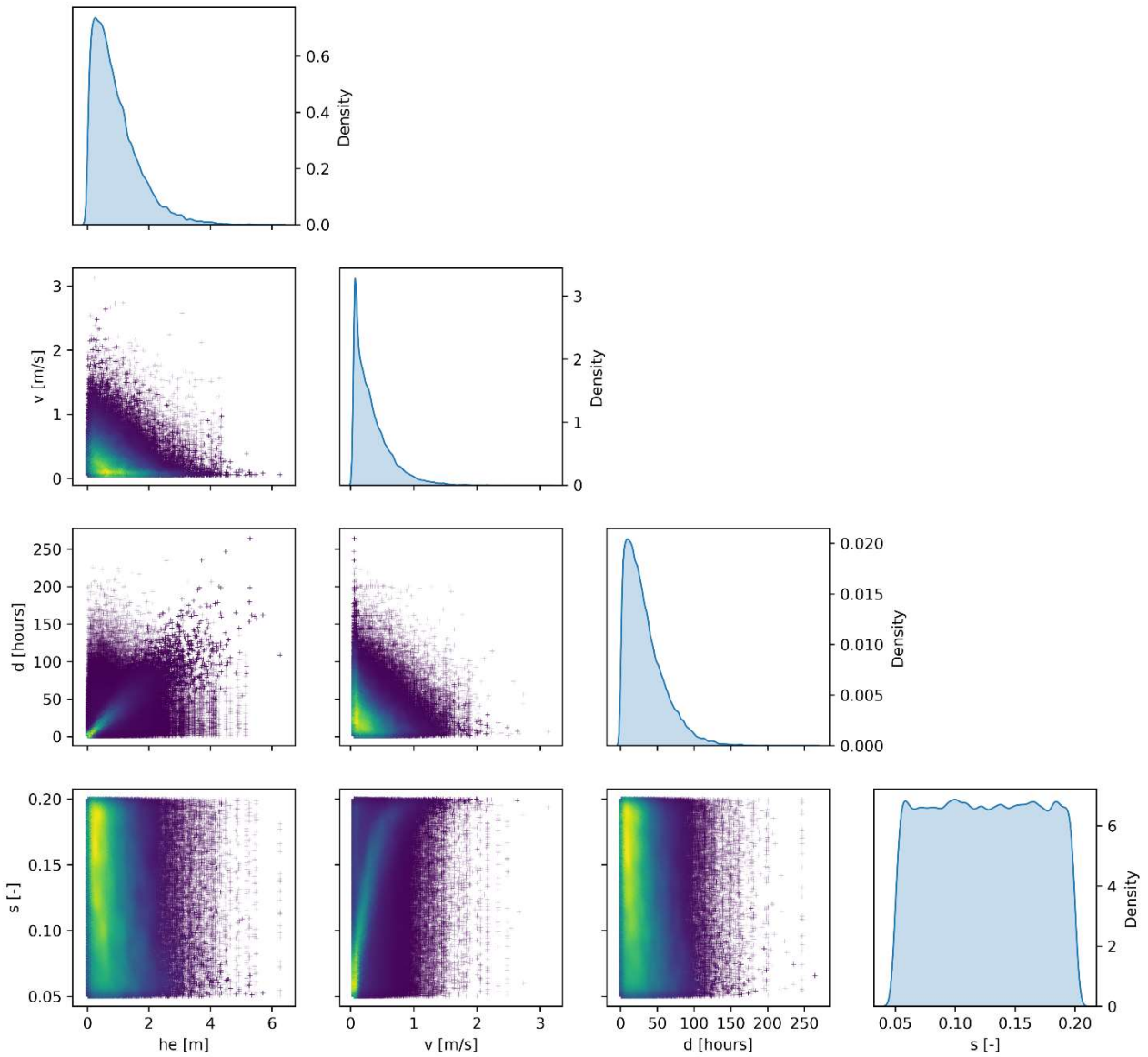
295 Figure 2. Empirical pairwise relationships assumed for the generation of the distributions representative of northern Italy Po River District synthetic dataset: hazard parameters-variables (water depth (he), flow velocity (v), inundation duration (d) and sediment load (s)).
