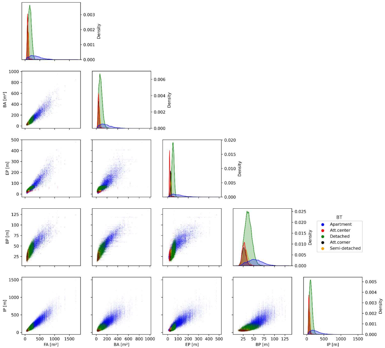
Figure 3. Empirical pairwise relationships assumed for the generation of the Po River District synthetic dataset of the distributions representative of northern Italy: extensive building parameters-variables (footprint (FA) and basement (BA) area; external (EP), internal (IP) and basement perimeter (BP)).
