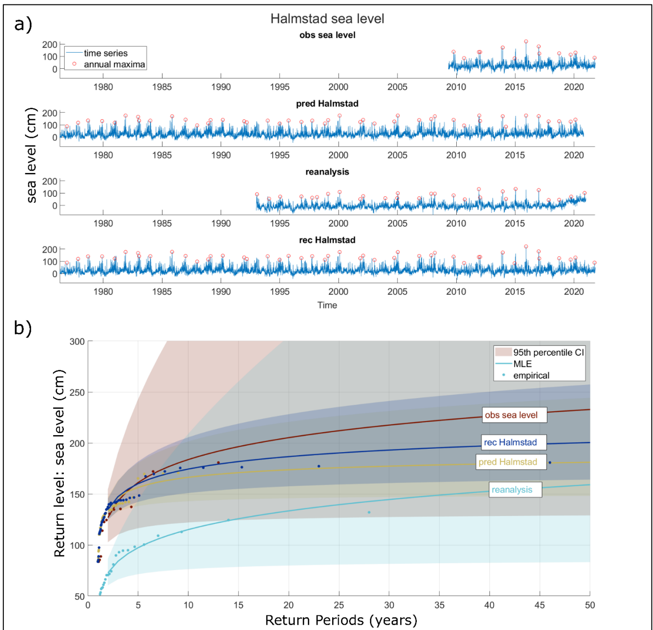
130 Figure 3: Halmstad sea level time series and annual maxima from different sources: observations ("obs sea level"), reconstructed ("rec Halmstad") and predicted ("pred Halmstad") derived from a machine learning model trained on data from the Viken station, and reanalysis ("reanalysis") datasets (panel a). RIs estimated from corresponding GEV fits of each dataset and the associated 95 th percentile confidence intervals (background colours). The dots depict empirical data (panel b).
