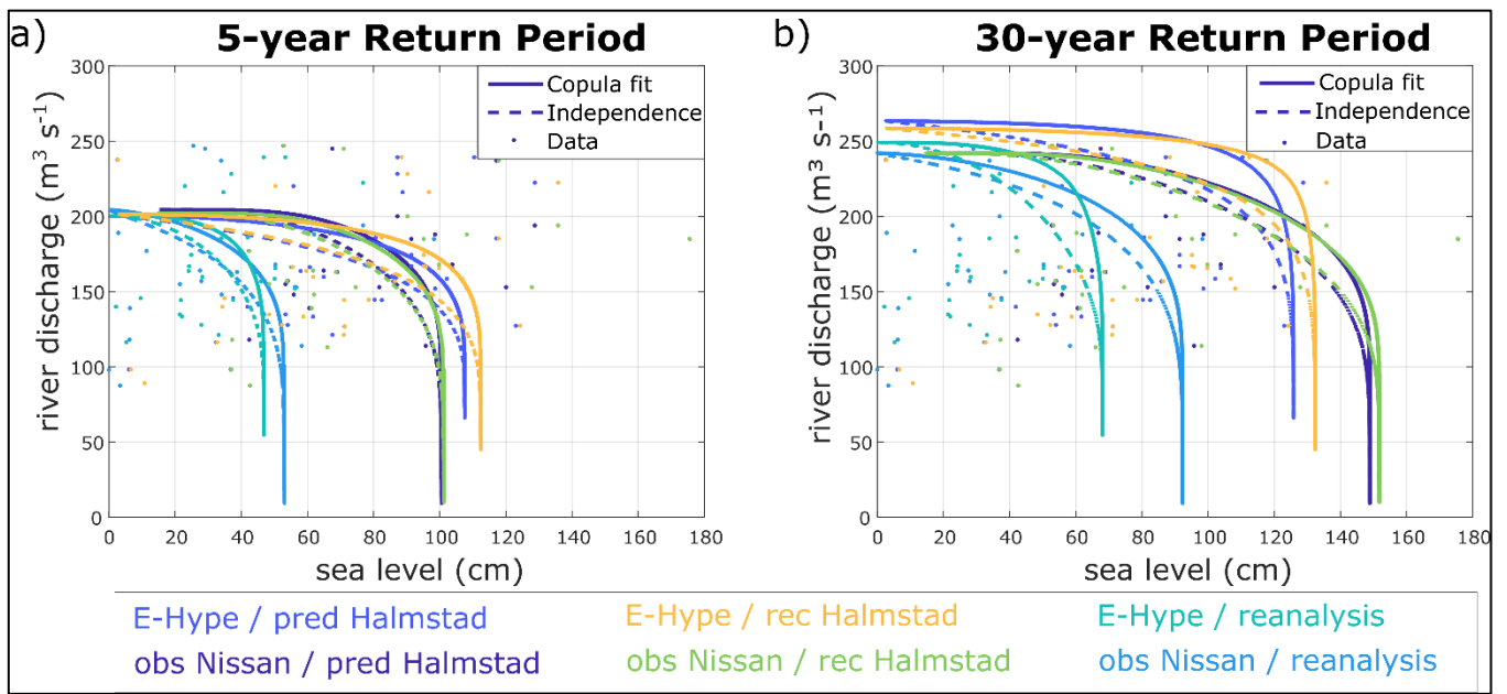
400 Figure 7: 5- (a) and 30-year (b) Return periods isolines for joint probability (AND scenario) of river discharge (y-axis) annual maxima and associated sea level (x-axis) maxima ( Q_n , s_n ) for Halmstad. Full lines implement the compound effect, and dashed lines represent fit, assuming independence between both variables. Dots show observed data. The best copula fit is used to model the dependence of ( Q_n , s_n ) calculated for each set visible in coloured text.
