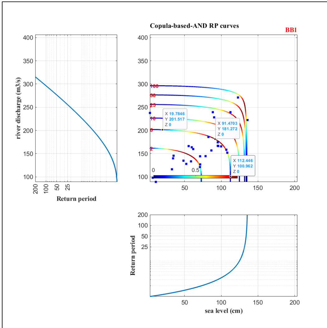
540 Figure A1: Set E-Hype / rec Halmstad, best copula fit: BB1. [2, 5, 10, 25, 50, 100] RPs and associated densities. The left and lower panels correspond to marginal RPs curves of each univariate parameter individually, river discharge and sea level (extracted from MhAST software).
