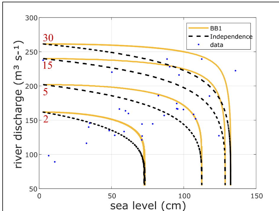
315 Figure 5: RLs for base case set rec Halmstad / E-Hype. Full lines correspond to the return period (RP) isolines for joint probability (AND scenario) of river discharge (y-axis) annual maxima and associated sea level (x-axis) maxima ( Q_n , s_n ). The dashed lines represent the distribution fit, assuming the independence between the variables. Blue dots show observed data. BB1 copula is used to model the dependence of river discharge annual maxima and associated sea level maxima calculated for each RPs visible in red text (2, 5, 15 and 30 years).
