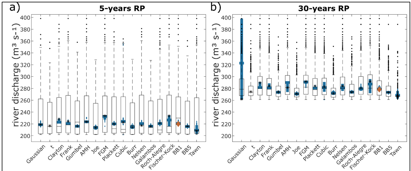
370 Figure 6: Fluvial component in bivariate events with 5- (a) and 30-year (b) Return periods from copula fits for rec Halmstad / E-Hype. Each column represents a copula distribution fit. Stars represent the most likely scenario return values from each copula for each set, and the red diamond is the best copula fit. Two uncertainty approaches are displayed as boxplots, giving a statistical summary. Median, first, and third quartiles are represented in each box, whiskers represent minimum/maximum values, and dots represent outliers. Outlined boxplots correspond to the "Weighted Average" approach, and filled ones to the "Maximum Density" approach. 375
