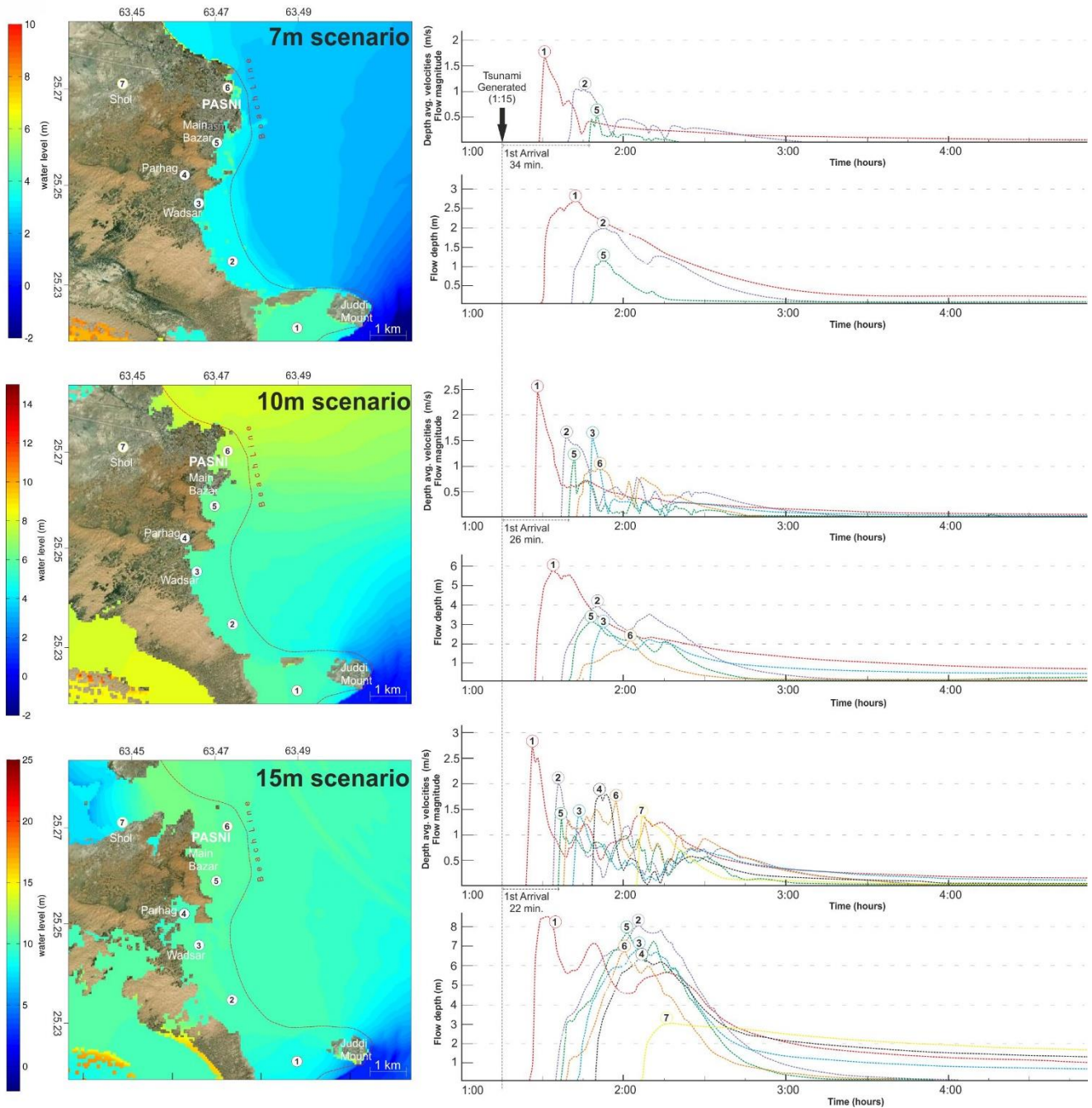
Figure 2: Hydrodynamic modelling results of each scenario with maximum inundation limits and depths at Pasni and surrounding areas. The graphs illustrate the flow depth and magnitude at monitoring points (M1 to M7). Simulation details for each scenario are provided in the supplementary materials.
