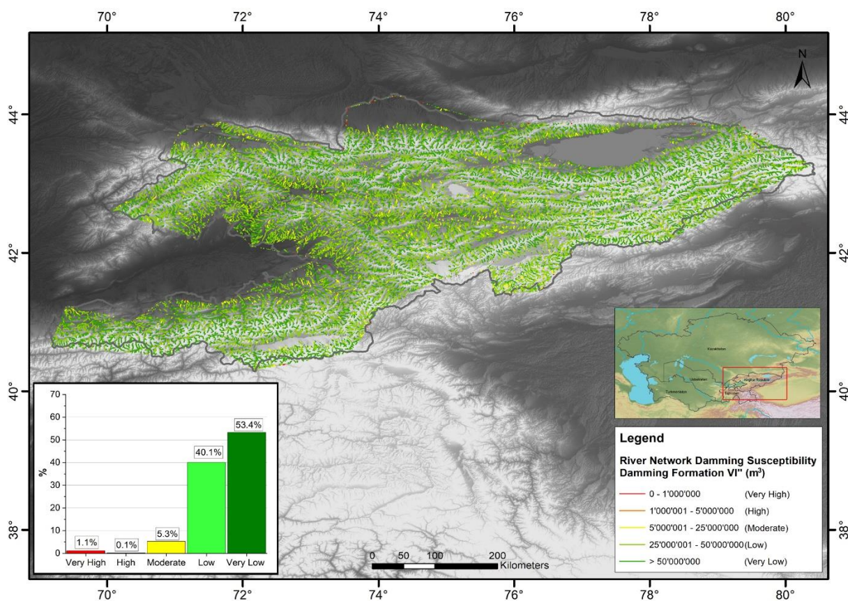
411 412 Figure 17. Damming Susceptibility Map of formation of river stretches by new landslides in the Kyrgyz 413 Republic territory. River network database from Coccia et al., (2023). Topographic base from NASA's SRTM 414 project (Far and Kobrick, 2000).
