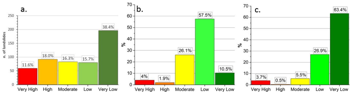
422 Figure 20. Classes distribution in Uzbekistan of the Damming Predisposition for landslides reactivation 423 (a.), Damming Susceptibility of Non-Formation (b.) and of Formation (c.) for new landslides.
