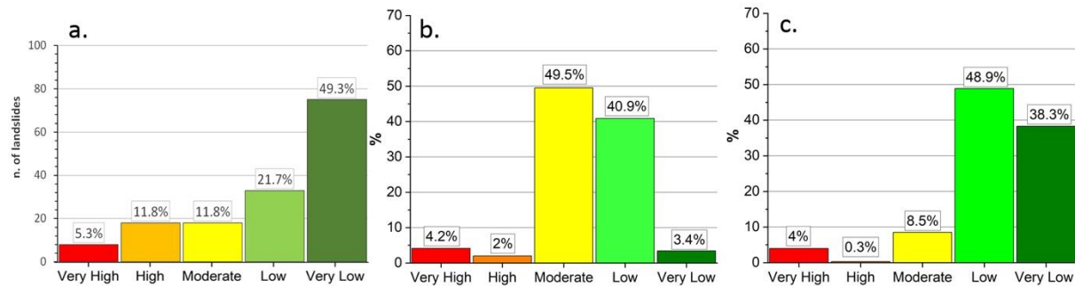
422 Figure 20. Classes distribution in Uzbekistan of the Damming Predisposition for landslides reactivation 423 (a.), Damming Susceptibility of Non-Formation (b.) and of Formation (c.) for new landslides.
