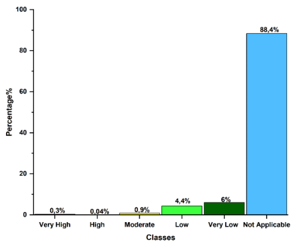
408 409 Figure 16. Distribution of the Damming Susceptibility in the study area by new landslides related to 410 Formation boundary values.
