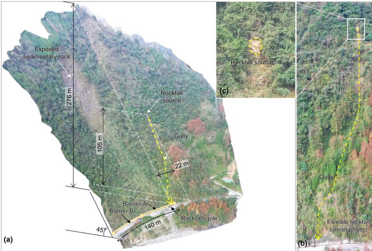
Figure 3: Investigation results of the rockfall source area and trajectory. (a) The digital model of the slope; (b) Rockfall impact gully; (c) Rockfall source.
