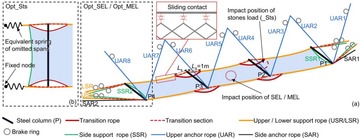
Figure 16: Structure representation of the model Opt_. (a) Simulation models Opt_SEL and Opt_MEL. (b) Simulation model Opt_Sts.
