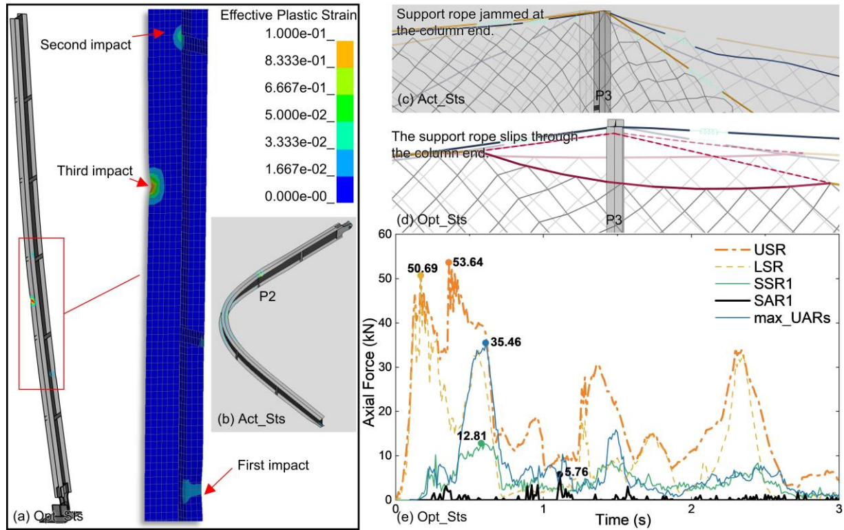
400 Figure 19: Opt_Sts calculation result: (a) The column P2 in Opt_Sts got local damages after several hits. (b) The column P2 in Act_Sts was buckling. (c) and (d) are the support rope sliding performance on the end of column P3 in Act_Sts and Opt_Sts, respectively, where semi-transparent for pre-impact and saturated colour for post-impact. (e) The internal force of part of the wire ropes in Opt_Sts.
