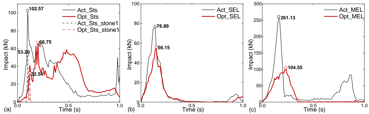
Figure 18: Temporal evolution of the impact of rockfalls and barriers
