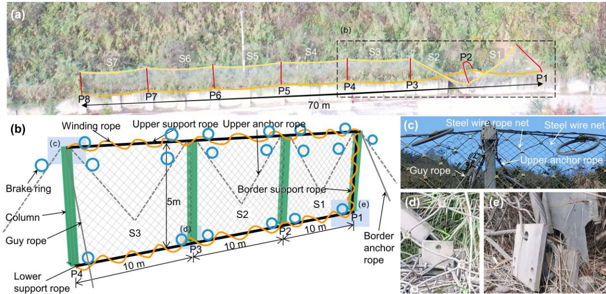
Figure 5: Structure composition of the flexible barrier. (a) Overall photo of the project; (b) Components connection relationship; (c) Details of column head; (d) Failure of column base at the mid-span; (e) Failure of border column base.
