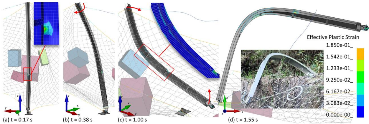
Figure 11: Column P2 deformation development in Act_Sts.
