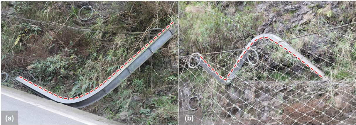
90 Figure 2: Steel column buckling forms of the other two flexible rockfall barrier projects: (a) "C"-shaped compression buckling and (b) "S"-shaped bending and torsion buckling.
