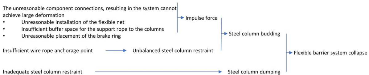
Figure 14: Analysis of the system damage mechanism of Act_Sts.
