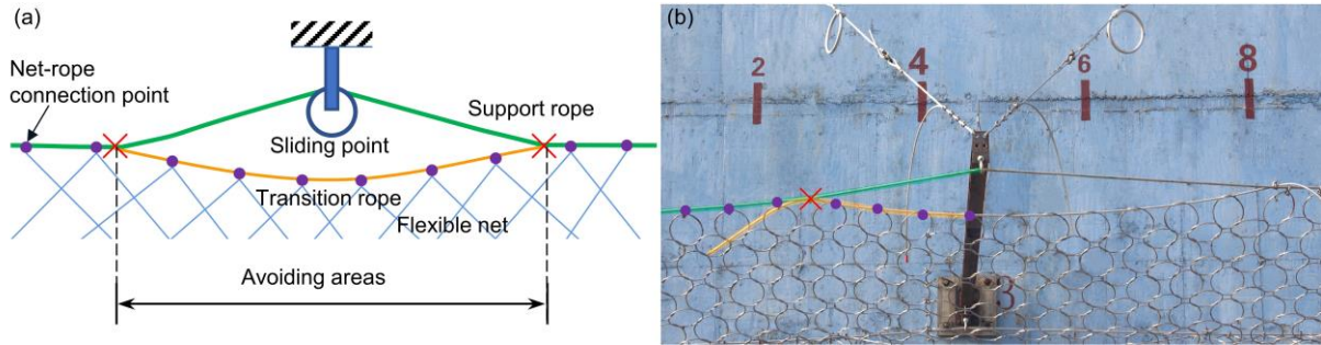
Figure 15: The transition rope applied between column ends and support ropes: (a) Structure schematic and (b) project photo.
