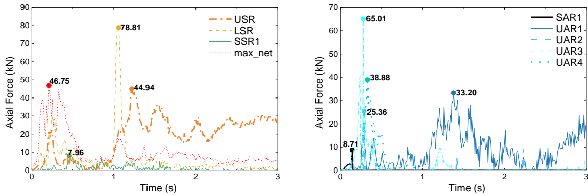
Figure 12: Axial force of the wire ropes in Act_Sts
