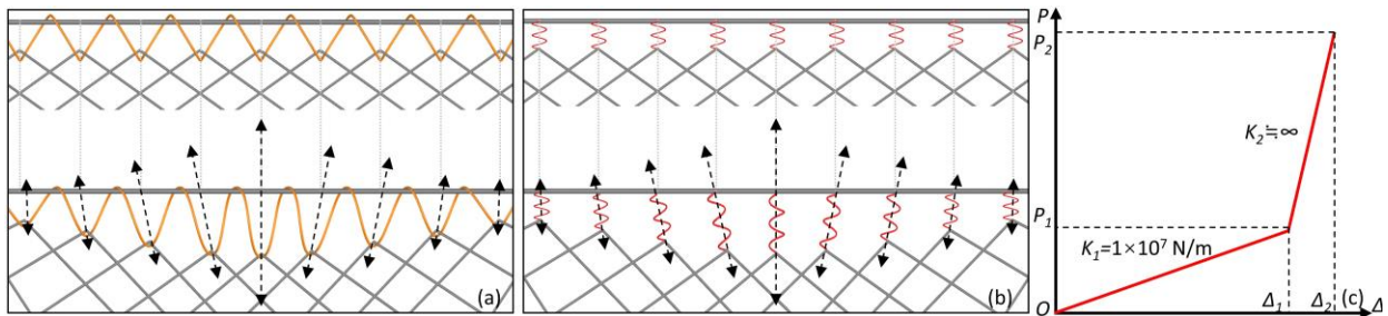
Figure 9: Spring equivalent model for winding rope. (a) Before and after winding rope deformation. (b) Before and after spring equal model deformation. (c) Bilinear constitutive model of the winding rope spring.
