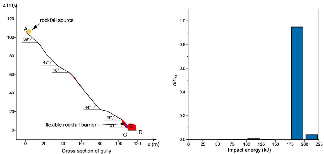
Figure 7: Rock mobility analysis : (a) Trajectory of rockfall and (b) Probability distribution of kinetic energy of falling rocks at the flexible barrier.
