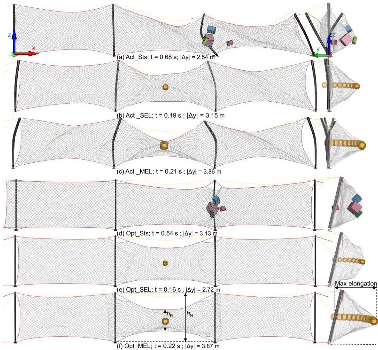
Figure 17: System forms at the moment of maximum y-directional elongation.
