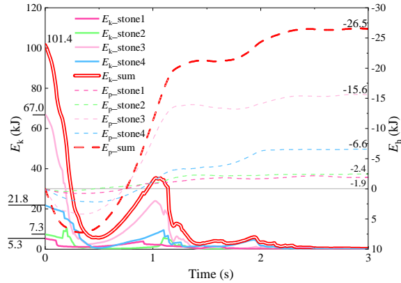
280 Figure 13: Temporal evolution of kinetic energy and potential energy of rockfalls.
