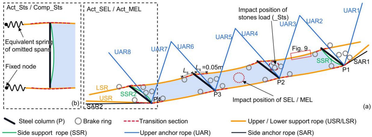
Figure 8: Structure representation of the actual model (Act_) and the comparative analysis model (Comp_). (a) Act_SEL and Act_MEL. (b) Act_Sts and Comp_Sts.
