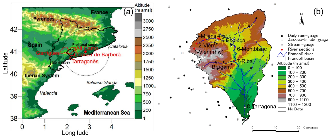
Figure 1. (a) Main geographical features of north-eastern coast of Spain. The location of the Barcelona weather radar from Spanish Agency of Meteorology is shown as a red dot. The Francolí catchment is highlighted in thick black line. Radius of the radar circle is 100 km. The municipalities traversed by the Francolí river are also shown in red. (b) Main geographical features of the Francolí basin. The automatic rain-gauges are shown as white dots. Automatic stream-gauges are labelled and depicted as white squares. Daily pluviometers are illustrated as black dots. River sections are denoted as red circles and labelled downstream.
