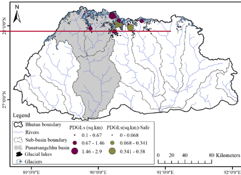
Figure 1. A map showing the rivers and basin system of Bhutan, as well as the distribution of potentially dangerous glacial lakes. Bubbles are scaled to total lake area and color coded for classification. Data source: National Center for Hydrology and Meteorology (NCHM).
