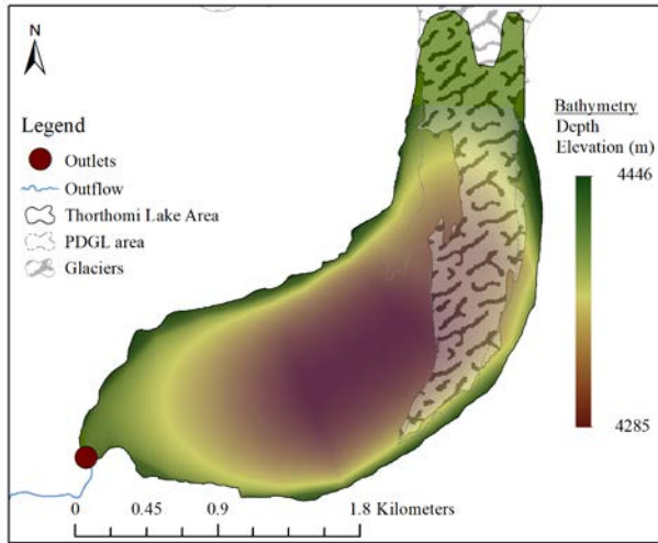
Figure 9. The estimated bathymetry of Thorthomi Lake.
