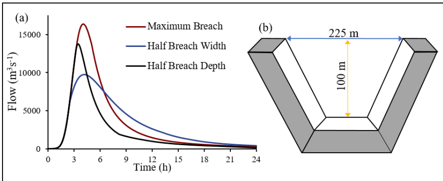
Figure 10. (a) A dam breach outflow hydrograph obtained from the BREACH model for three different scenarios; and (b) breach parameters, breach width ( \leftrightarrow ), and breach depth ( \Uparrow ) in metres for the maximum breach scenario.
