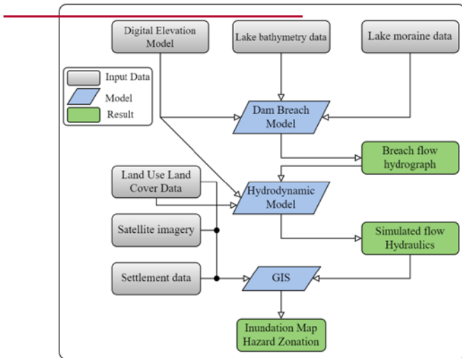
Figure 2. A schematic diagram of the methodology employed in our study. Input data used for the study are indicated with grey boxes, models are indicated with blue boxes, and results are indicated with green boxes.
