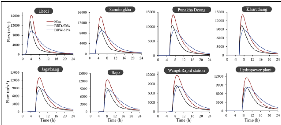
520 Figure 11. A simulated flow hydrograph at important locations, derived from the HEC-RAS result for each scenario. (Max: maximum breach, BRD-50%: half of maximum breach depth, BRW: half of maximum breach width).
