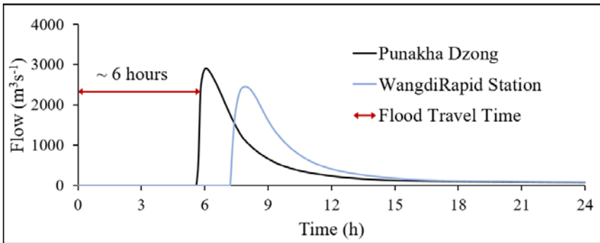
475 Figure 8. A simulated GLOF hydrograph at different locations along the flow path.
