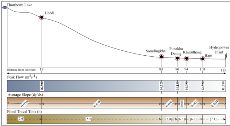
535 Figure 12. A schematic representation of flood parameters at six important locations along the flow path for the maximum breach scenario.
