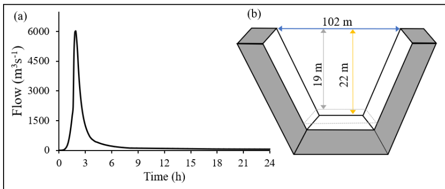
Figure 7. (a) A breach outflow hydrograph from the BREACH model; and (b) an illustration of breach parameters, breach width ( \leftrightarrow ), breach depth ( \updownarrow ), and the change in water surface elevation ( \updownarrow ).
