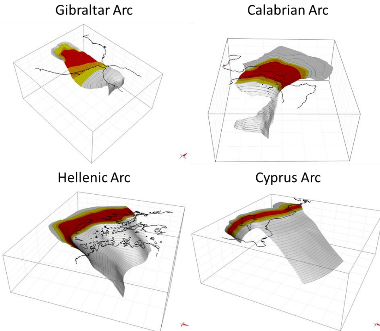
Figure 4: Oblique views of the tri-dimensional geometry of the four slab models. The vertical extent of all boxes is 300 km. The colored part of the slab top surface represents the extent of the seismic interface, including the uncertainty represented by the upper and lower seismogenic depths (see Figure 2).
