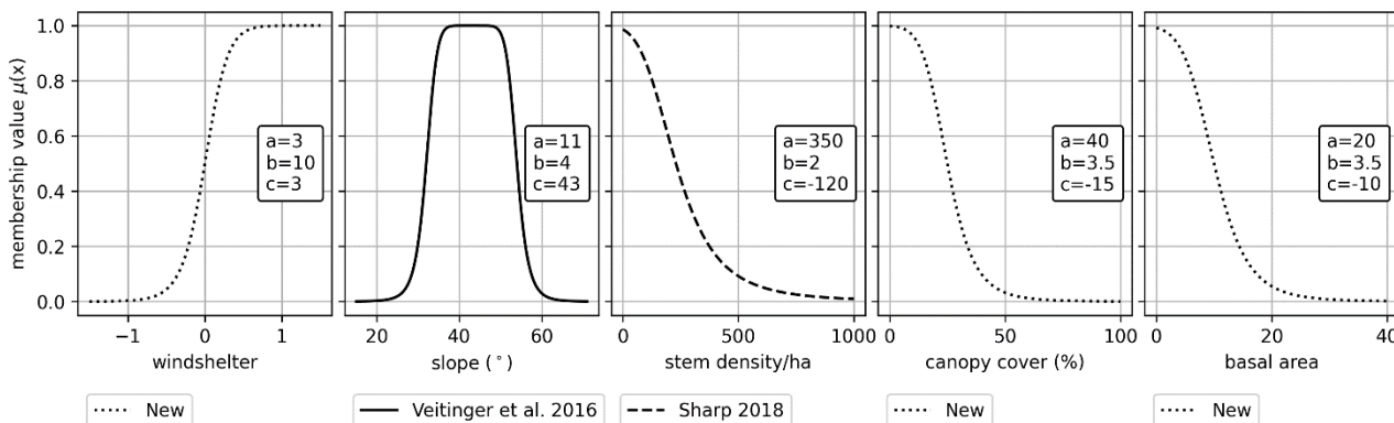
245 Figure 2: The different Cauchy functions used by Veitinger et al. (2016) and Sharp (2018) for slope angle and stem density. The values a, b and c are inputs for the Cauchy membership value (Eq. 1). We have suggested new membership values for windshelter, canopy cover (%) and basal area. We recommend that these values are fine-tuned for specific datasets and applications. Read a more in-depth discussion of this in section 4.3.
