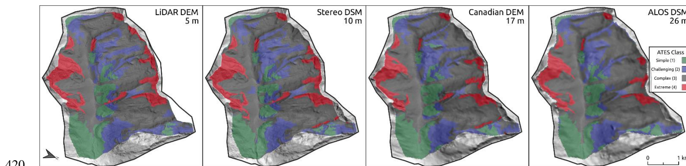
420 Figure 12. DEM sensitivity analysis for Connaught Creek study area, showing the spatial patterns between the output have some variation but are largely consistent despite vastly different accuracy of the input DEM data.
