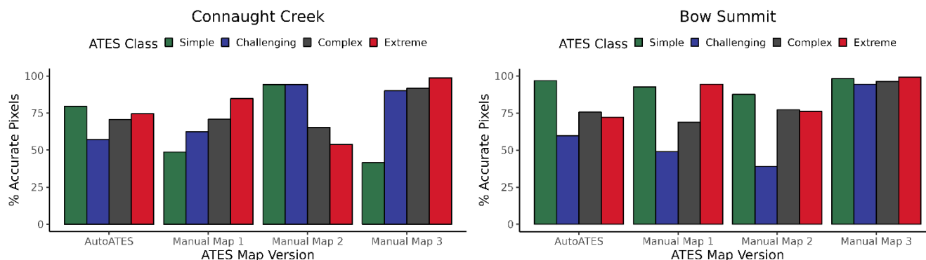
400 Figure 11. Performance of AutoATES and three human mappers compared to ATES benchmark map for Connaught Creek (left) Bow Summit (right) color coded by ATES class simple (green), challenging (blue), complex (black), and extreme (red) terrain
