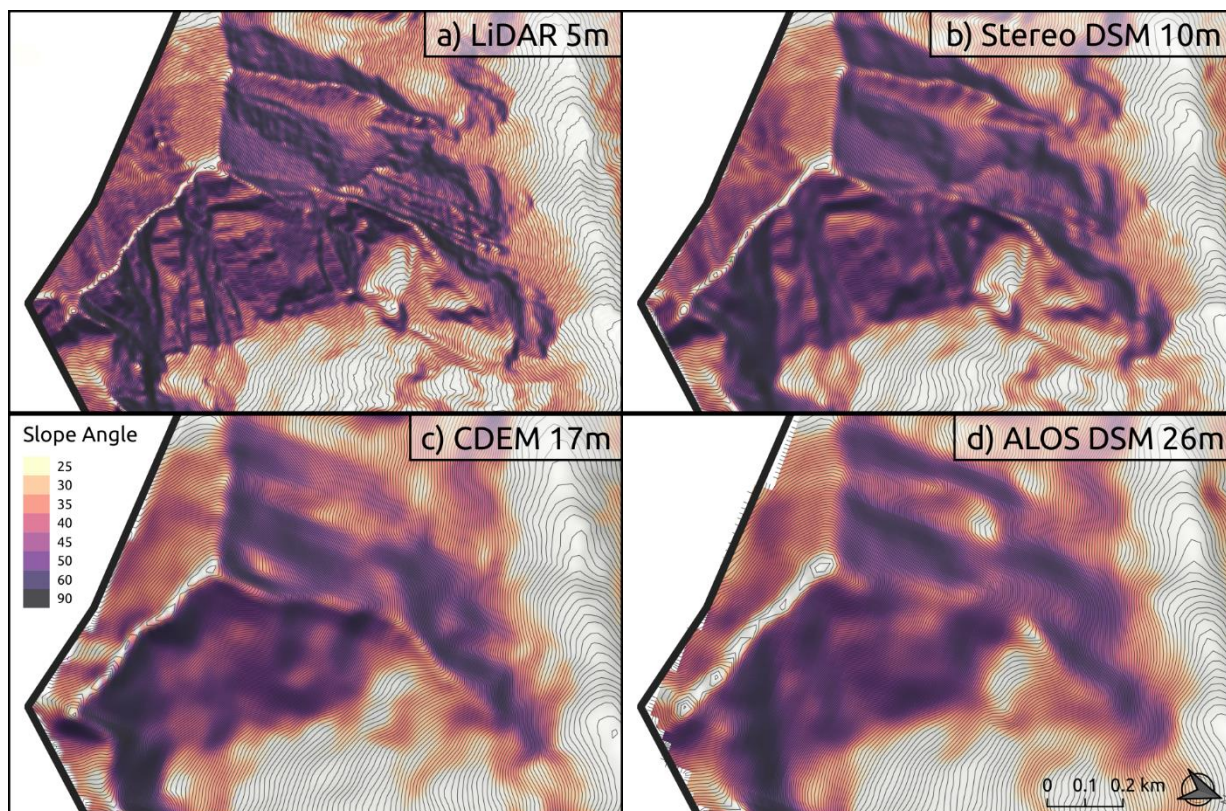
Figure 6. Slope angle rasters from the LiDAR DEM (a), satellite stereo DSM (b), Canadian national DEM (c), and ALOS DSM (d). The wide variety of DEM data illustrate the smoothing effect of lower resolution input data.
