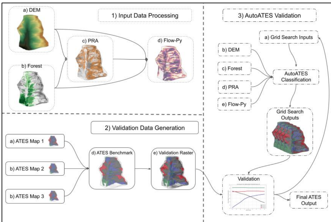
160 Figure 3: Automated ATES processing and validation workflow.
