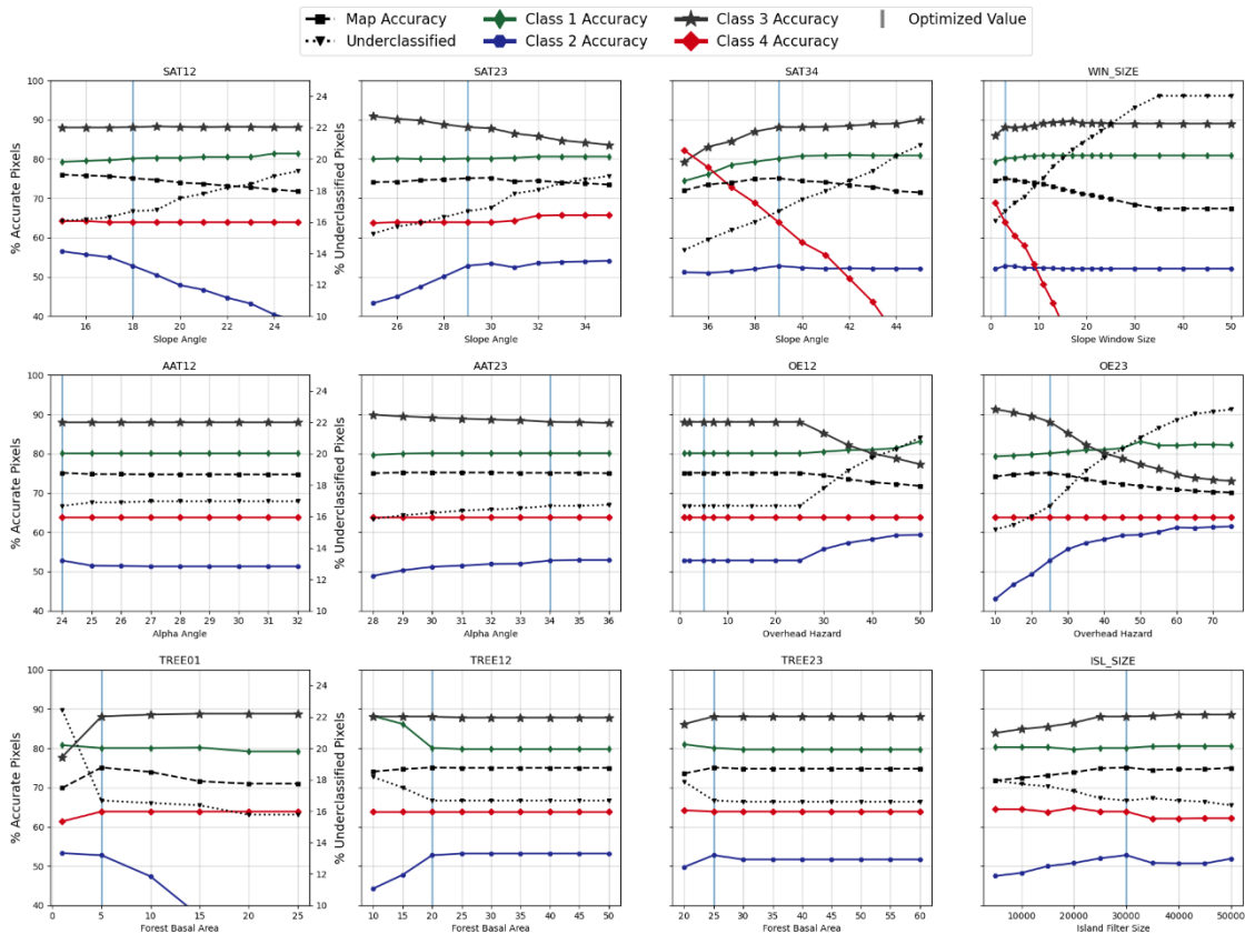
315 Figure 7. Results of the grid search procedure for the Connaught Creek study area. To select optimal parameter values, we considered overall accuracy, percent underpredicted, and balanced accuracy across ATEs classes.
