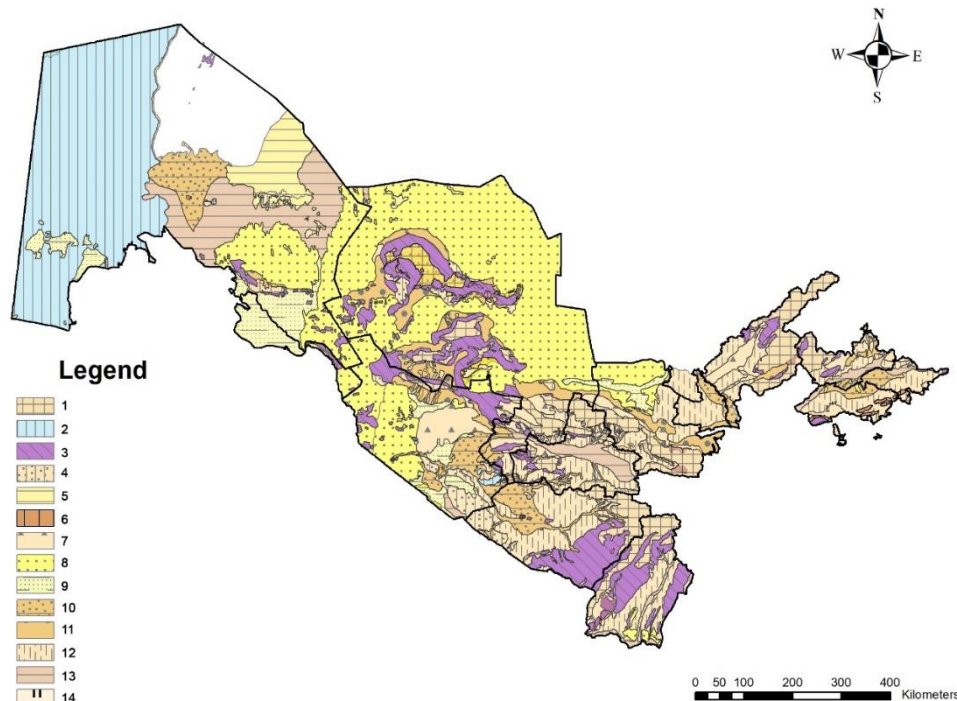
Fig. 1: Engineering-geological map of Republic of Uzbekistan. Autors: Islamov et al. (1968). 1-Rock soil; 2-Limestone; 3-Sand and sandstone; 4-Clay and sand; 5-Clay, marl, sandstone; 6-Clay, sandy clay, sand; 7-Gravel; 8-Sand; 9-Sand, sandy clay, sand; 10-Sandy loam, sand; 11-Gravel, pebble, rubble; 12-Loess, loess loam, and sandy clay; 13-Clay, loam and sandy clay; 14- Gypsum, loam and clay.
