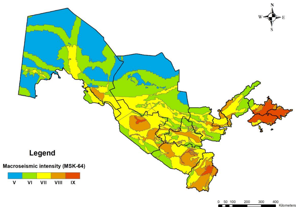
155 Fig. 3. The schematic map of seismic intensity in the territory of the Republic of Uzbekistan.
