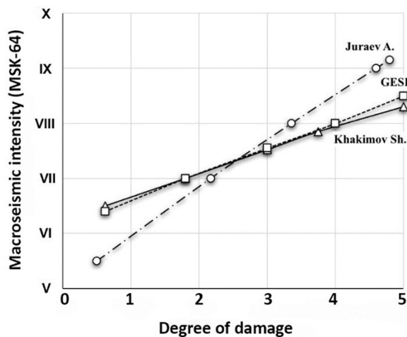
Fig. 7: Graph of changes in the average degree of damage to individual mudbrick houses depending on the seismic intensity according to different authors.
