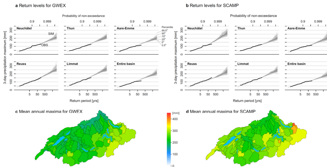
Figure 4. Top: Empirical return levels obtained for MAP3d (3-day mean areal precipitation) from the 30 time series of 10 000 years generated with GWEX (a) and SCAMP (b) for the entire Aare River basin and five main sub-regions using the Gringorten plotting position. The bounds of the grey shaded areas correspond to the 0.5/99.5 th , 5/95 th and 25/75 th percentiles of the 30 time series, respectively. Bottom: Mean maximum simulated MAP3d from the 30 × 10 000 year time series for each of the 79 HBV sub-catchments (c: GWEX, d: SCAMP); major lakes are drawn in cyan. Note that the largest simulated MAP value in one 10 000-year long simulation corresponds to a return period of 18 000 years (Gringorten plotting position). Also note that the extreme MAP values mapped do not necessarily occur simultaneously, i.e., do not correspond to one single event.
