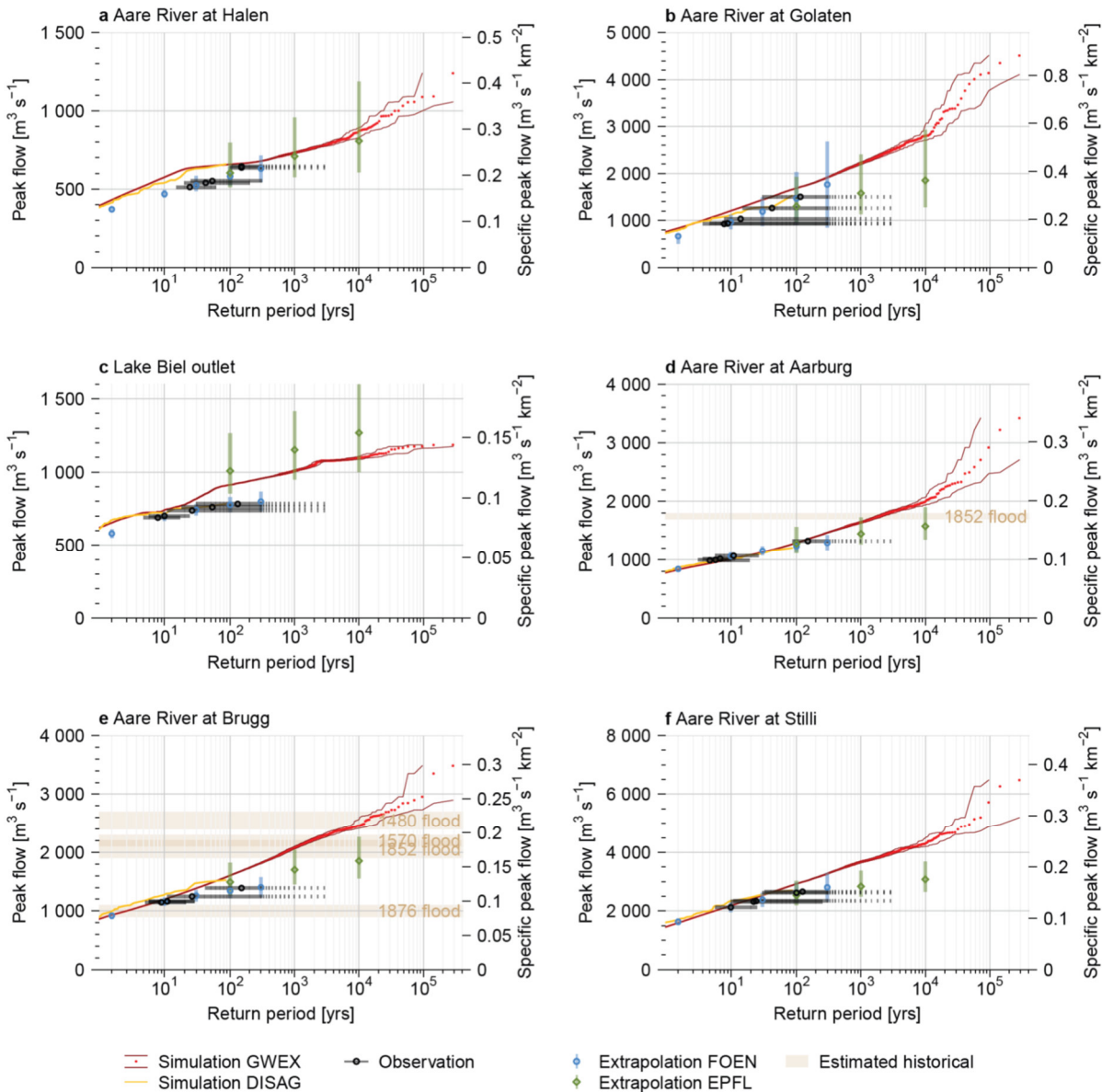
425 Figure 7. Exceedance curves for selected sites along the Aare River: Halen, Golaten (downstream of the confluence with the Saane River), outlet of Lake Biel (close to Brügg-Aegerten), Aarburg (downstream of the confluence with the Emme River), Brugg (upstream of the 430 confluence with the Reuss and Limmat Rivers) and Stilli (downstream of the confluence with the Reuss and Limmat Rivers). Red: AMFs for CS (median representative parameter set) based on 289 000 years of GWEX weather scenarios, with the central 95% confidence interval 435 computed according to Loucks and van Beek (2017); orange: simulated AMFs (median representative parameter set) on the basis of 85 years of disaggregated weather observations (DISAG); black: 5 highest observed peak flows plotted at return periods according to FOEN with confidence interval (Baumgartner et al., 2013) (confidence intervals that are unbounded towards high return periods are drawn in dash); blue: extrapolation of observed peak flow records according to FOEN with confidence interval (Baumgartner et al., 2013); green: regionally enhanced extrapolation of observed peak flow records according to EPFL with confidence interval (Asadi et al., 2018); light brown (for Brugg and Aarburg only): range of reconstructed historical floods (Baer and Schwab, 2020). Observation and reconstruction sites do not always match simulation sites exactly; the corresponding values have been scaled where necessary, assuming constant discharge per unit area.
