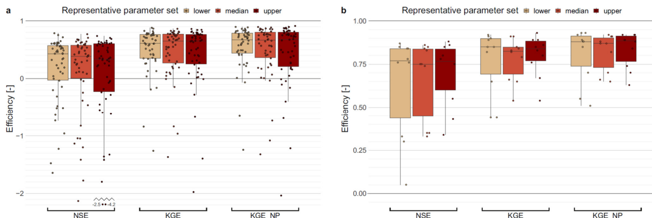
Figure 6. Model efficiencies at hourly time-step over the period 1974–2015 for HBV (a, 49 gauged sub-catchments) and RS Minerve (b, 10 gauged output nodes) showing the three representative parameter sets. The efficiency criteria used are Nash-Sutcliffe (NSE), Kling-Gupta (KGE) and non-parametric Kling-Gupta (KGE_NP). All criteria have an upper bound of 1 (which means ideal performance), and are unbounded towards the bottom.
