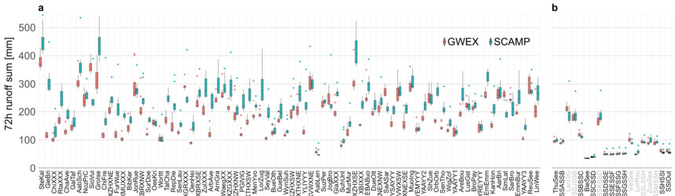
Figure 14. Comparison of hydrological results achieved with GWEX inputs (red) and SCAMP inputs (blue). Shown are boxplots for the ten largest 72-hour runoff sums (median representative parameter set), each for the outlets of the 79 individual HBV sub-catchments (a, ordered by increasing catchment area) and the 19 RS Minerve nodes (i.e., critical sites including Aare River outlet) (b, ordered by location along the Aare River, tributaries are designated with grey label colour). For the sub-catchment and output node abbreviations see Supplementary Tables 2 and 3.
