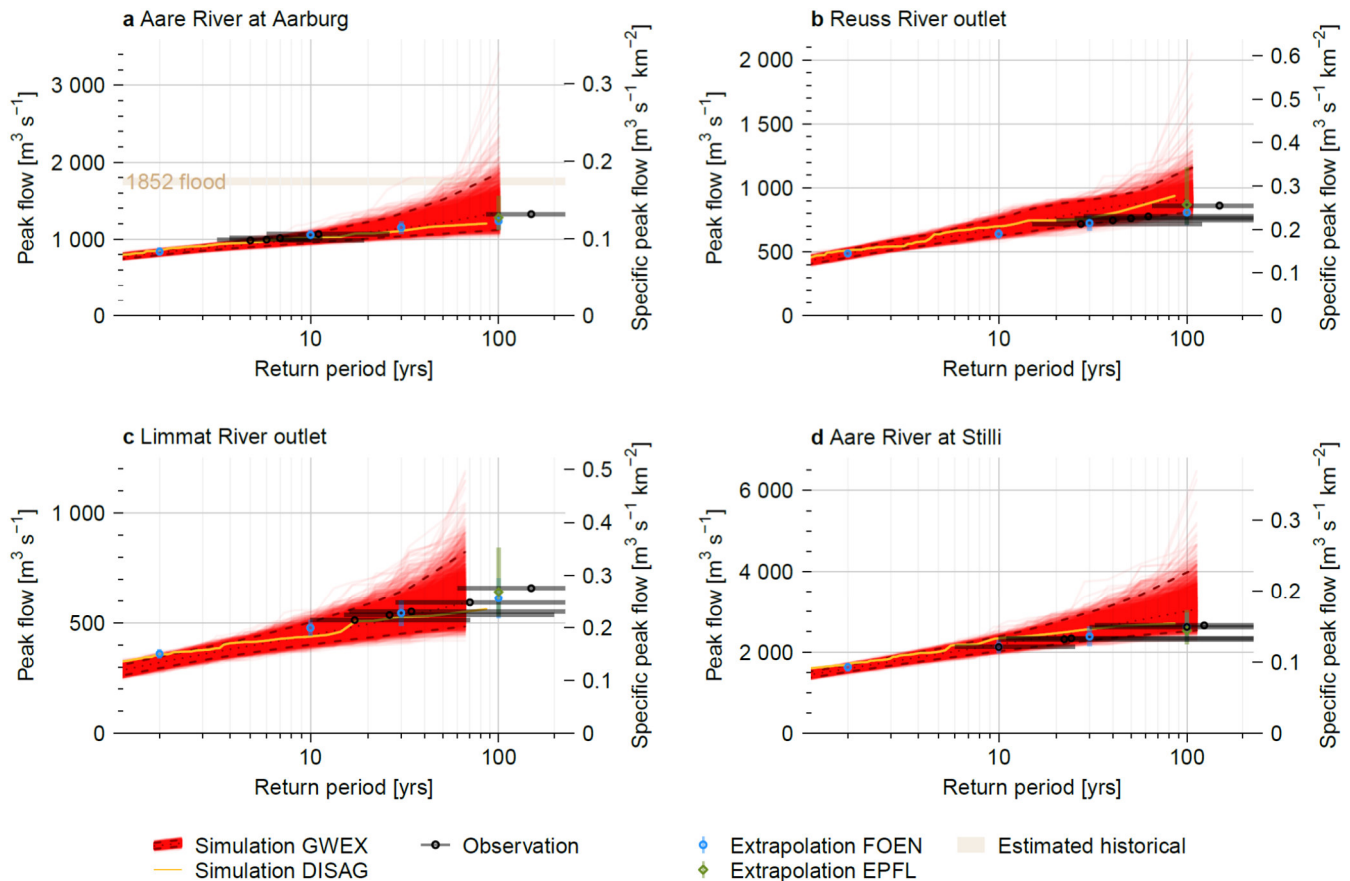
Figure 13. Exceedance curves for AMFs from 289 000 years of CS based on GWEX weather generator scenarios (red), split up into blocks with length equal to that of observed peak flow records. Results are shown for the Aare River at Aarburg (a, block length 100 years), the outlets of rivers Reuss (b, 106 y) and Limmat (c, 65 y), and for the Aare River close to the outlet at Stilli (d, 112 y). Orange: AMFs from 85 years of simulation (median representative parameter set) using disaggregated weather observations 1930–2014 (DISAG); black: top-5 observed peak flows drawn at return periods estimated by FOEN (Baumgartner et al., 2013); blue: extrapolation of observed peak flow records by FOEN (Baumgartner et al., 2013); green: regionally enhanced extrapolation of observed peak flow records according to EPFL (Asadi et al., 2018); light brown (for Aare at Aarburg only): range of reconstructed historical floods (Baer and Schwab, 2020). Measurement sites do not always match simulation sites exactly; the corresponding observations and extrapolations have been scaled where necessary, assuming constant discharge per unit area.
