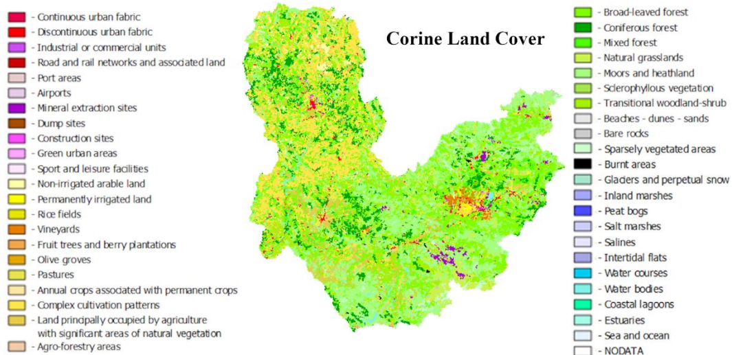
610 Figure 2: General land uses defined by Corine Land Cover and their distribution for the area under scope.
