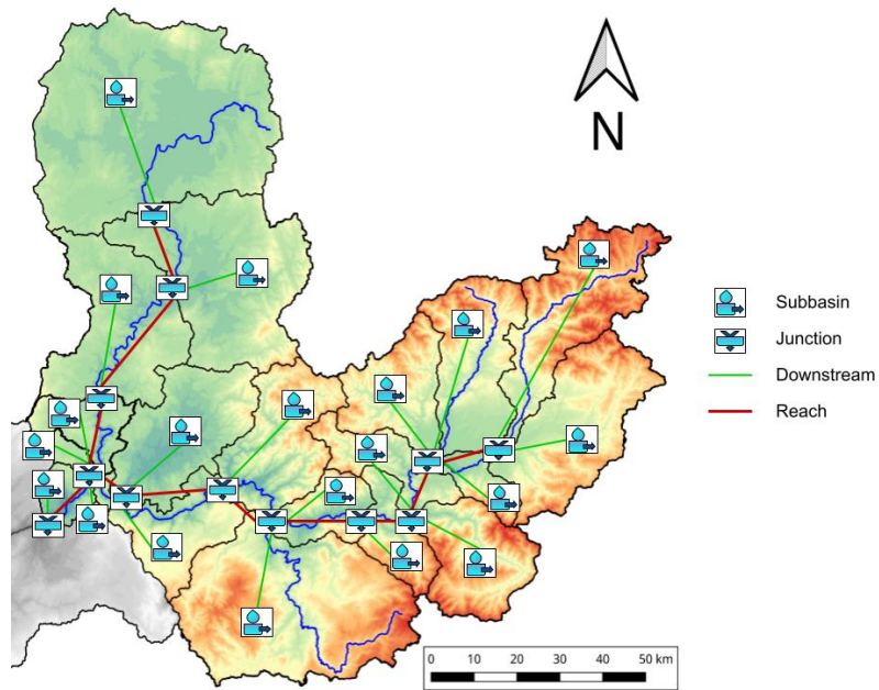
615 Figure 3: Map with the hydrological characterization of the basin under scope attending to its topographical features. Subbasin is referred to the divisions of the basin under scope, Junction is referred to the points in the flow network where multiple inflows combine, Downstream is referred to the point in the main river channel where each subbasin flows, and Reach represents the main river channels.
