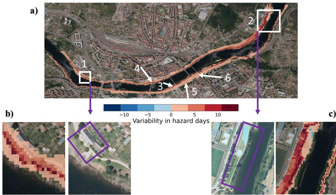
655 Figure 9. (a) Future variability in the number of days under hazard by floods in Ourense city. The increase (decrease) in the number of cases is obtained subtracting for each pixel of the domain the number of days under flood hazard situation in the historical period from the hazard cases in the future period. Thus, red (blue) colors represent the increase (decrease) in the flood hazard considering the average of all models. Only the area outside the riverbed was taken into account for the flood risk analysis. In lower panels two important areas of the city are shown in detail, (b) Chavasqueira thermal baths and (c) Oira park. 660 (Aerial pictures courtesy of PNOA © Instituto Geográfico Nacional).
