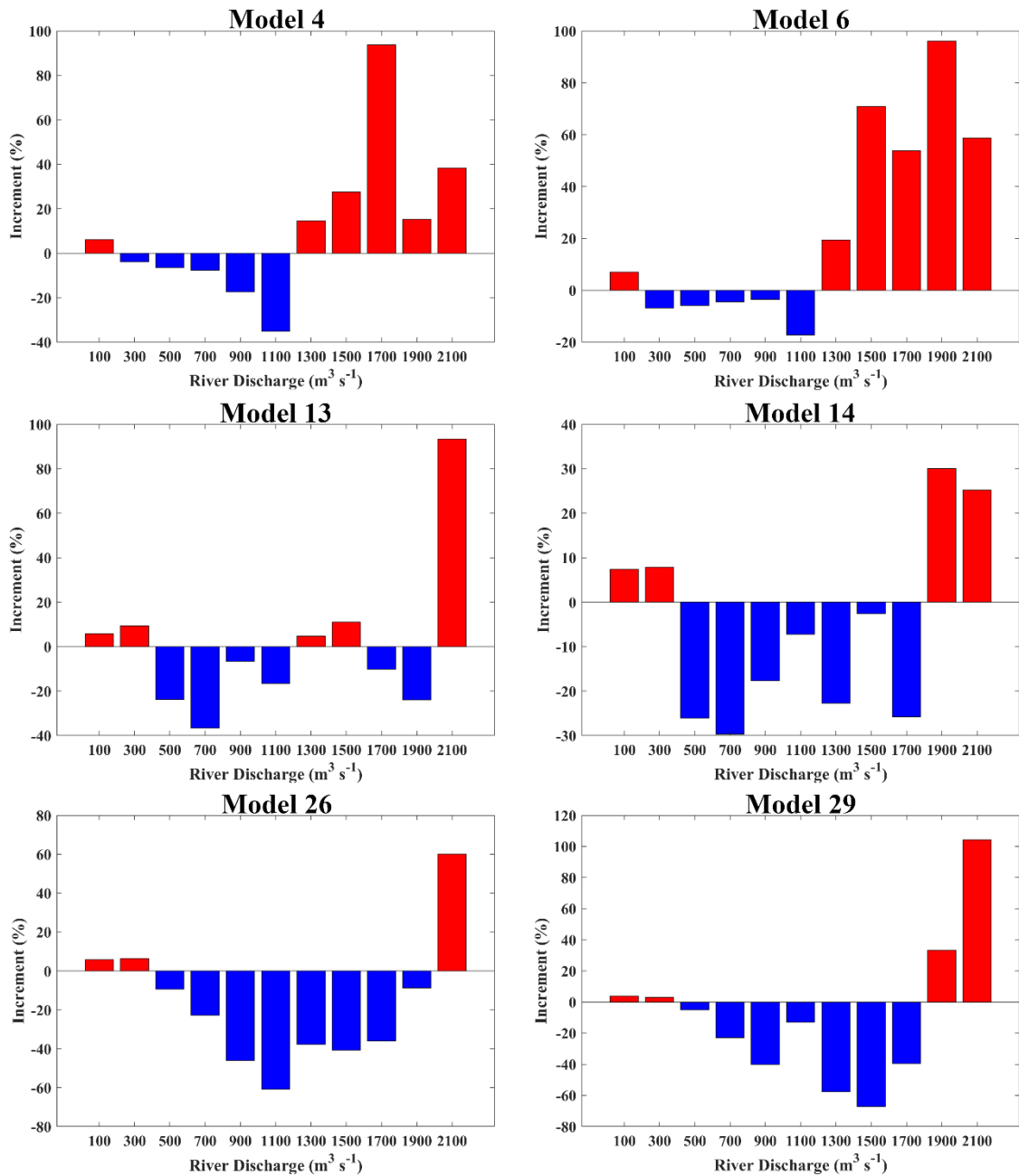
625 Figure 5. Percentage of change in the frequency of river flow ranges in the future with respect to the historical period for each valid model. The river flow data was distributed in ranges of 200 \text{ m}^3 \text{s}^{-1} . Each value of the river discharge indicates the mean of the corresponding range ( 100 \text{ m}^3 \text{s}^{-1} corresponds to the range of 0\text{--}200 \text{ m}^3 \text{s}^{-1} ). In the last range ( 2100 \text{ m}^3 \text{s}^{-1} ), the river flows surpassing the alert threshold ( 2000 \text{ m}^3 \text{s}^{-1} ) are included. Positive (negative) values indicate increase (decrease) in the future.
