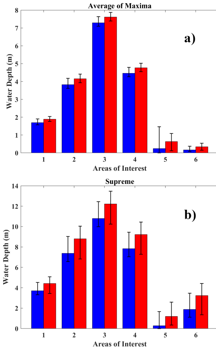
665 Figure 10. (a) Mean of maxima and (b) supremum water depths in important areas of Ourense for the historical (blue) and future (red) periods considering the average of all models. Areas under analysis are named from 1 to 6: Chavasqueira thermal baths, Oira Park, Antena fluvial beach, Ribeira de Canedo park, Miño park, and N-120 road. Black bars represent the multi-model deviation.
