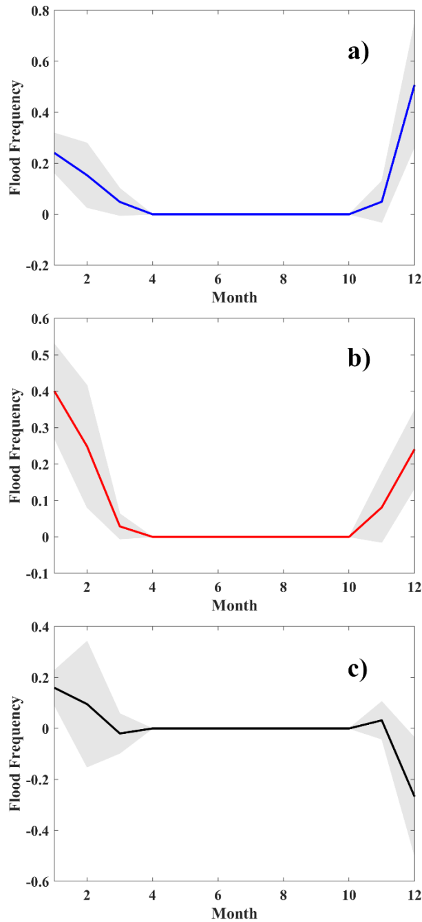
640 Figure 7. Multi-model mean of the monthly flood frequencies for the (a) historical and (b) future periods. Frequencies were calculated dividing the flood alerts detected in each month by the total number of alerts. Thus, the sum of the frequencies of all months is equal to 1. (c) Differences in flood frequency between historical and future periods. Positive (negative) values indicate an increasing (decreasing) of flood frequency in the future. Grey shadow areas represent multi-model deviation.
