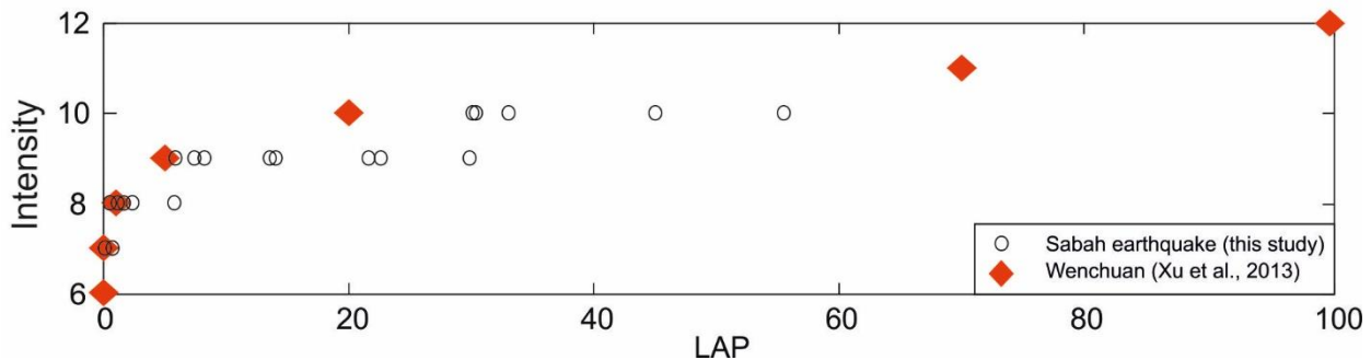
Figure 9: Plots of LND (a) and LAP (b) vs ESI-07 values; small black circles are the median values for the Sabah earthquake, obtained with the different scaling laws. Red diamonds are the values proposed by Xu et al. (2013) for the 2008 Wenchuan earthquake. This study adopts the ESI-07 scale, while the classes by Xu et al. (2013) refer to the Chinese intensity scale.
