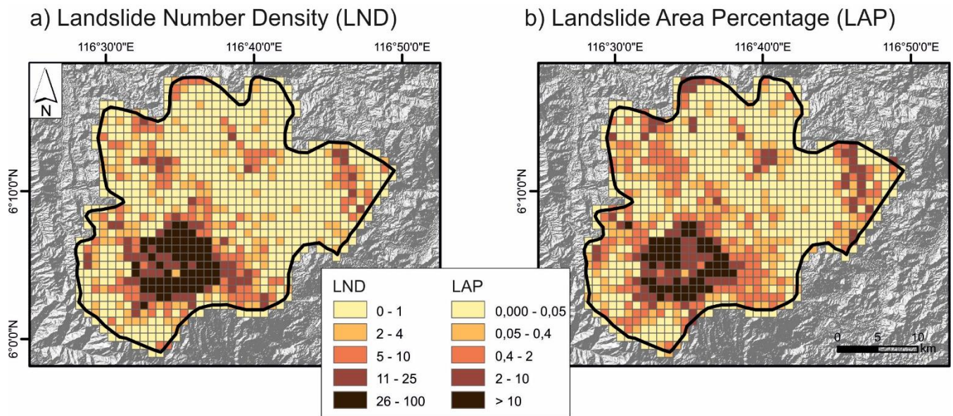
Figure 4: Grid maps of Landslide Number Density (LND, a) and Landslide Area Percentage (LAP, b). Colormap follows Cramer et al. (2020).
