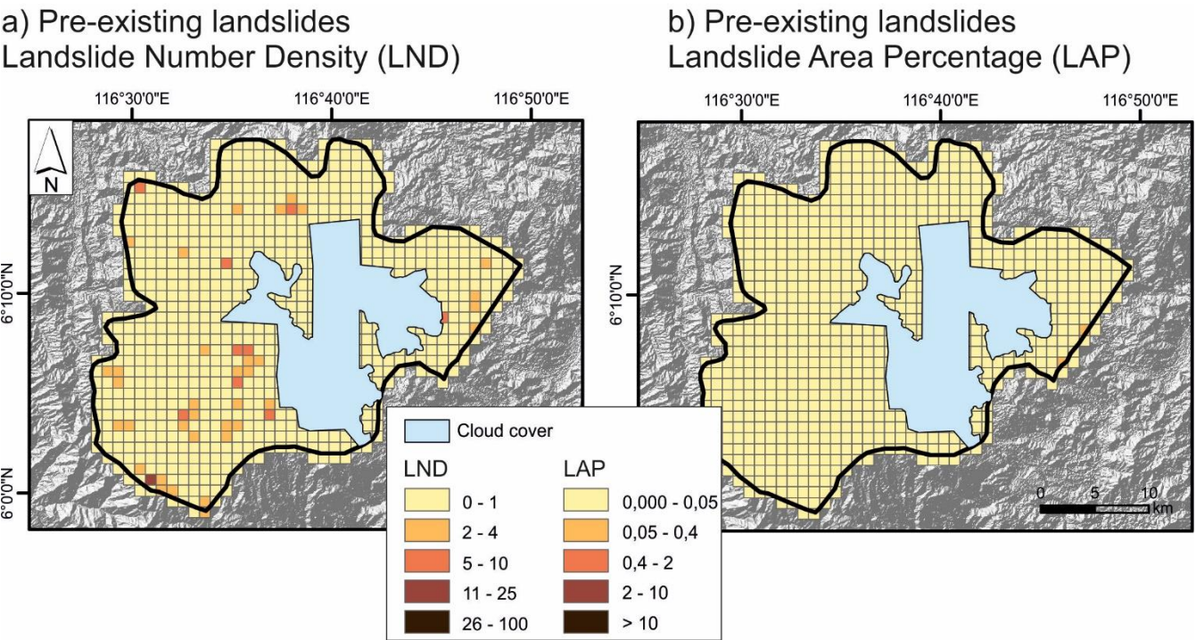
Figure 6: Grid maps of Landslide Number Density (LND, a) and Landslide Area Percentage (LAP, b) for pre-existing landslides; the blue area represents a region where cloud-free pre-earthquake imagery is lacking. Colormap follows Crameri et al. (2020).
