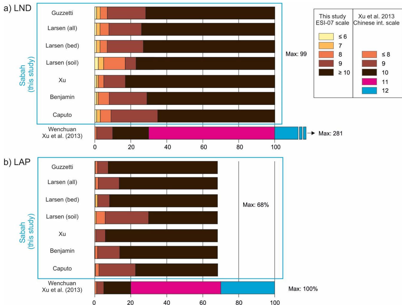
Figure 9: Comparison among LAP and LND classes proposed for the Sabah and Wenchuan earthquakes (this study and Xu et al., 2013, respectively). This study adopts the ESI-07 scale, while the classes by Xu et al. (2013) refer to the Chinese intensity scale.
