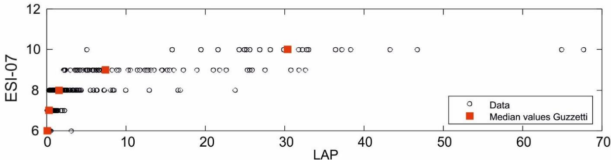
Figure 8: Plots of LND (a) and LAP (b) vs local ESI-07; intensity computed using the Guzzetti et al. (2009) scaling relation is shown as an example.
