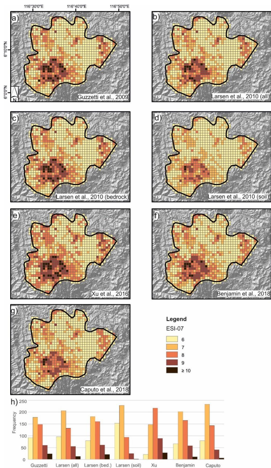
Figure 5: Grid maps of ESI-07 local intensity obtained by adopting different area-volume scaling relations.
