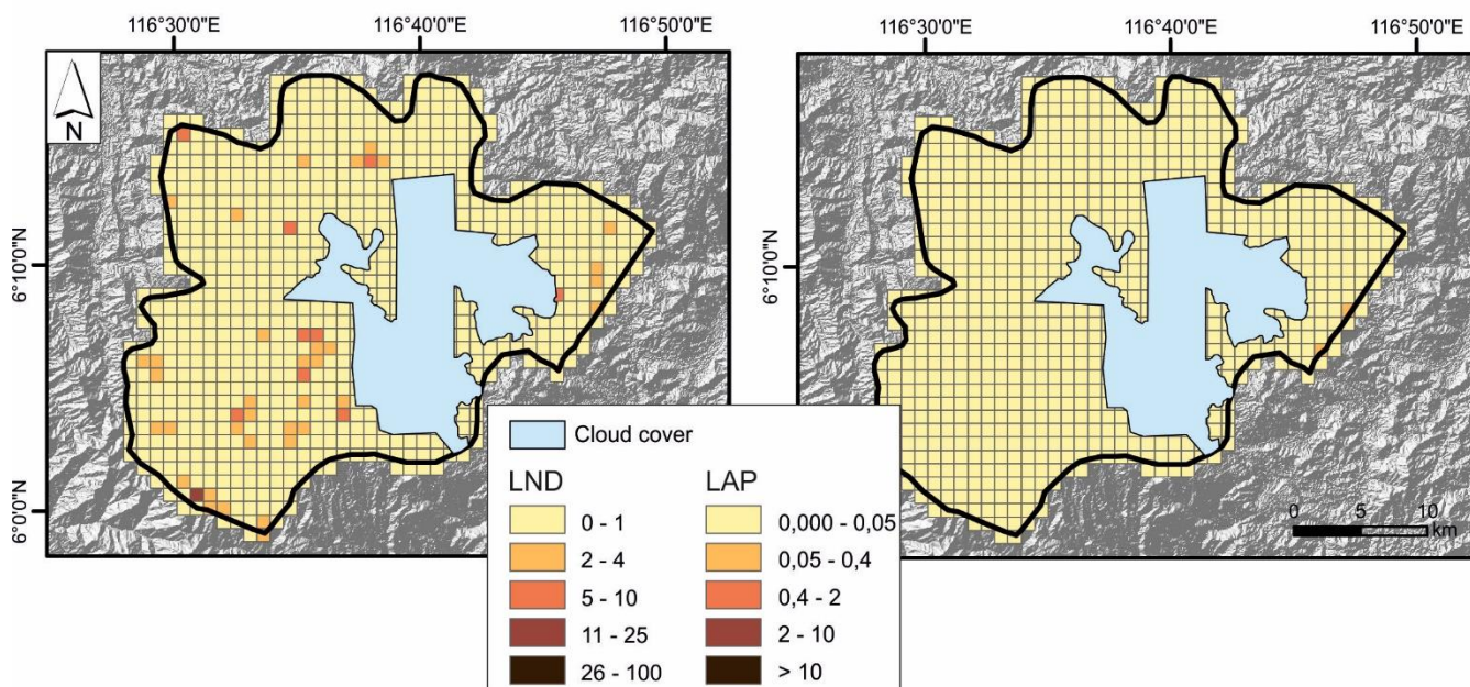
Figure 6: Grid maps of Landslide Number Density (LND, a) and Landslide Area Percentage (LAP, b) for pre-existing landslides; the blue area represents a region where cloud-free pre-earthquake imagery is lacking. Colormap follows Crameri et al. (2020).
