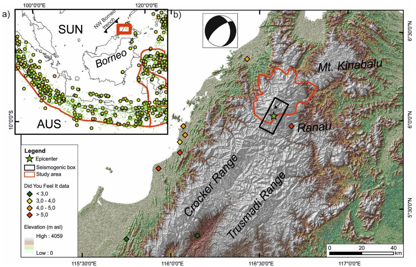
Figure 1: a) Regional seismotectonic setting of SE Asia showing main plate boundaries and M > 5 earthquakes (USGS/NEIC catalogue); AUS: Australian Plate, SUN: Sundaland block; the red rectangle marks the area enlarged in b. b) Digital elevation model derived from 30-m resolution ALOS DEM; focal mechanism is from USGS, epicenter and seismogenic box after Wang et al. (2017); intensity data from DYFI program are shown as well.
