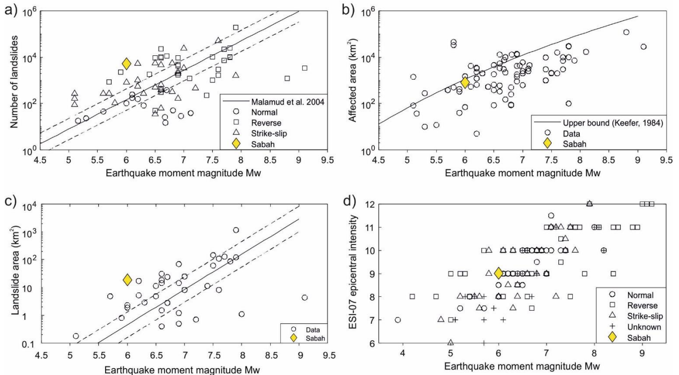
305 Figure 7: Comparison of the Sabah earthquake with global studies: a) number of landslides vs Mw, regression is Equation (2); b) affected area vs Mw, upper bound after Keefer, 1984; c) landslide area vs Mw, regression is Equation (3); d) ESI-07 epicentral intensity.
