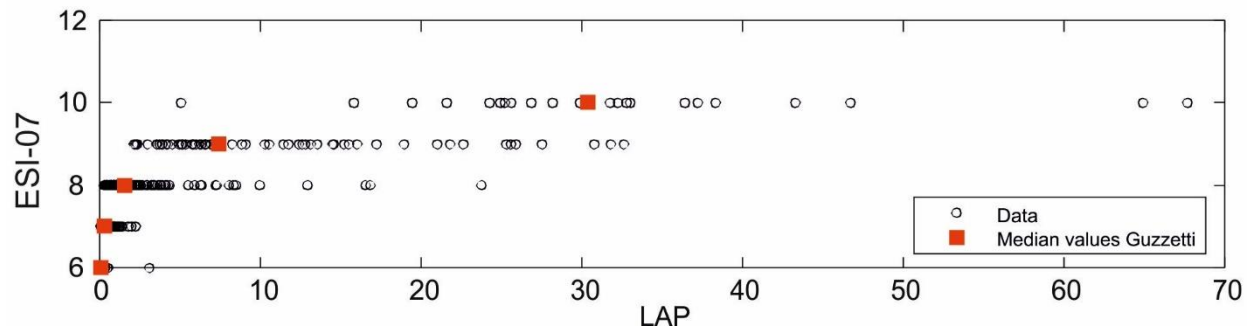
330 Figure 8: Plots of LND (a) and LAP (b) vs local ESI-07; intensity computed using the Guzzetti et al. (2009) scaling relation is shown as an example.
