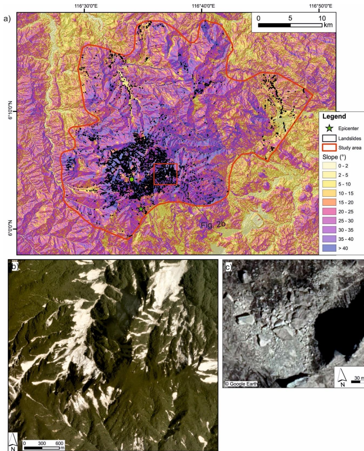
Figure 2: a) Slope map and hillshade derived from 30-m resolution ALOS DEM; the red polygon is the study area, while landslides are shown in black; b) Planet Labs image (3-m resolution) taken on 18 March 2016 showing widespread landslides; c) © Google Earth image of a rockfall on top of Mt. Kinabalu (location is the green dot in Fig 2a).
