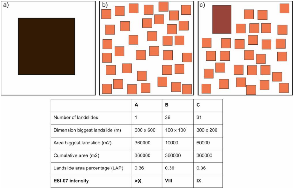
Figure 3: Sketch illustrating the role of number and dimension of landslides (coloured squares) on the computation of LND, LAP and ESI-07. The upper panels represent simplified scenarios: a) one wide landslide; b) many landslides, all of small dimension; c) many landslides with variable dimension.
