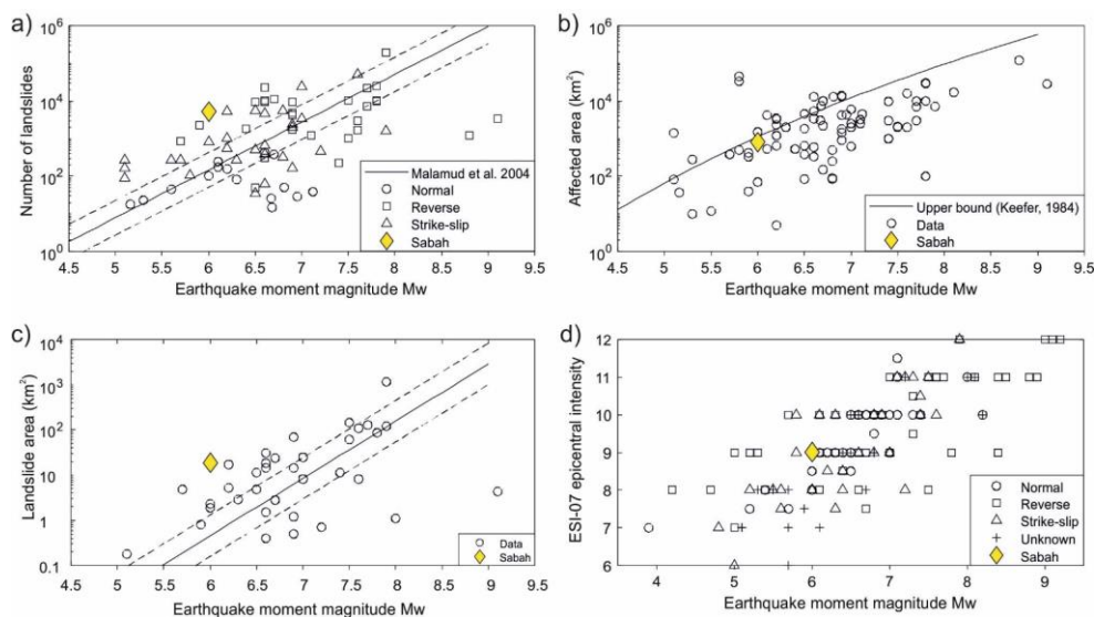
Figure 7: Comparison of the Sabah earthquake with global studies: a) number of landslides vs Mw, regression is Equation (2); b) affected area vs Mw, upper bound after Keefer, 1984; c) landslide area vs Mw, regression is Equation (3); d) ESI-07 epicentral intensity.
