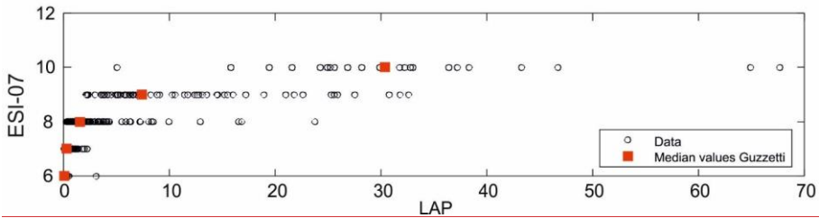
Figure 8: Plots of LND (a) and LAP (b) vs local ESI-07; intensity computed using the Guzzetti et al. (2009) scaling relation is shown as an example.
