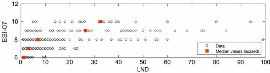
b) LAP vs ESI-07
