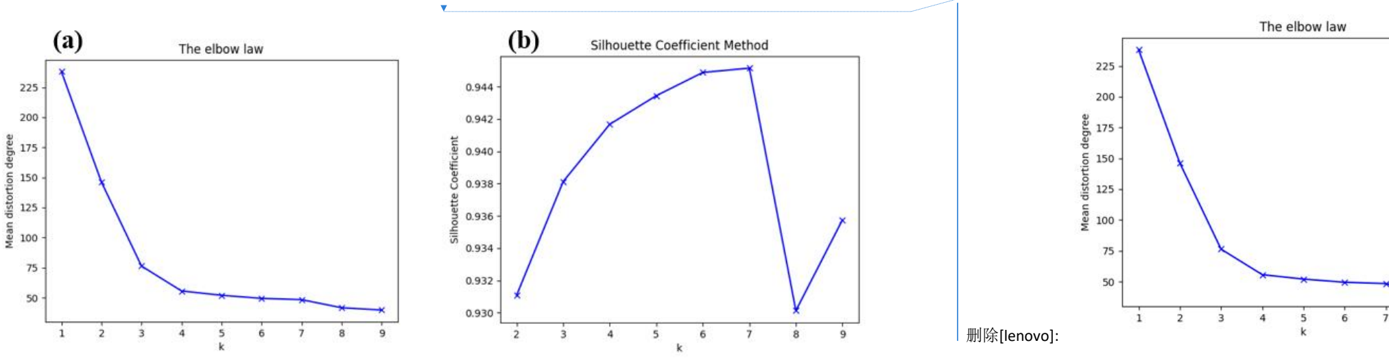
Figure 2. Evaluation for different number of categories in k-means by the elbow law and silhouette coefficient method
