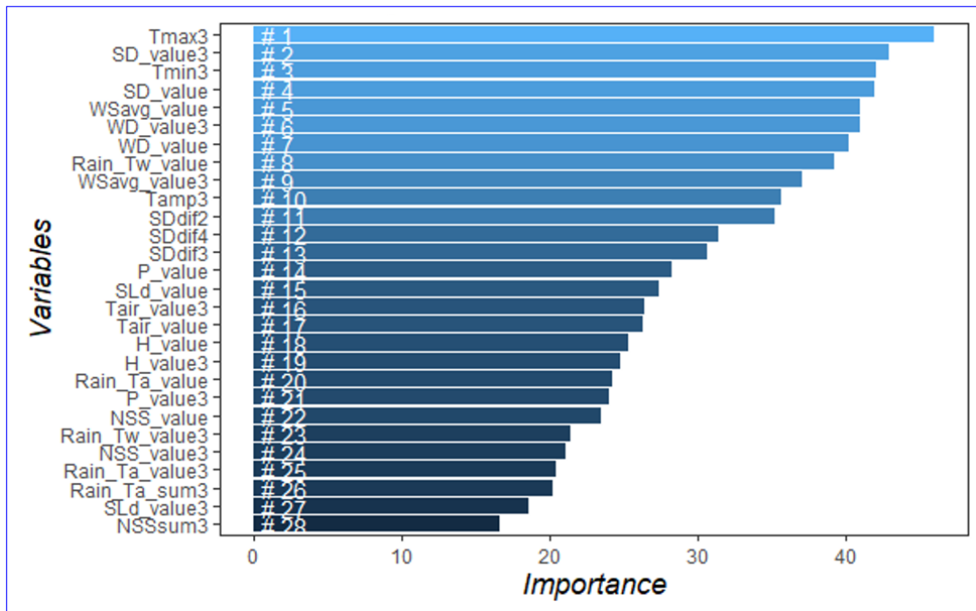
Fig. 6. Variable importance using the Mean Decrease Accuracy (MDA) for each variable of wet avalanche dataset (winter seasons 1979–2020) in the ran
