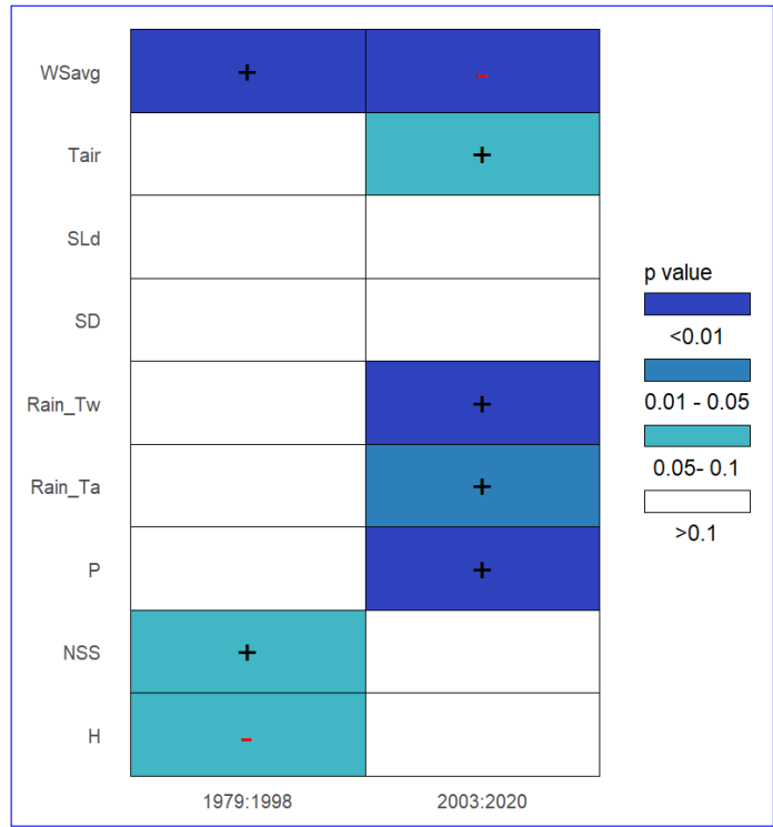
Fig. 7. Trends at LBOU meteorological station for meteorological and snow variables (mean values) in winter season (1.10-31.5). The values represent T
