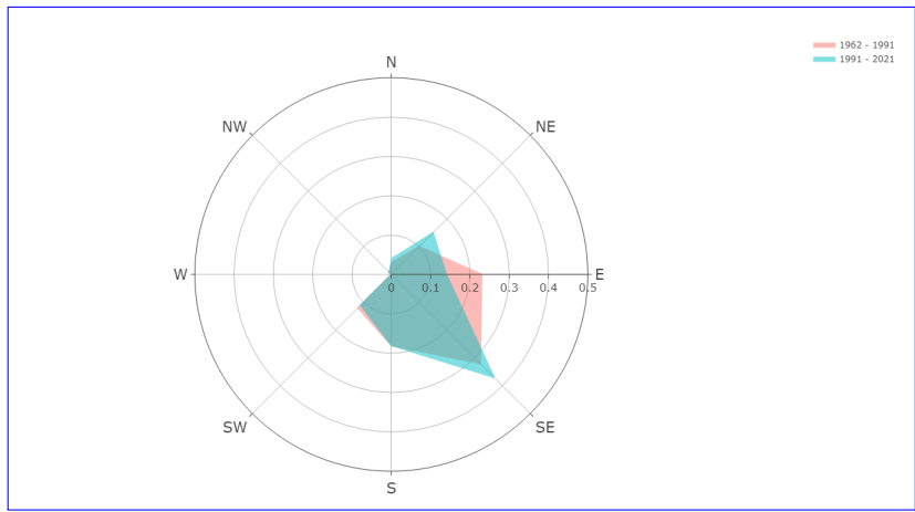
Fig. 8. The avalanche occurrence path distribution per orientation for slab avalanches. Radial axis represents the avalanche portion for each cardinal direct
