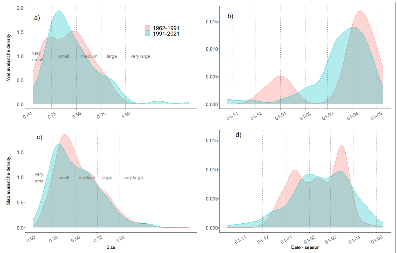
Fig. 3. Occurrence of wet avalanches over the last six decades. a) Total number Wet snow and slab avalanche size over decades. Each decade represents the snow characteristics splitted into two winter season starting the 1st of October periods 1962-1991 and ending the 31st of May 1991-2021. Four events are omitted due to missing value a) Proportional sizes of avalanche length related to the RAMMS 100 year return period output. b) Total numbers over months Winter season distribution of avalanche occurrences.
