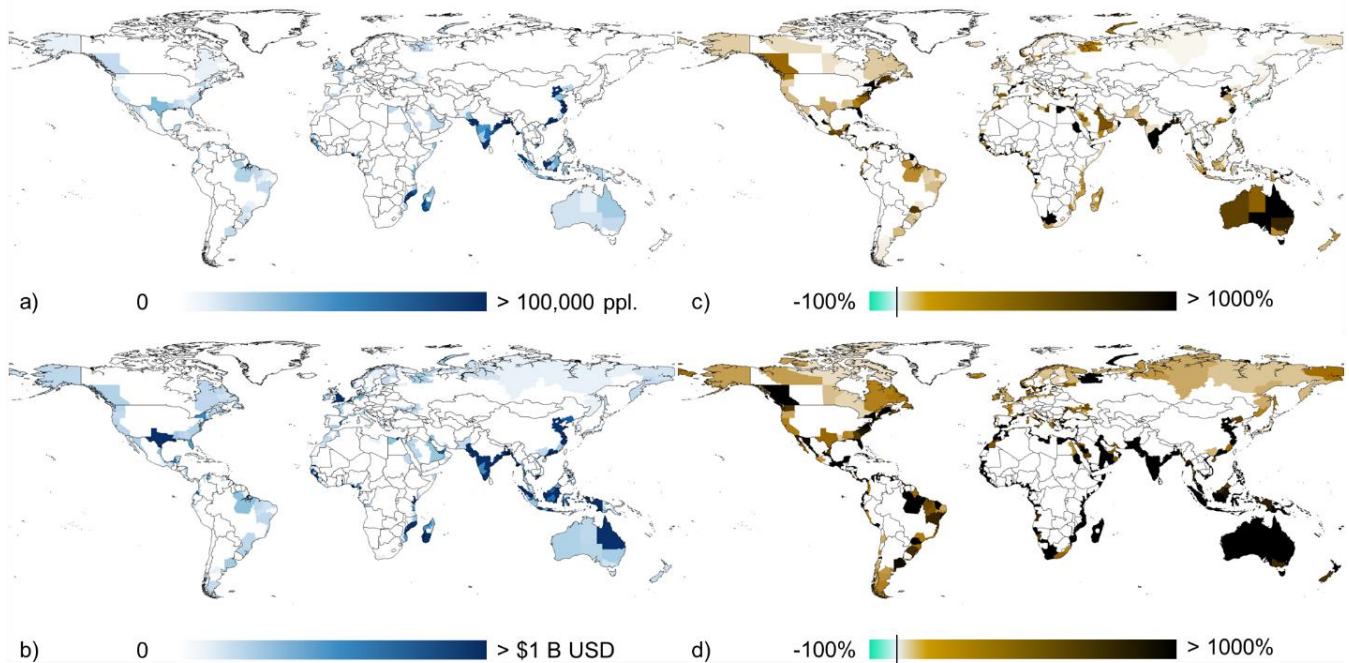
330 Figure 2: Global maps depicting simulated sub-national regional changes between 2020 and 2080 in: a) absolute EAAP, b) absolute 335 EAD, c) relative EAAP, and d) relative EAD, assuming there are no increases to current protection standards.
