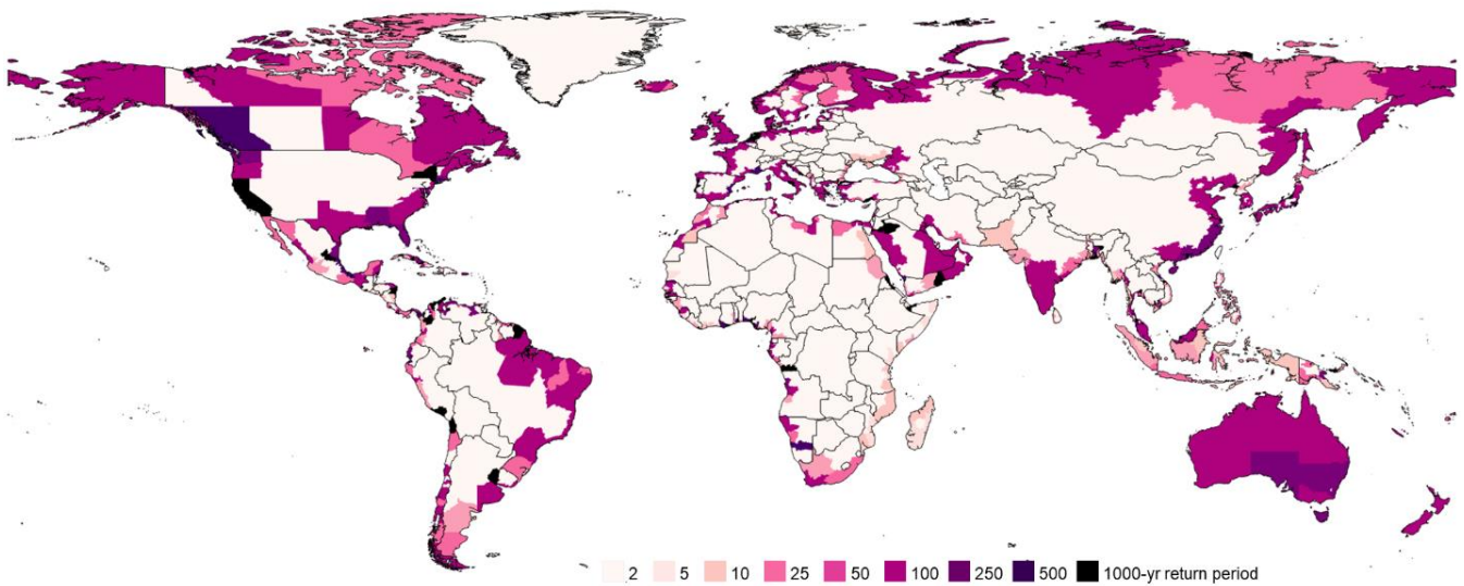
350 Figure 4: Estimated protection standards required for sub-national regions to achieve their relative-risk constant risk reduction targets in 2080.
