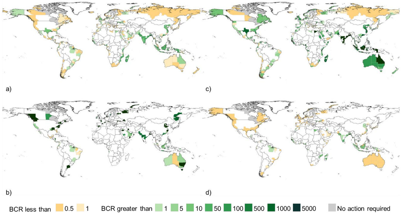
Figure 6: Benefit-cost ratio values for a) dykes and coastal levees, b) foreshore vegetation, c) zoning restrictions, and d) dry-proofing on the sub-national scale, where yellow indicates overall direct costs outweighing overall benefits and green overall benefits outweighing overall direct costs. Grey areas are sub-national regions where action is not required to achieve the relative-risk reduction targets.
