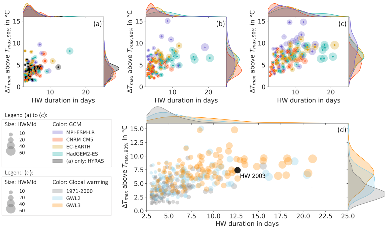
Figure 7. Bubble plot of the strongest HW in each summer half-year (May–Oct) in every projection run. The considered events are identified over the maximum of the HWMIId integrated over the area. The HW features of all involved grid points are averaged. The bubble plots show the strongest HW in each summer half-year (May–Oct) in every projection run with respect to duration on the abscissa and excess temperature on the ordinate. Bubble size indicates mean HWMIId over all grid point results affected by the HW. Marginal plots show the distribution of duration of the heat waves in days (abscissa) and the distribution of the excess temperature (ordinate). Panel a to c show the single ensemble members and comparison with the observation: a for 1971–2000, b for GWL2, and c for GWL3. In Panel d the ensemble members of one GWL are merged to display the evolution over time. Panel d shows the total set of all of the heat waves from the single ensemble members for 1971–2000, GWL2 and GWL3. The black data point corresponds to the HW in 2003 derived from HYRAS data.
