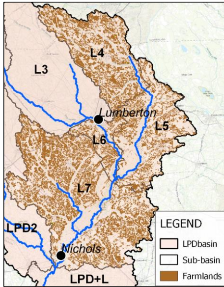
340 Figure 6. Feasible sites for afforestation in croplands (original LULC layer extracted from MRLC consortium).
