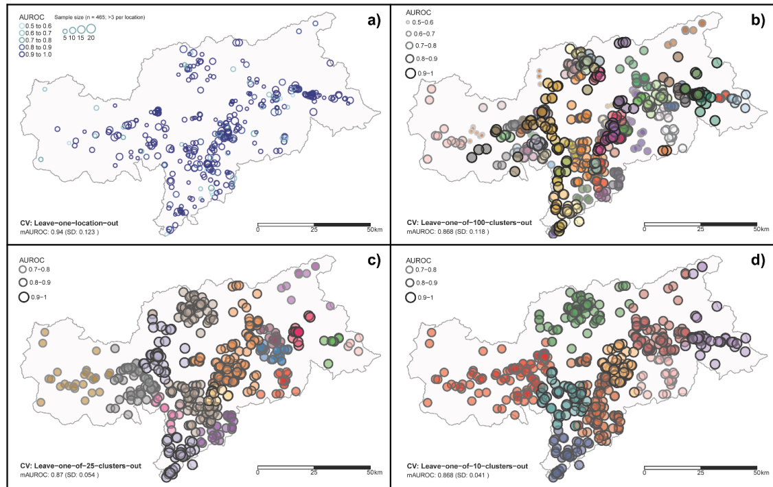
565 Figure 11 Leave-one-spatial-unit-out CV. The maps depict, for different test subregions, the predictive performance of models that were trained on the remaining subregions. Leave-one-location-out CV (a) was performed for 465 locations associated with more than three observations per location. In a) The AUROCs are shown from light blue (0.5 – 0.6) to dark blue (0.9 – 1) and the circle size is proportional to the test sample size. The maps (b) to (d) are based on k-means clustering and depict different k-values (i.e., 100 clusters in b, 25 in c, 10 in d). Each colour is associated to a cluster while larger circles and darker circle borders are associated to higher AUROCs and vice versa. The AUROC at the bottom refers to the mean of all locations/clusters (mAUROC).
