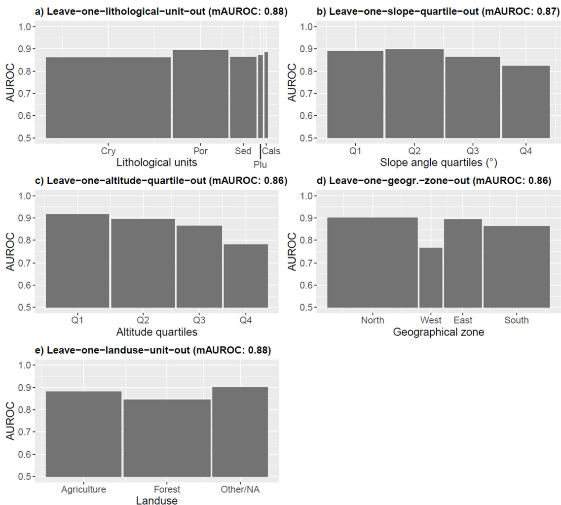
Figure 12 Leave-one-factor-out CV. The AUROCs reveal, for each environmental test unit, the predictive performance of a model that was trained on the remaining environmental units (e.g., data associated to the slope quartiles Q1 to Q3 was used to train a model whose prediction was tested with slope quartile Q4 data). Bar-heights depict the test AUROCs for different lithological units (a), slope quartiles (b), altitude quartiles (c), geographical zones (d) and land use units (e). Lithological units: Crystalline basement (Cry), Porphyry (Por), Sedimentary rocks (Sed), Plutonite (Plu) and Calcschists with ophiolites (Cals). The bar-width is proportional to
