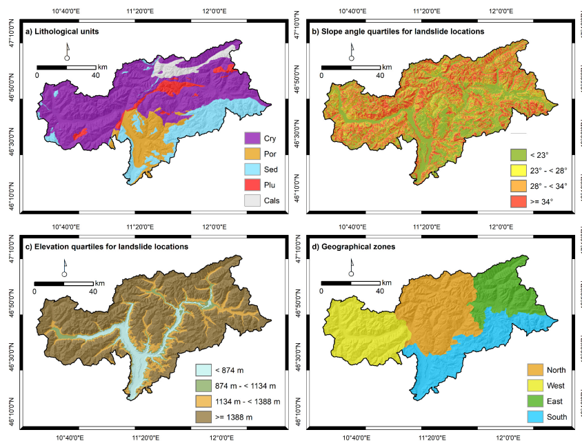
Figure 2 Spatial environmental maps used for leave-one-factor-out CV. The lithological map (a) shows the classes Crystalline basement (Cry), Porphyry (Por), Sedimentary rocks (Sed), Plutonite (Plu) and Calcschists with ophiolites (Cals). The quartile classification for slope angle (b) and elevation (c) is based on the final landslide presence sample (i.e., each class contains 25% of landslides). The geographical zonation (d) is based on the intersection of catchments.
