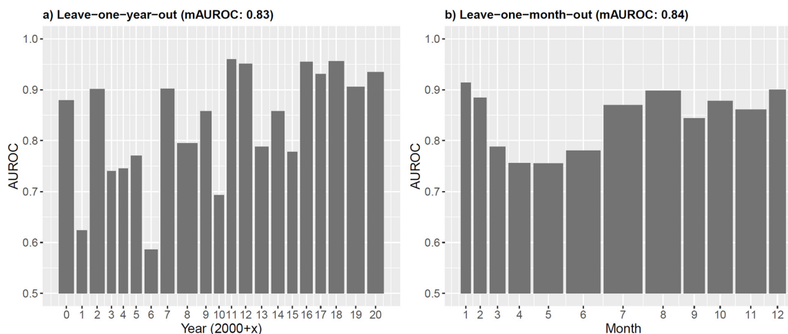
550 Figure 10 Leave-one-temporal-unit-out CV. The AUROCs reveal, for each test year (a) or test month (b), the predictive performance of a model that was trained on the remaining time periods (e.g., the months 1 to 11 were used to train a model whose prediction was tested with month 12 data). The bar-width is proportional to the underlying test sample size (presences plus absences). The mAUROC at the top refers to the mean AUROC of all time periods.
