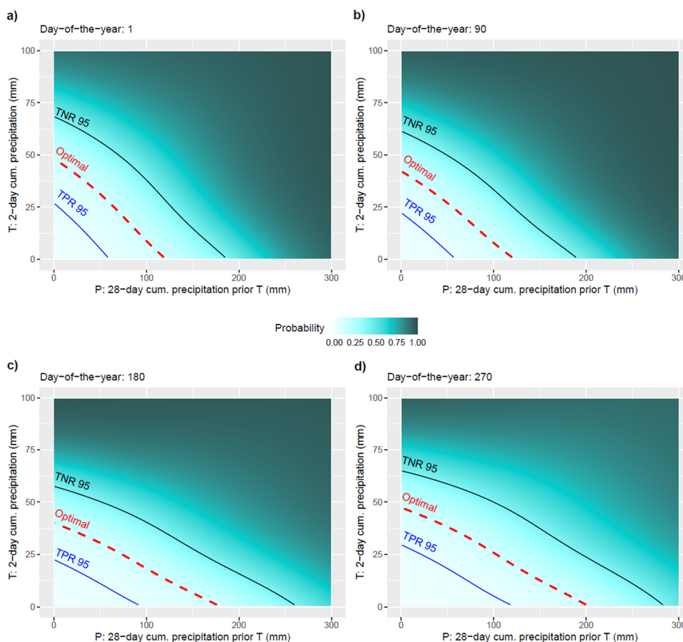
525 Figure 9 T - P plot showing the predicted probability for increasing precipitation amounts ( T , P ) and associated thresholds for a selected DOY : Day 1 (a), Day 90 (b), Day 180 (c) and Day 270 (d). The animation in the supplementary material (Animation.gif) visualizes the continuous changes from day 1 to 365.
