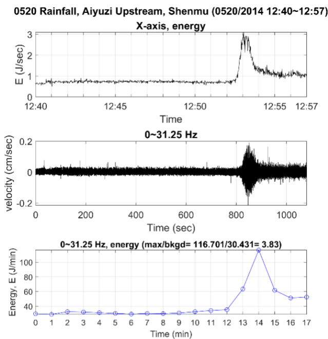
Figure 12: Energy of vibrational signals (a) 0504 Rainfall in 2012 (b) 0520 Rainfall in 2014 (Huang et al., 2019).
