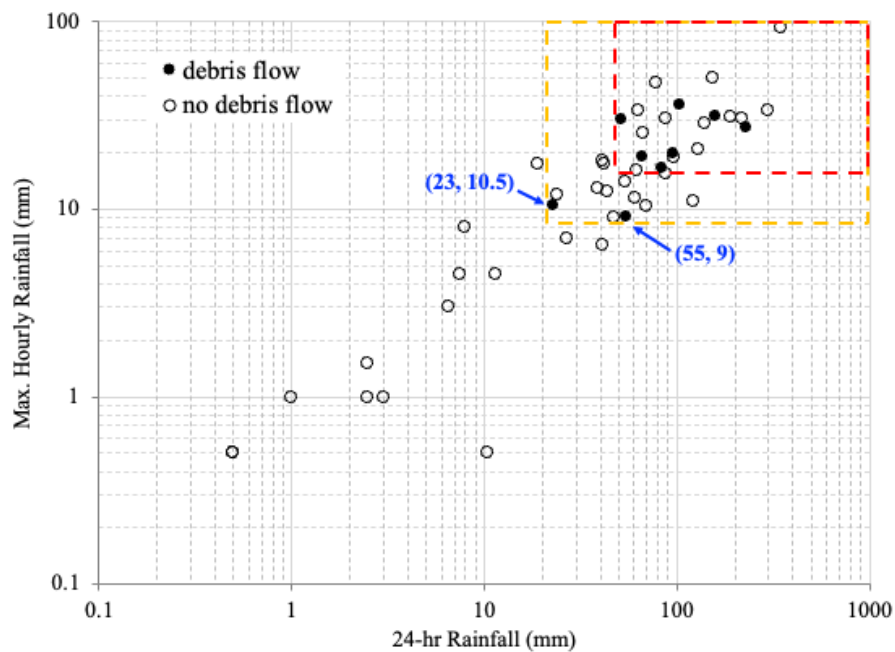
Figure 7: The max. hourly rainfall and 24-hr rainfall of events in the Shenmu area.
