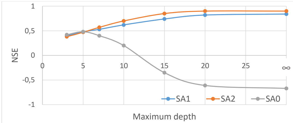
Figure S1. Shows the impact of varying the maximum depth of the decision trees on the RF – SA1 & 2 model performance using holdout validation method. The X-axis shows the implemented maximum depth of the decision trees while the Y-axis denotes the computed Nash Sutcliffe Efficiency (NSE)
