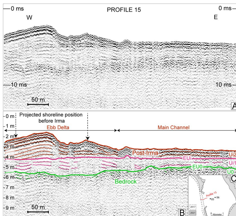
1065 Figure 5. (A) Seismic profile 15 (length approximately 570 m) showing a part of the lagoon central inlet structure (east–west transect) in June 2021. (B) Interpreted profile. (C) Profile localization in comparison with the sandy barrier in 2021 (in gray) and in 2017 before Hurricane Irma (in dotted lines).
