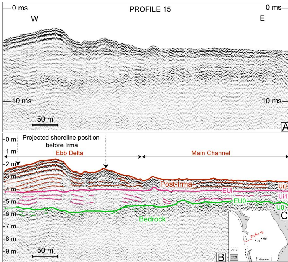
1070 Figure 5. (A) Seismic profile 15 (length approximately 570 m) showing a part of the lagoon central inlet structure (east–west transect) in June 2021. (B) Interpreted profile. (C) Profile localization in comparison with the sandy barrier in 2021 (in gray) and in 2017 before Hurricane Irma (in dotted lines).
