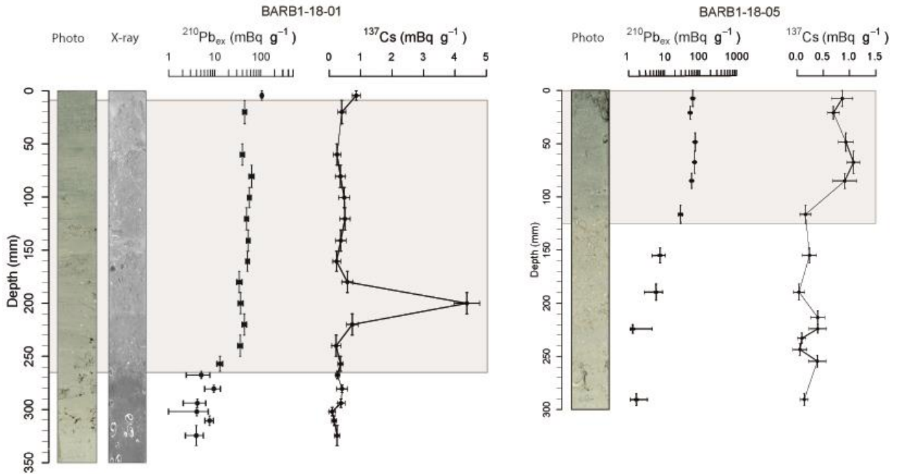
Figure 11. BARB1-18-01 and BARB1-18-05 short-lived radionuclide data with 210 Pb ex on a logarithmic scale associated with the 137 Cs activity profiles, core pictures and X-ray. The gray rectangles display the F1 layer boundaries.
