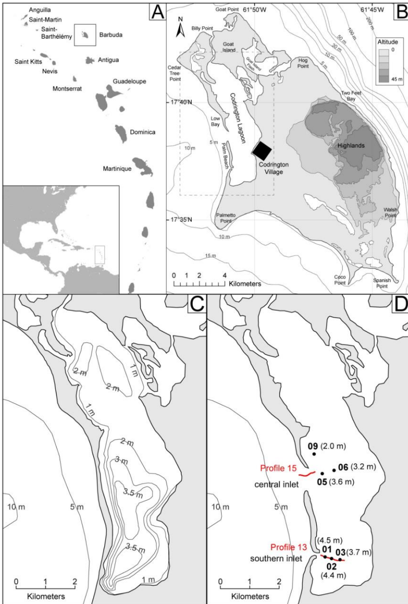
1030 Figure 1. (A) The Caribbean Sea and Lesser Antilles Arc ( https://freevectormaps.com/world-maps/caribbean/WRLD-CI-01-0001?ref=atr ). (B) Topography of Barbuda Island in 2018 (after Irma), modified from Bain et al., 2018 and Brasier 1975a, 1975b. (C) Codrington Lagoon morpho-bathymetry, from Brasier 1975a, 1975b. (D) Codrington Lagoon morphology 3 months after
