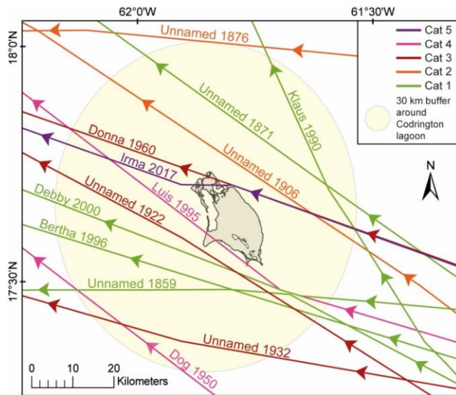
Figure 2. Historical hurricane tracks (1859–2017) passing within 30 km from Codrington Lagoon (Barbuda) (NOAA, 2021, Historical Hurricane Tracks).
