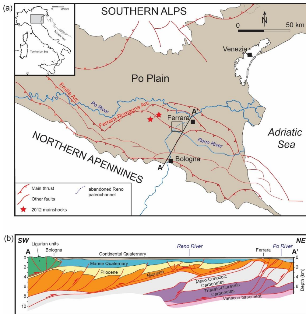
495 Figure 1: a) Tectonic sketch map of the Po Plain (Northern Italy) showing the main buried faults of the Northern Apennines and Southern Alps and epicenters of the two mainshock from the 2012 Emilia sequence (red stars) (modified from Tentori et al., 2022 and Bruno et al., 2021). The black-lined rectangle encloses the study area. b) Simplified stratigraphic cross section and major tectonic structures along the trace A–A' in figure a) (modified after Boccaletti et al., 2004). The tectonic structures are enucleated into Mesozoic to Paleogene carbonate successions, and largely controlled the sedimentary evolution of the terrigenous basins during the Neogene (Ghielmi et al., 2013; Rossi et al., 2015; Ricci Lucchi, 1986). The Pliocene-Pleistocene boundary records the transition from turbiditic sedimentation to marine clay deposition whereas the Quaternary sedimentary fill consists of marine deposits, nearshore sands and alluvial deposits (see text for details). 500
