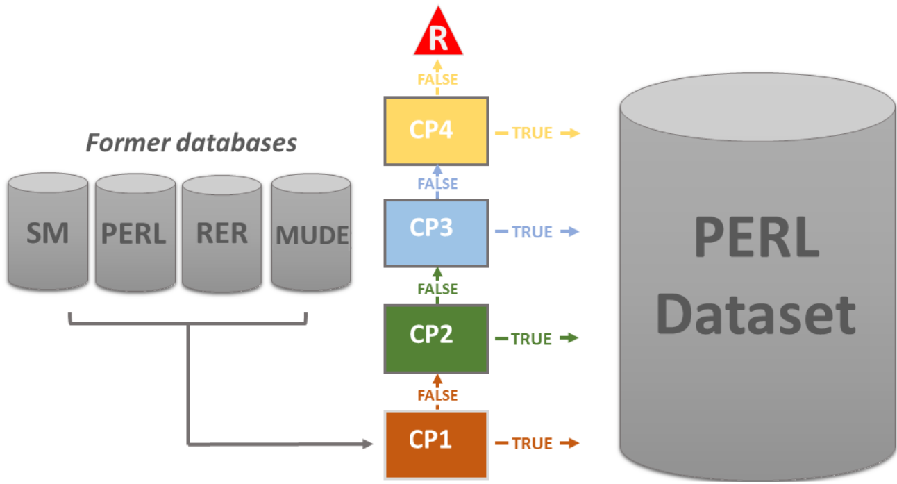
510 Figure 2: Synthetic workflow of the method used to merge MUDE, RER, SM database and new realization investigations into the PERL dataset.
